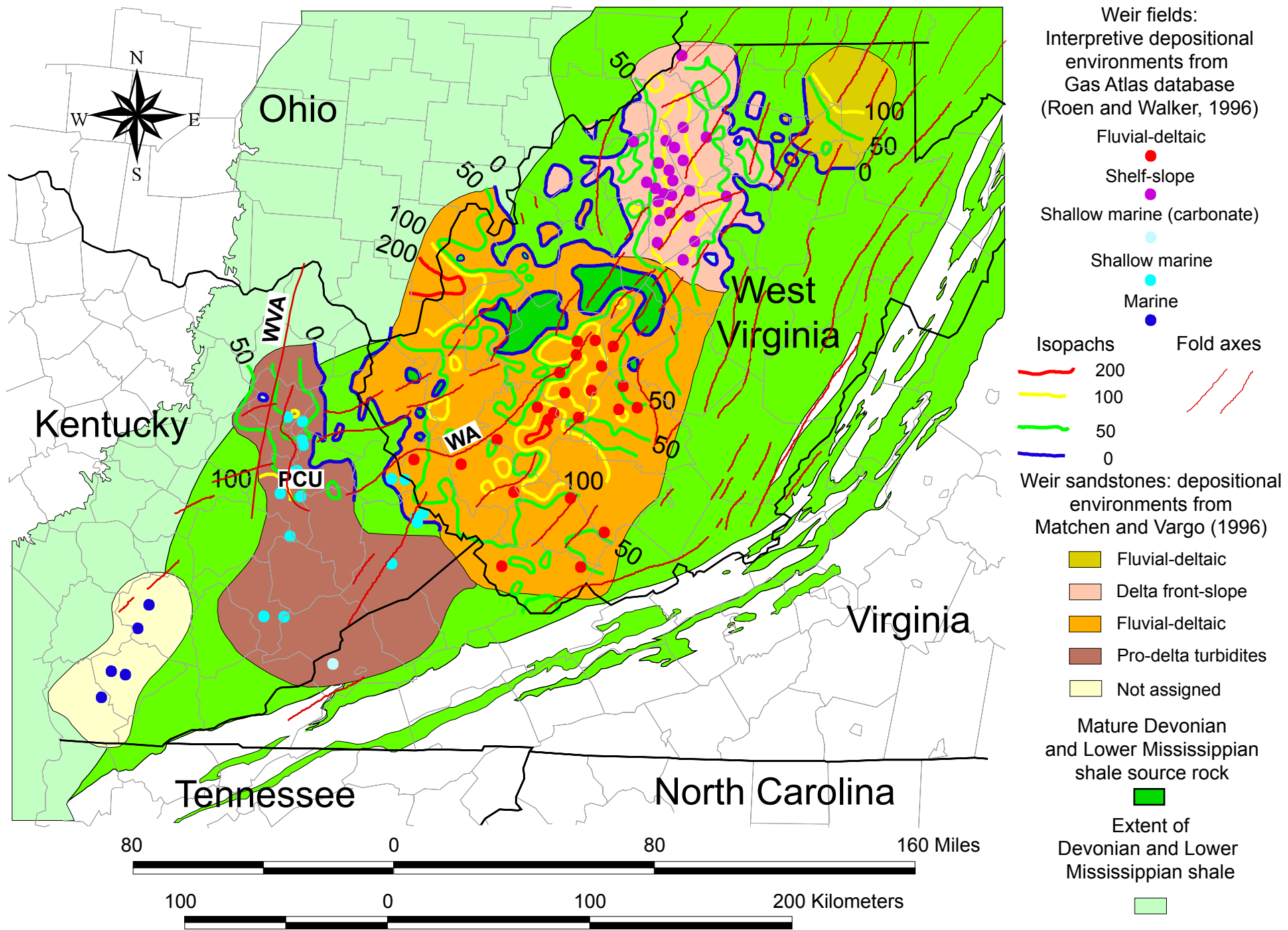
Figure 54. Weir sandstones in the Appalachian basin, showing interpreted depositional environments, generalized thickness, and field locations. WA is Warfield anticline; PCU is Paint Creek Uplift; WVA is Waverly arch. (modified slightly from Matchen and Vargo, 1996).
