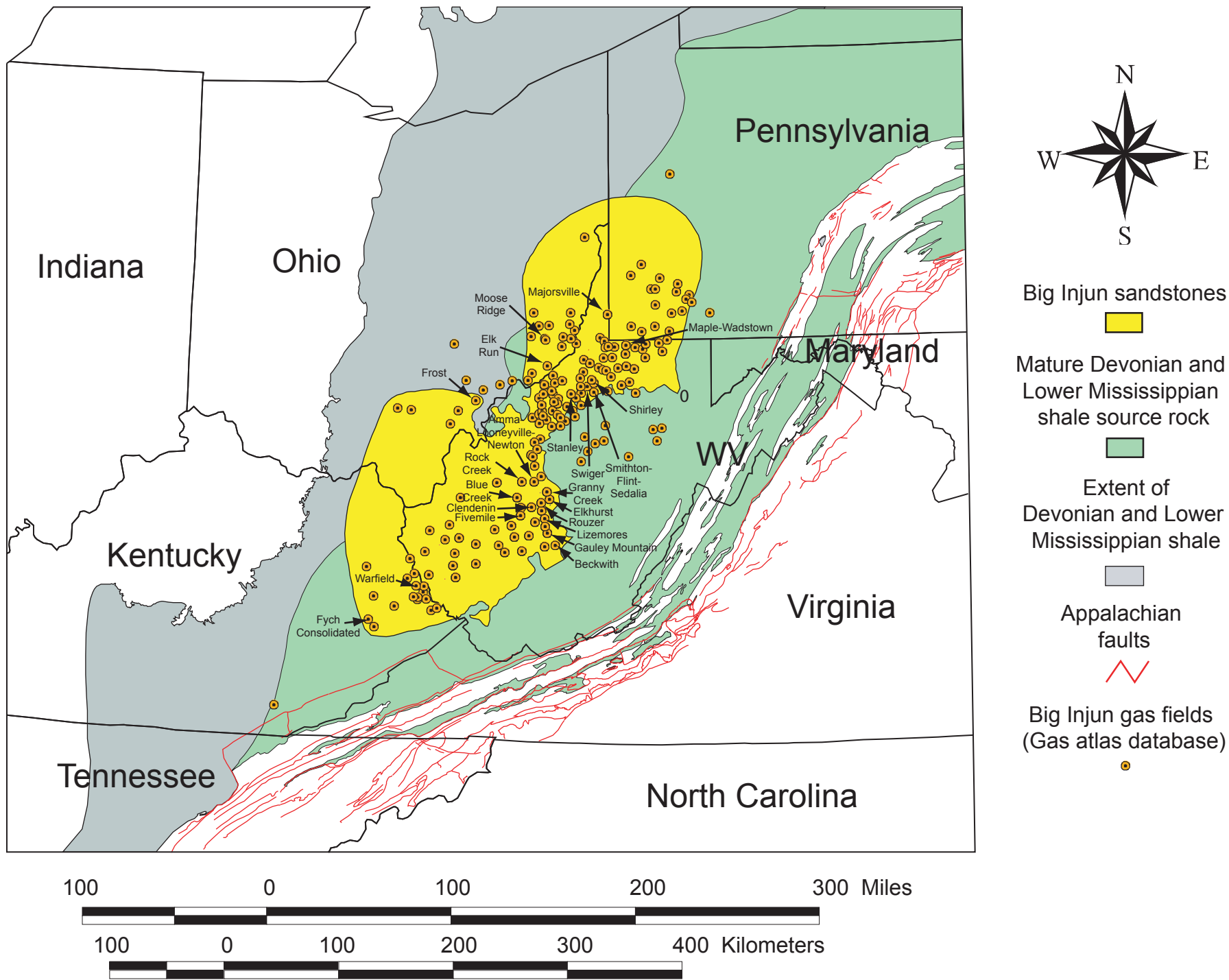
Figure 57. Selected Big Injun sandstone field names (includes those described in the database of Roen and Walker, 1996; modified slightly from Vargo and Matchen, 1996) WV is West Virginia.
