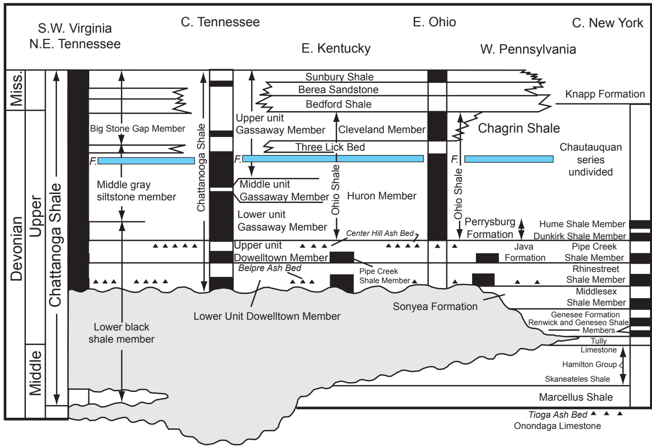
Figure 6. Correlation of Devonian and Mississippian black gas shales and some related rocks in the Appalachian basin (slightly modified from deWitt and others (1993). F. Foerstia zone; ▲, ash bed.
