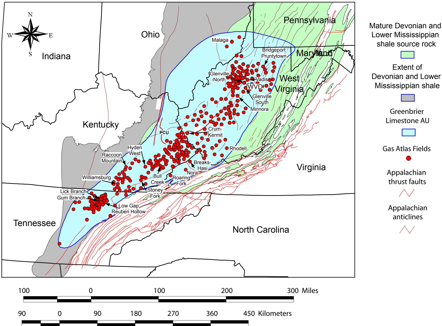
Figure 60. The Greenbrier Limestone Assessment Unit, showing the locations of gas fields (from database of Roen and Walker, 1996; Smosna, 1996). WVD is West Virginia dome; WA is Warfield anticline; WVA is Waverly arch; PCU is Paint Creek uplift.
