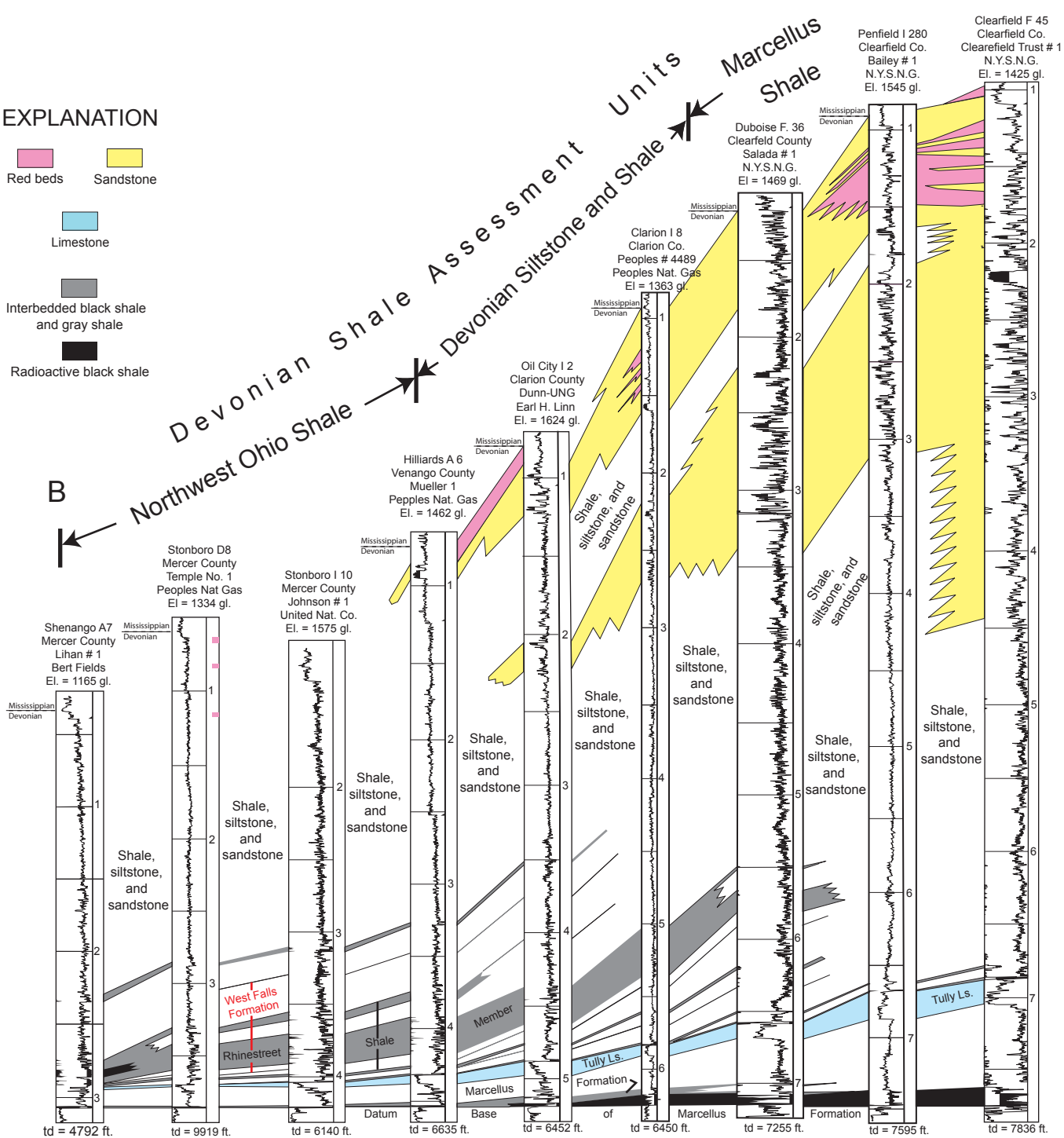
Figure 8b. Gamma ray cross section BB' of Middle and Upper Devonian strata from Clearfield to Mercer Counties, western Pennsylvania, showing relationship of shale source rocks to sandstone reservoirs (adapted from Piotrowski and Krajewski, 1977). Vertical scale in thousands of feet (See figure 8a for location of section).
