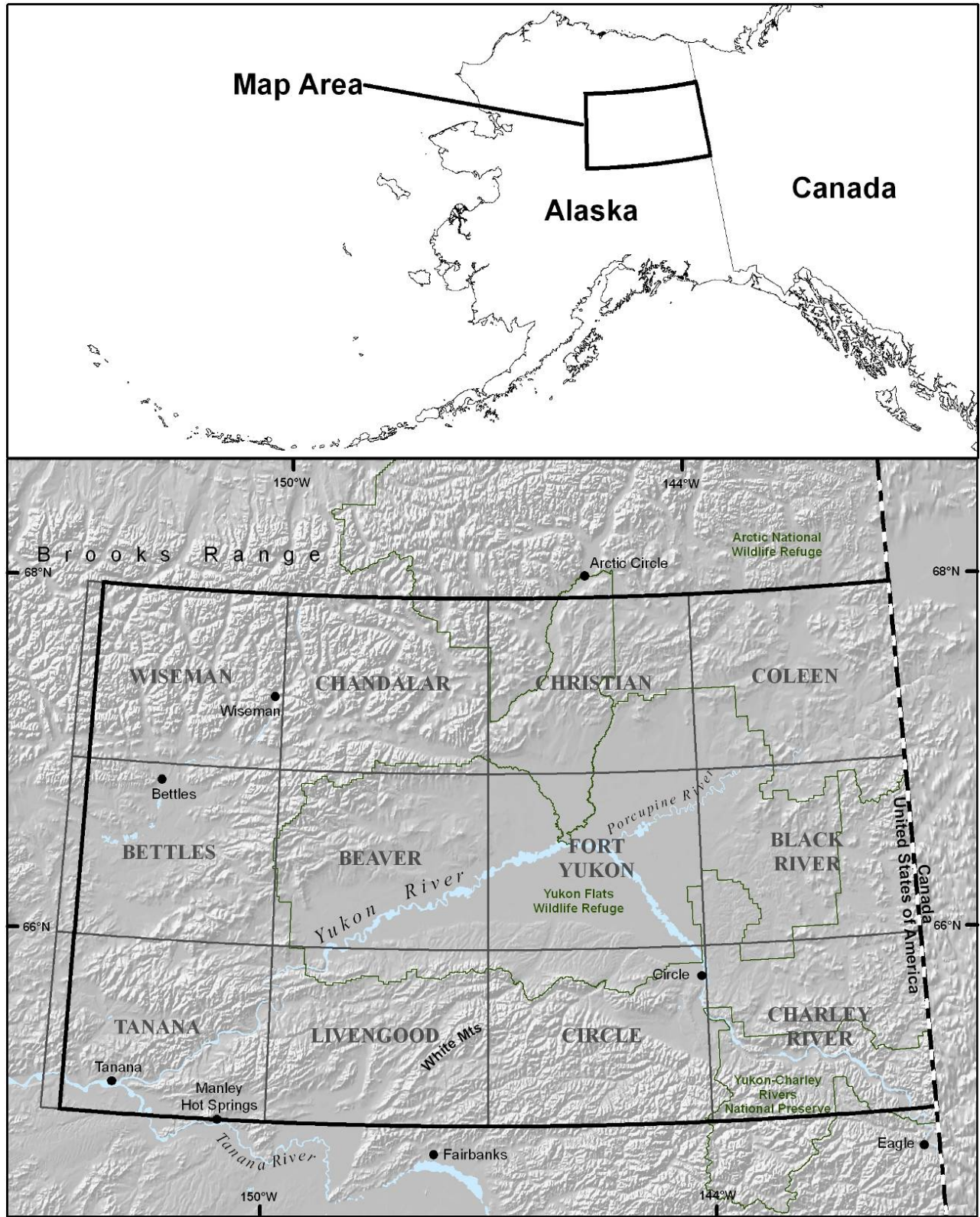
Figure 1. Location of the reconnaissance geologic map of the Yukon Flats showing the geographic setting and associated 1:250,000 quadrangles.
