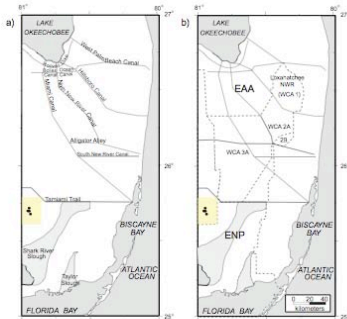
Figure 3. Map of water control structures in place in greater Everglades ecosystem. a) ~1930 AD b) ~1970 AD (post C&SF Project) (from Willard and others, 2006). Study area is highlighted in yellow. Core sites are indicated by black dots.
