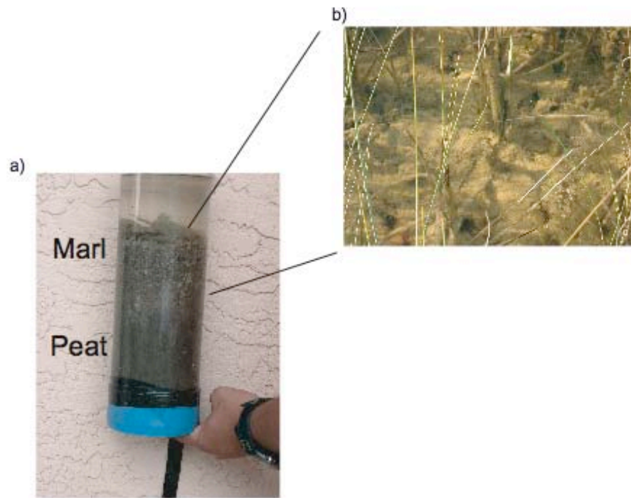
Figure 2. a) Sediment core collected from solution hole in marl prairie habitat. Note marl layer at top of core. b) Photograph of periphyton and marl sediment that makes up surface sediments in Everglades marl prairies.
