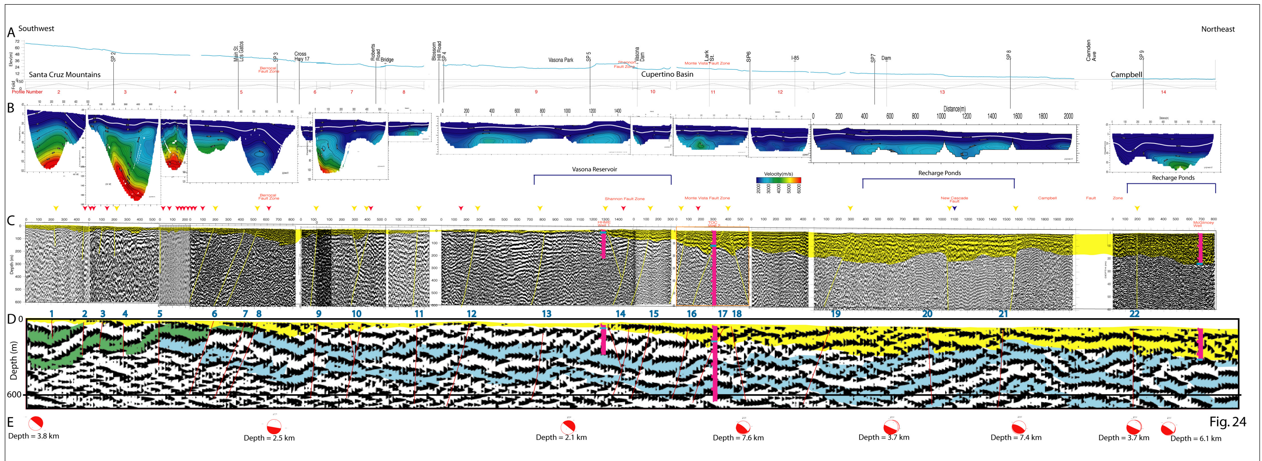
Figure 24. Comparative figures of (a) topographic profile along the SCSI-HR seismic profile, (b) composite P-wave velocity images from figure 20, (c) composite interpretative unmigrated reflection images from figure 21b, (d) interpretative SCSI-LR migrated reflection image from figure 23b, and (e) focal mechanisms in plan view for shallow-depth earthquakes along the profile. The numbers above figure 24d indicate imaged faults on both the SCSI-HR and SCSI-LR seismic profiles.
