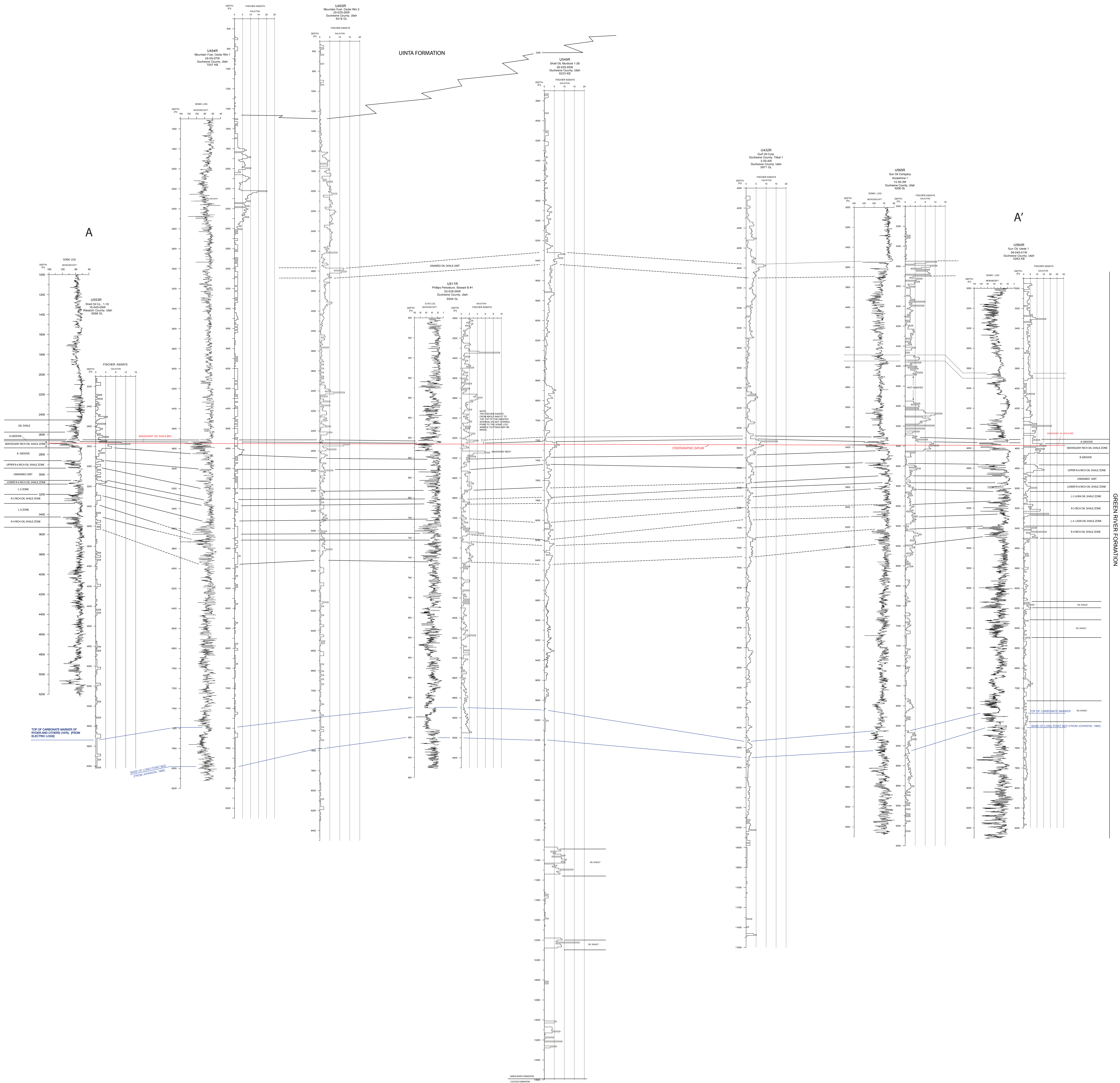
PLATE 1.—CROSS SECTION A-A' IN THE WESTERN PART OF THE UINTEA BASIN, UTAH
