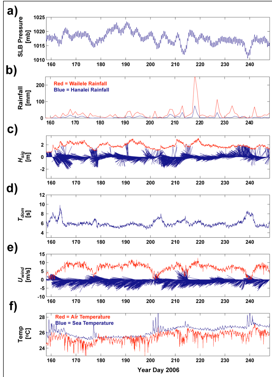
Figure 4. Deep-water oceanographic and meteorologic forcing during the study period from the NDBC (2006) buoy. a) Sea-level barometric pressure. b) Rainfall. c) Significant wave height. d) Dominant wave period. e) Wind speed (red) and velocity and direction (blue). f) Air (red) and sea surface (blue) temperature. The waves were predominantly due to the northeast trade winds throughout most of the experiment except for two periods of larger-than-normal waves in early June (YD 161-165) and late July (YD 202-205).
