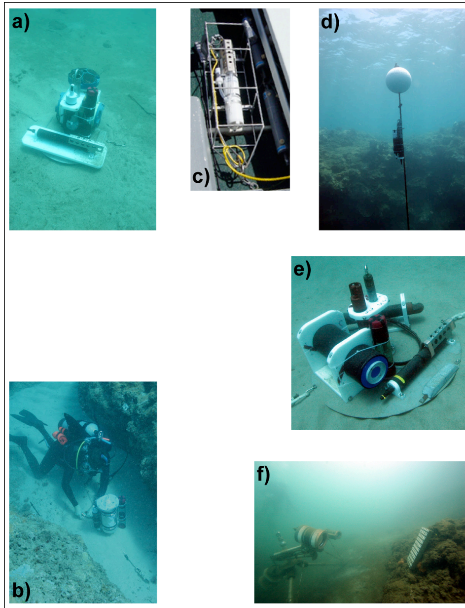
Figure 3. Photographs of the equipment used in the study. a) ADCP, SLOBS, and CT along the 10m isobath at the CRAMP Site. b) Dobie and SLOBS at the Northwest Reef Site. c) CTD/OBS/PAR profiler. d) Microcat and SLOBS 3m below the surface at the Outer Wall Site. e) ADP, SLOBS, and CT along the 10m isobath at the South-central Reef Site. f) CIS along the 10m isobath at the Outer Wall Site. See text for definition of acronyms. All of the instrument packages and moorings were deployed in patches of sand.
