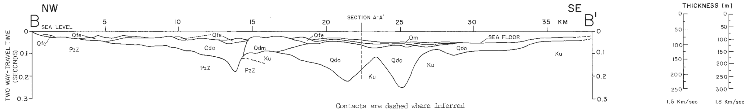
FIGURE 11 INTERPRETIVE GEOLOGIC SECTIONS A-A' AND B-B' FROM FIGURE 10
