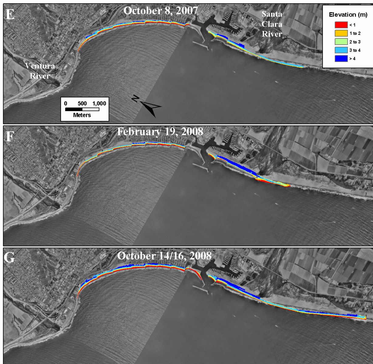
Figure B10 (cont.). Topographic data gridded to 2 m cells from the Ventura study site.
