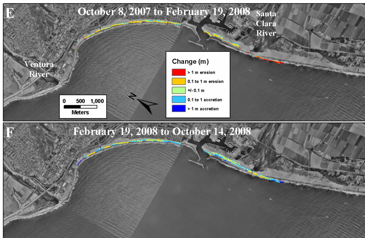
Figure B12 (cont.). Vertical change from seasonal surveys in Ventura.
