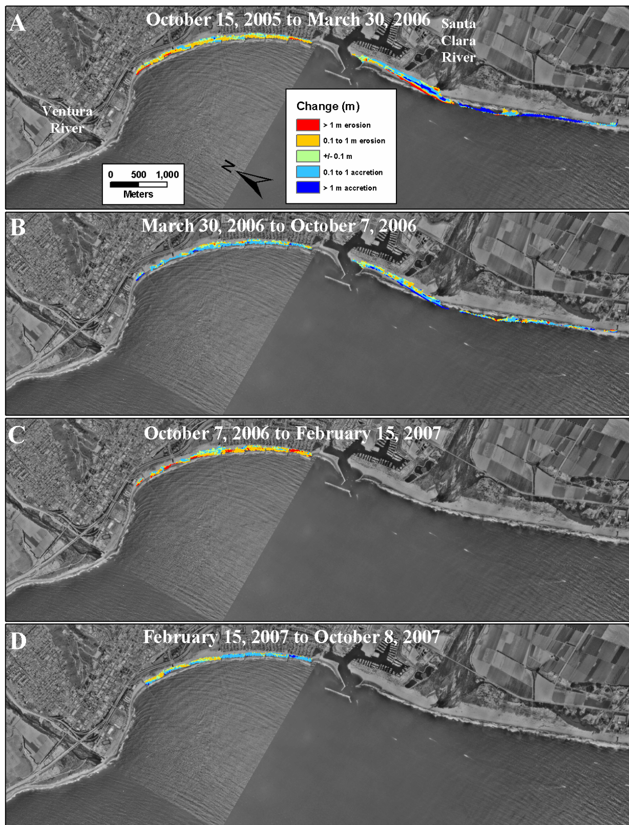
Figure B12. Vertical change from seasonal surveys in Ventura.
