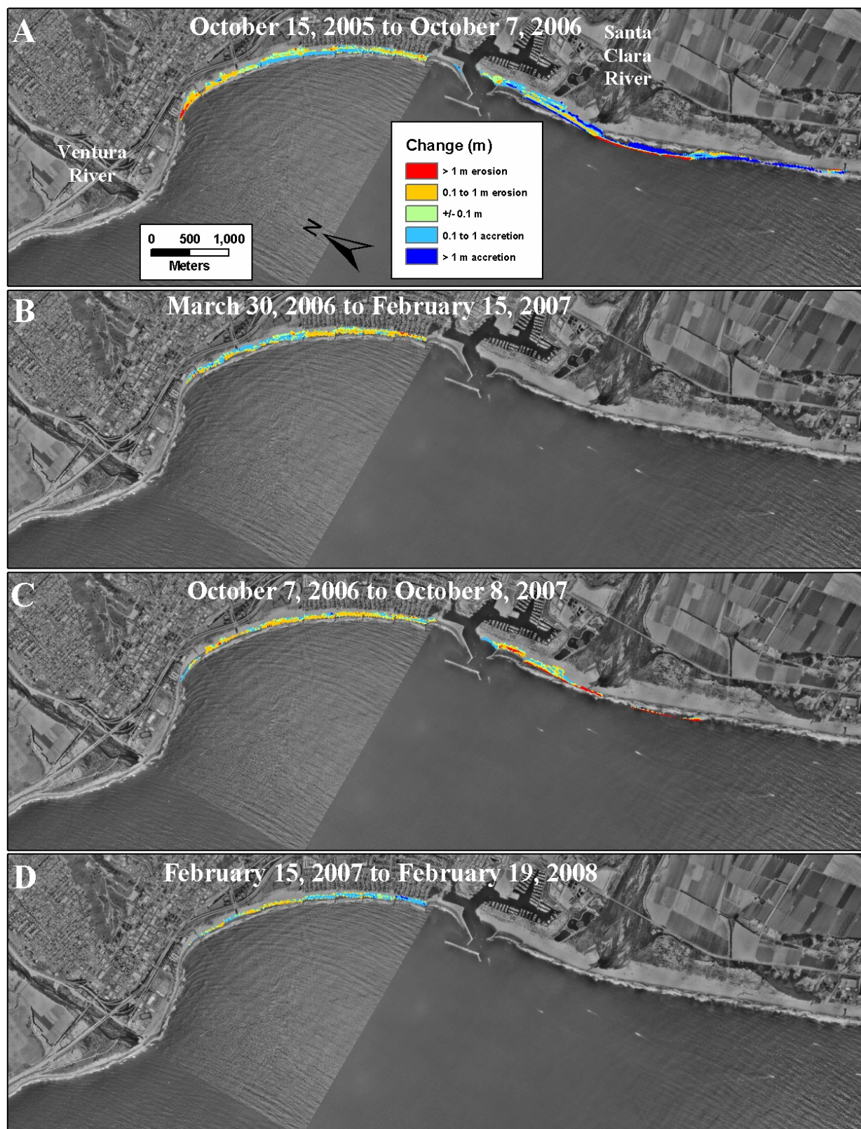
Figure B11. Vertical change from the annual surveys in Ventura.
