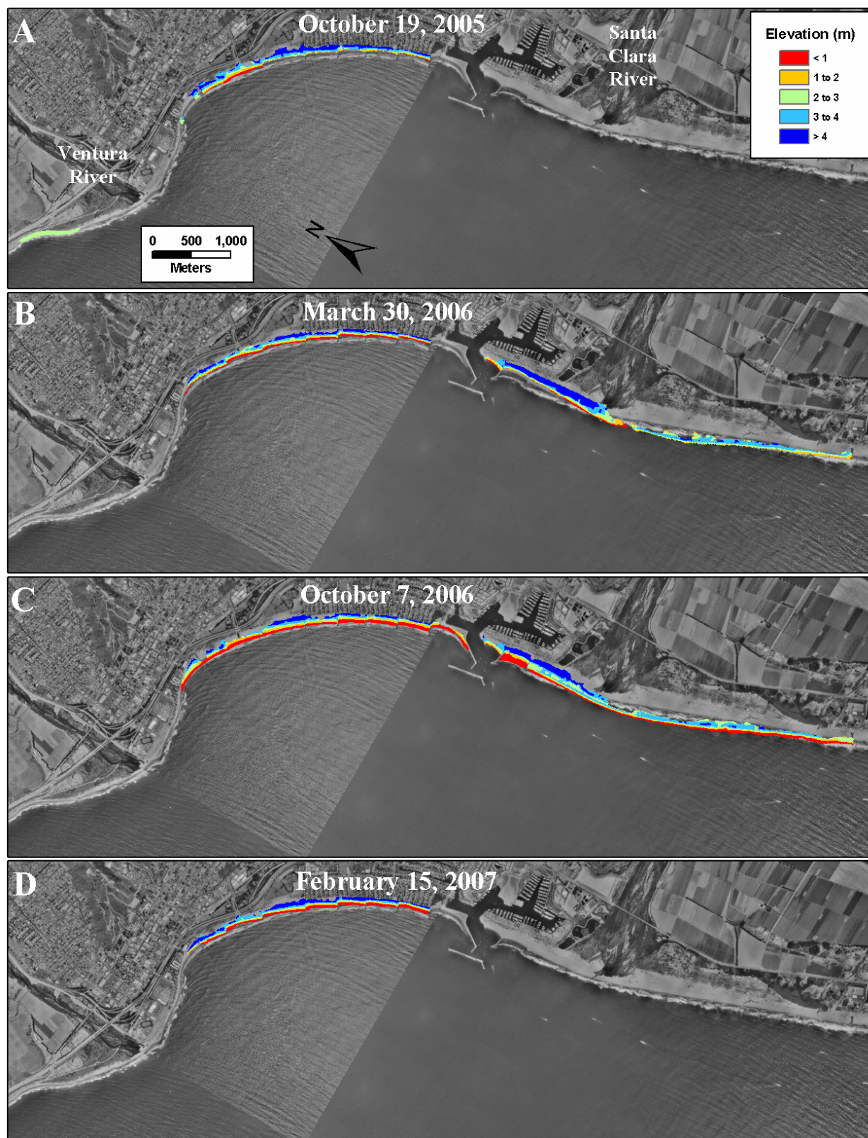
Figure B10. Topographic data gridded to 2 m cells from the Ventura study site.
