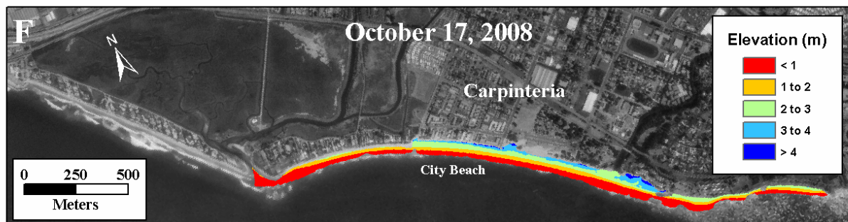
Figure B6 (cont.). Topographic data gridded to 2 m cells from the Carpinteria study site.
