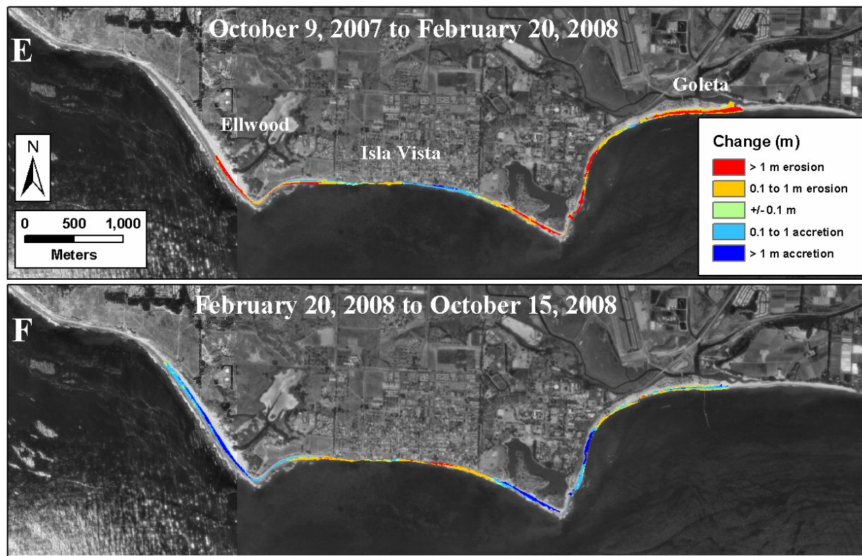
Figure B4 (cont.). Vertical change from seasonal surveys in Ellwood/Isla Vista/Goleta.
