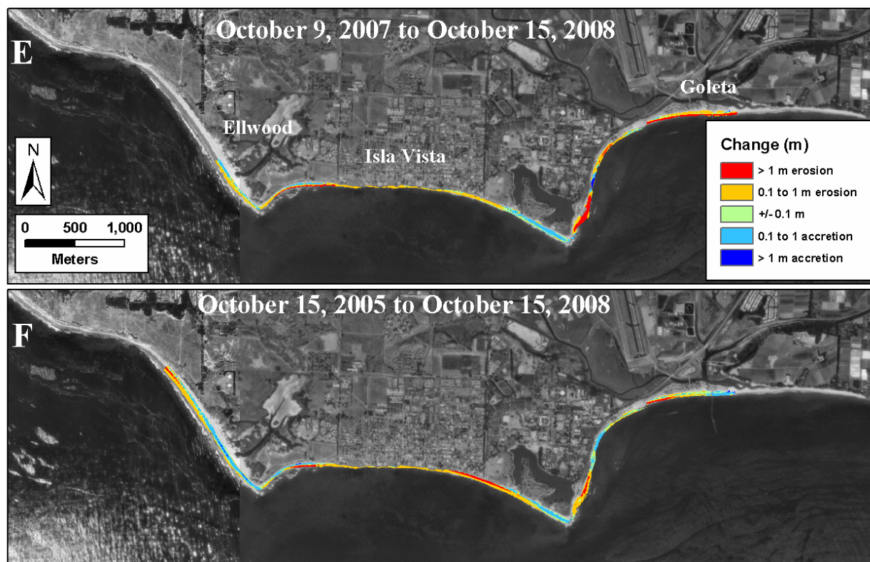
Figure B3 (cont.). Vertical change from the annual surveys in Ellwood/Isla Vista/Goleta.
