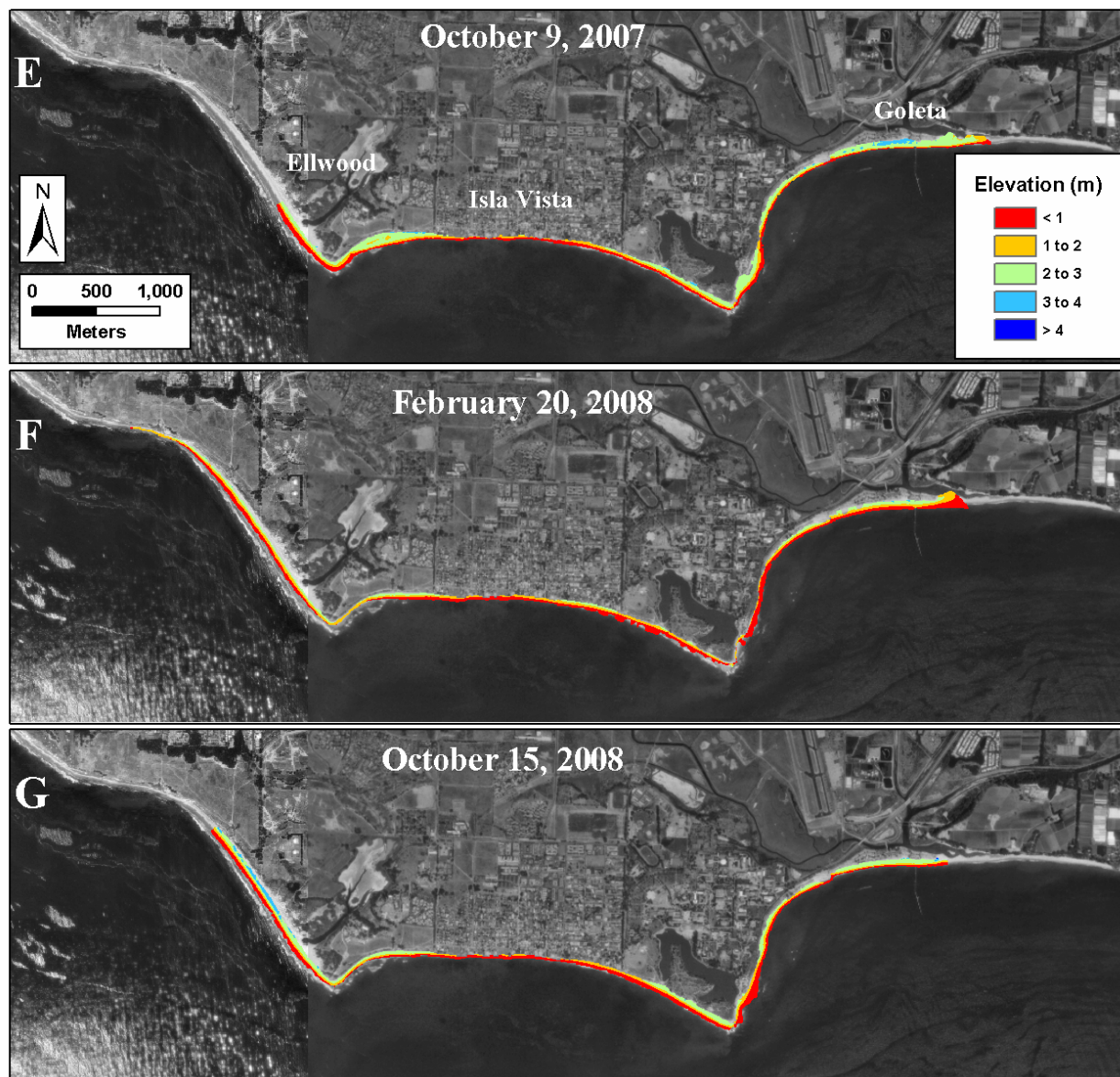
Figure B2 (cont.). Topographic data gridded to 2 m cells from the Ellwood/Isla Vista/Goleta study site.
