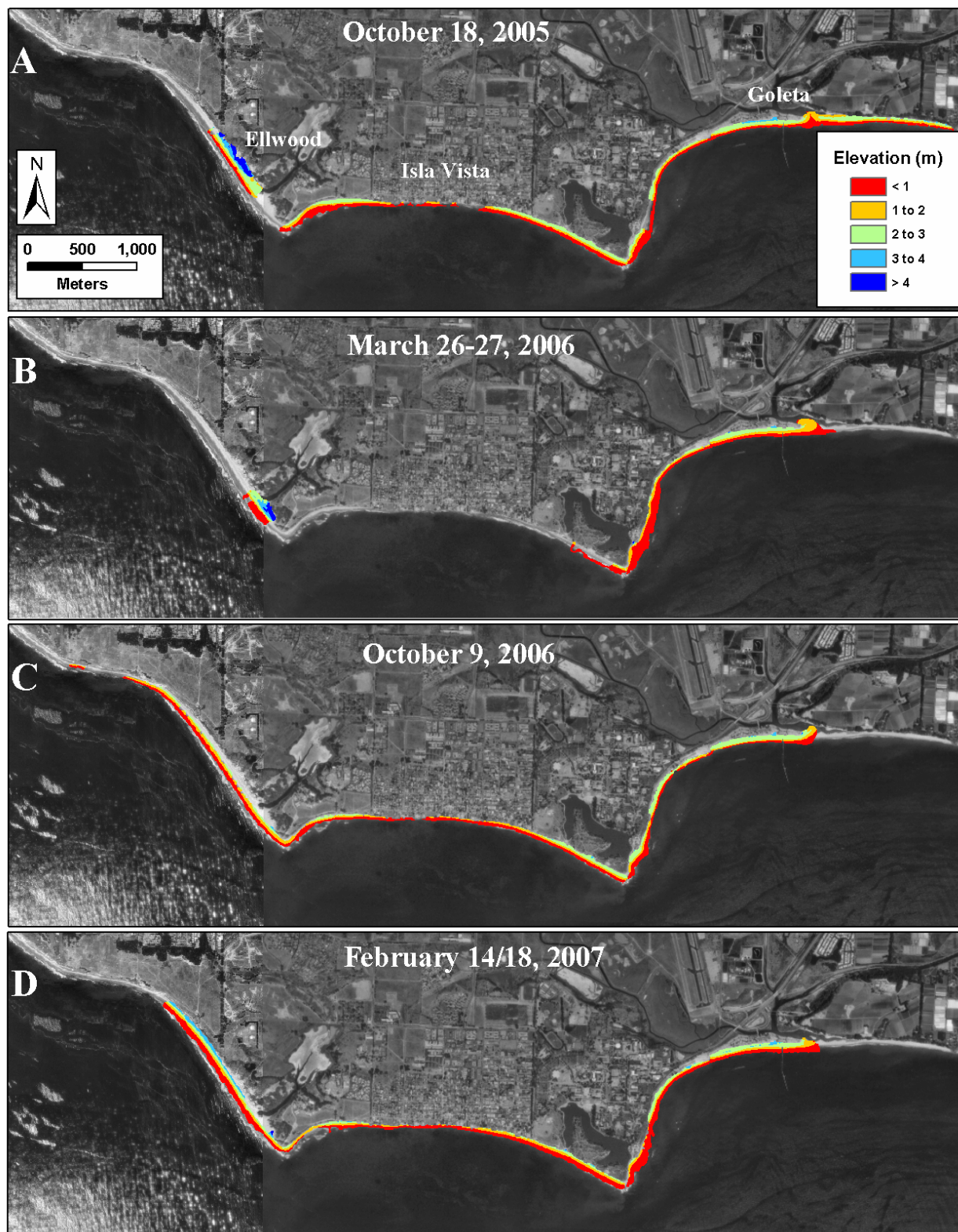
Figure B2. Topographic data gridded to 2 m cells from the Ellwood/Isla Vista/Goleta study site.
