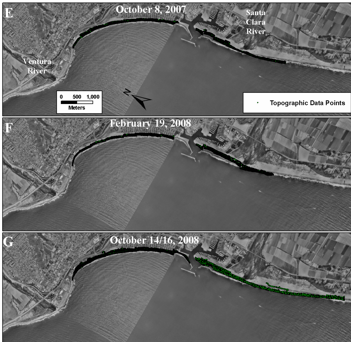
Figure B9 (cont.). Topographic data points collected in the Ventura study site.
