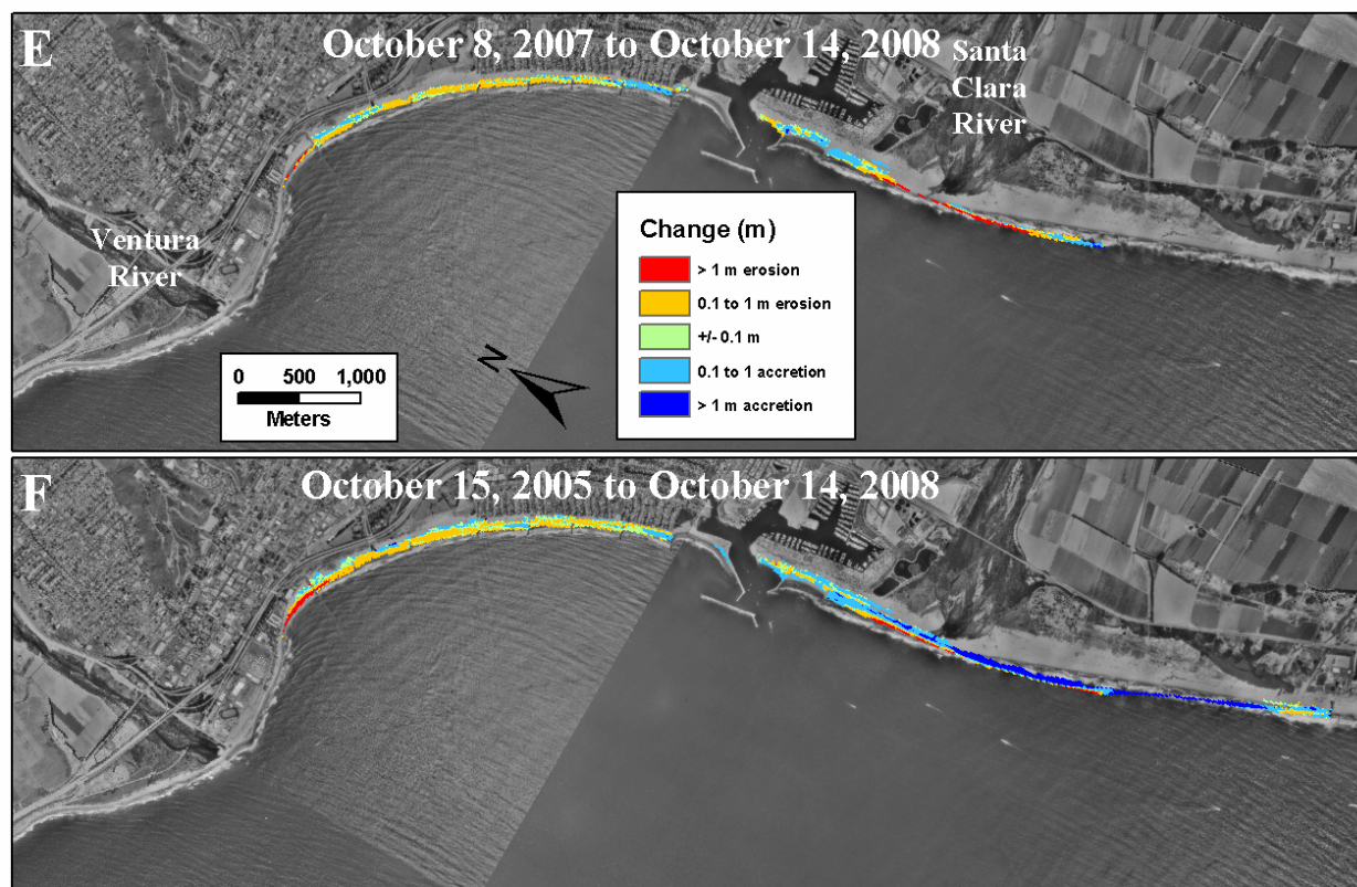
Figure B11 (cont.). Vertical change from the annual surveys in Ventura.
