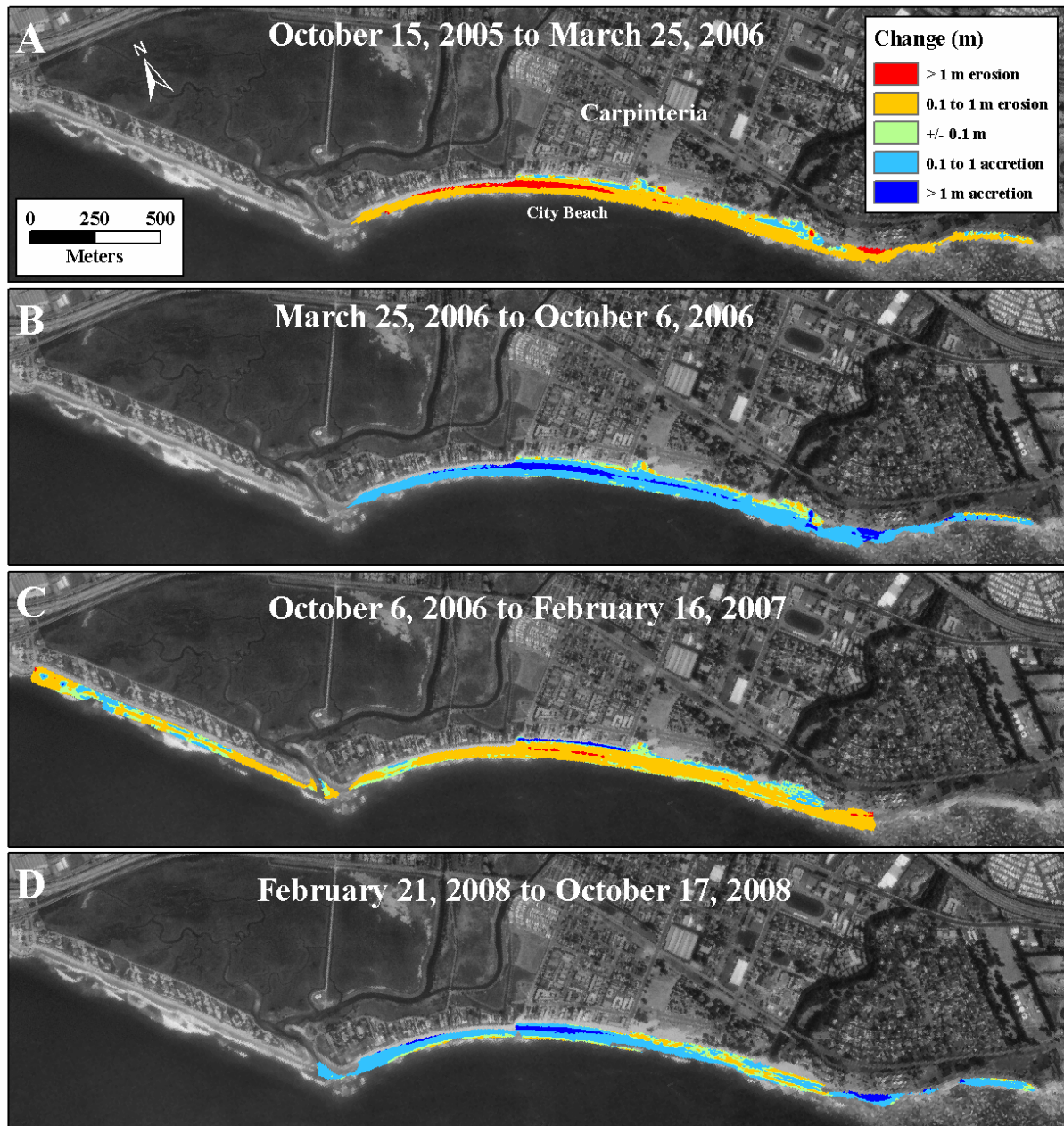
Figure B8. Vertical change from seasonal surveys at the Carpinteria study site.
