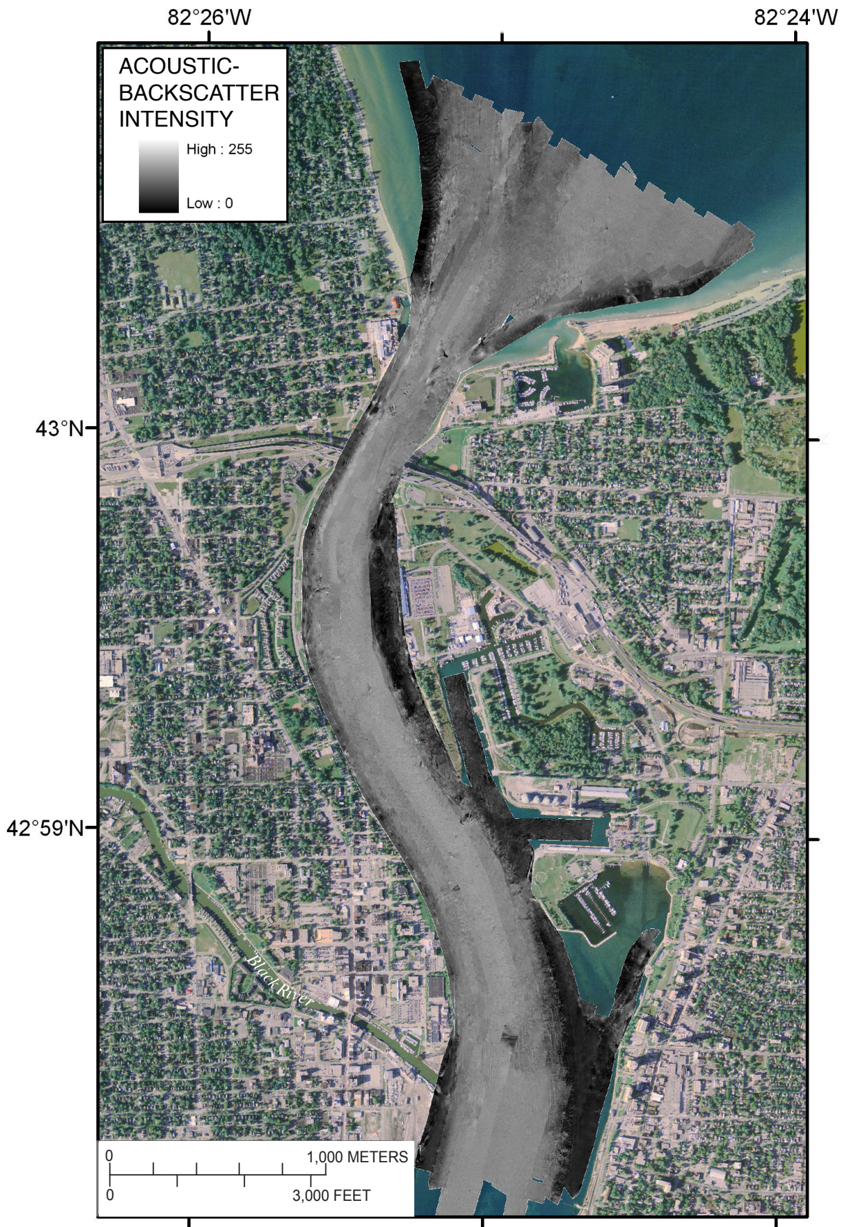
Figure 21. Map showing SWATHplus-processed acoustic backscatter intensity in the northernmost St. Clair River area. Dark areas are lower backscatter and light are higher backscatter. (2005 orthophoto base from Michigan State University, Remote Sensing & GIS Research and Outreach Services, USDA-FSA Aerial Photography Field Office.)
