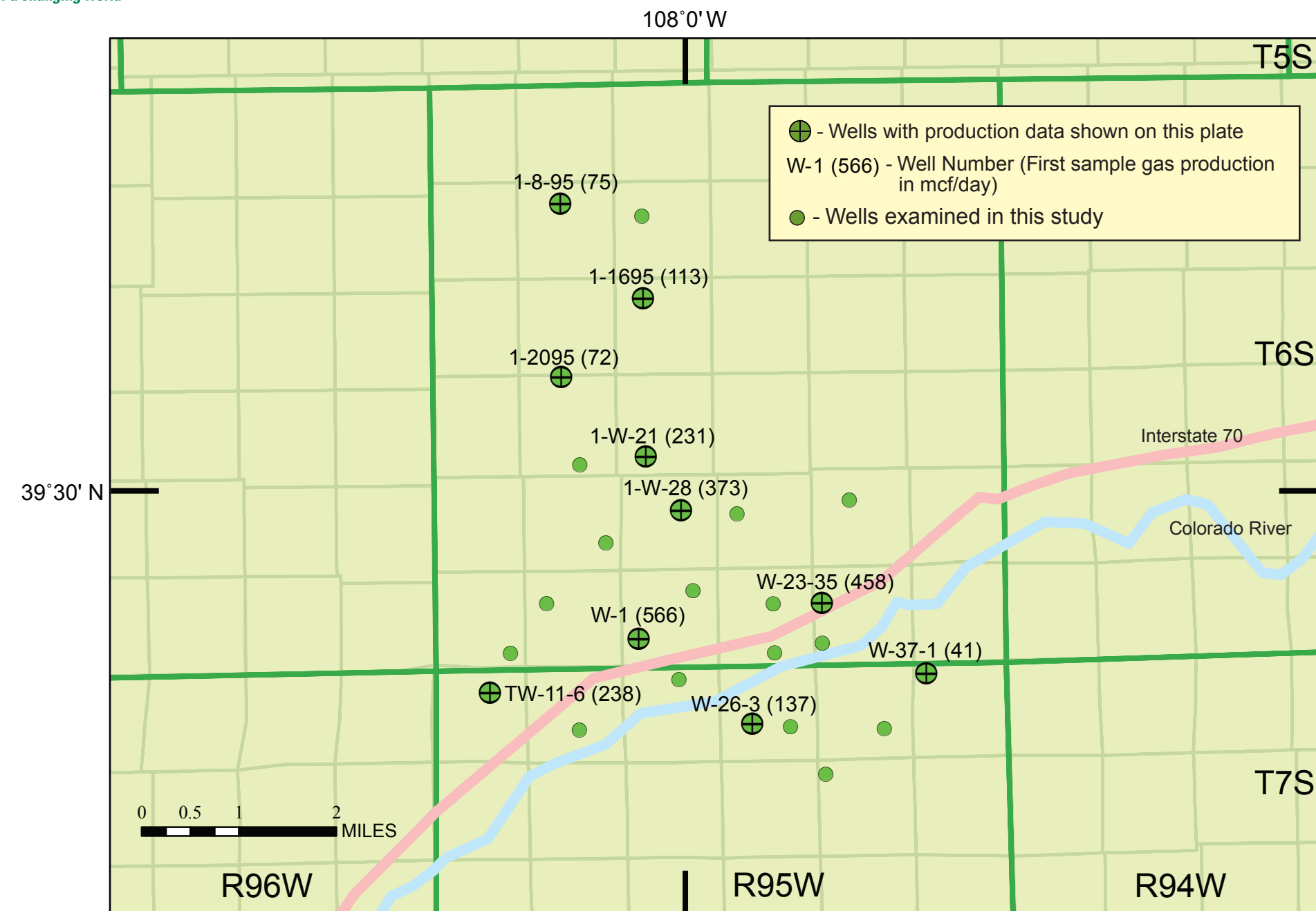
Figure 1-1. Map of wells in this study for the Wasatch Formation, Parachute field.
