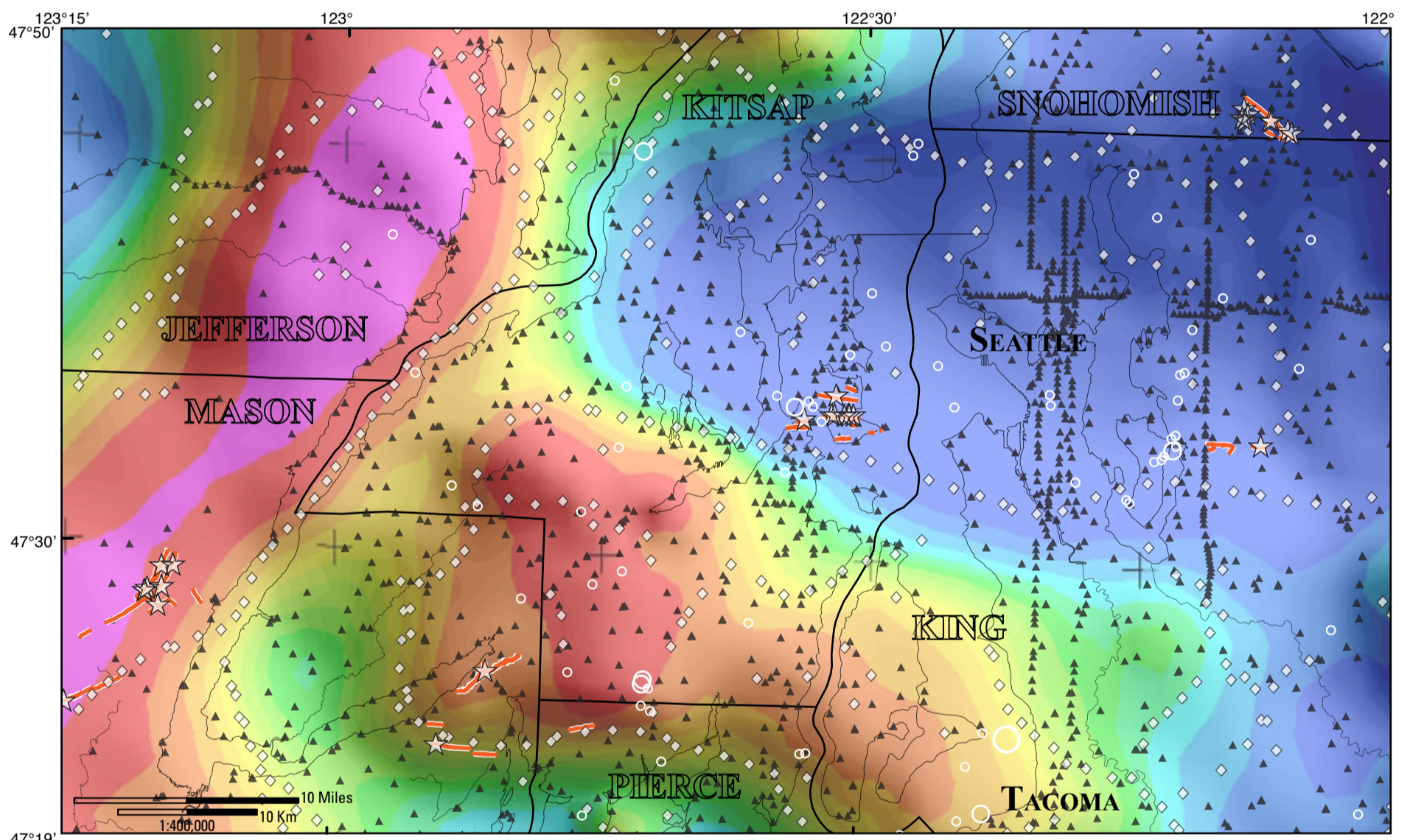
INSET MAP 12: ISOSTATIC RESIDUAL GRAVITY ANOMALIES IN SEATTLE/TACOMA REGION
