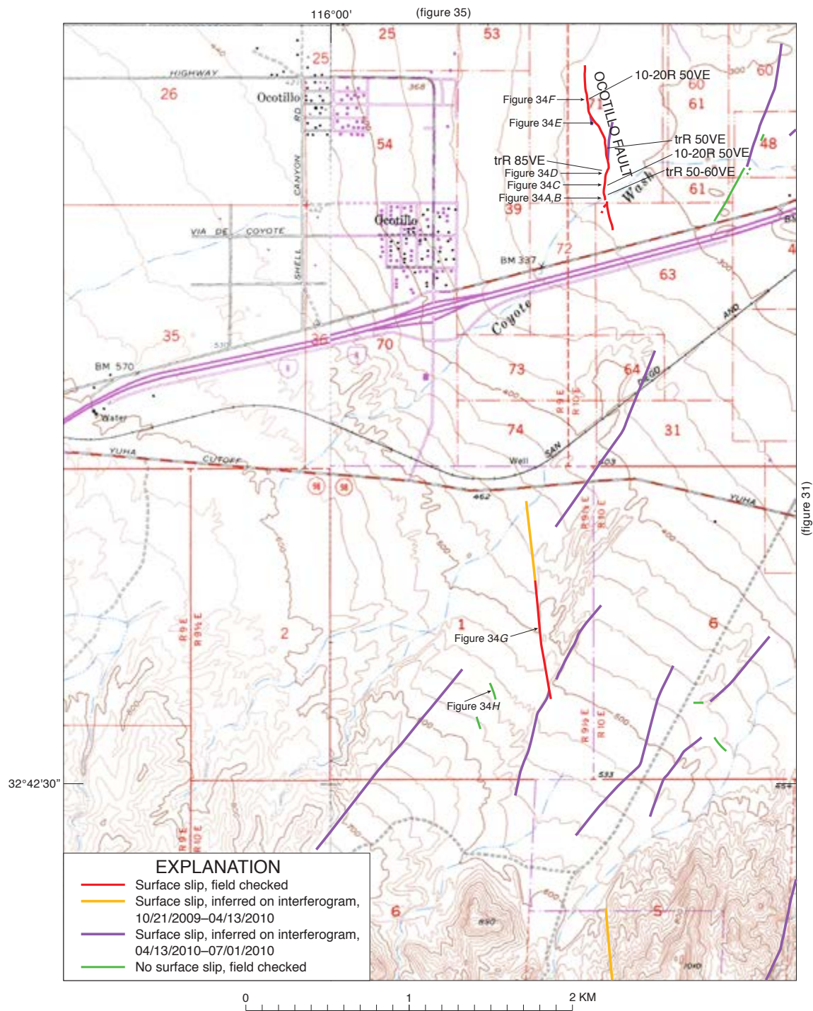
Figure 33. Map of faults and surface fractures in the Yuha Desert surrounding the community of Ocotillo. Amount of slip shown in millimeters for both right-lateral (R) and vertical (V) components. Vertical component of slip, where present, is indicated with either west (W) or east (E) side up. 'tr' indicates trace amount. Map base from portions of the Coyote Wells and In-Ko-Pa Gorge 7 1/2-minute topographic quadrangles. See figure 17 for location of map area.
