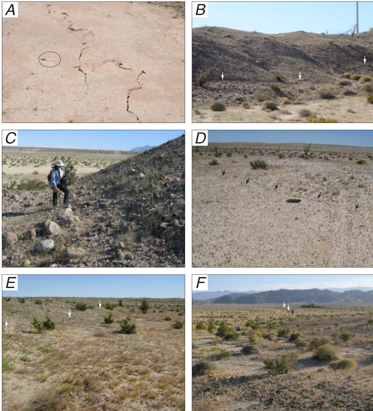
Figure 26. Photographs of fractures and fault scarps along faults shown in figure 25. A , Left-stepping, semicontinuous fractures with right-lateral offset and local “tent” structures along the Laguna Salada Fault, west branch; view to the northwest. Pen (circled) for scale. Photograph taken April 6, 2010. B , Fault scarp (white arrows) along Laguna Salada Fault, west branch. View to the west. Photo C is at leftmost arrow. Photograph taken April 7, 2010, by J.A. Treiman. C , Fault scarp (at change in slope, about 1 m in front of person) along Laguna Salada Fault, west branch; view to the south. Photograph taken April 7, 2010, by J.A. Treiman. D , Fault scarp (at change in slope) with fractures (black arrows) along one of several normal faults within an extensional zone near the juncture between the Laguna Salada Fault Zone and the Yuha Well Fault Zone; view to the north. Photograph taken May 12, 2010, by J.A. Treiman. E , Fault scarp (white arrows) along a northeast-trending fault within the Yuha Well Fault Zone; view to the northeast. Photograph taken April 6, 2010, by J.A. Treiman. F , Fault scarp (white arrows) along a fault within the Yuha Well Fault Zone; view to the southwest. Black arrow (and white outline), vehicle for scale. Photograph taken May 11, 2010, by J.A. Treiman.
