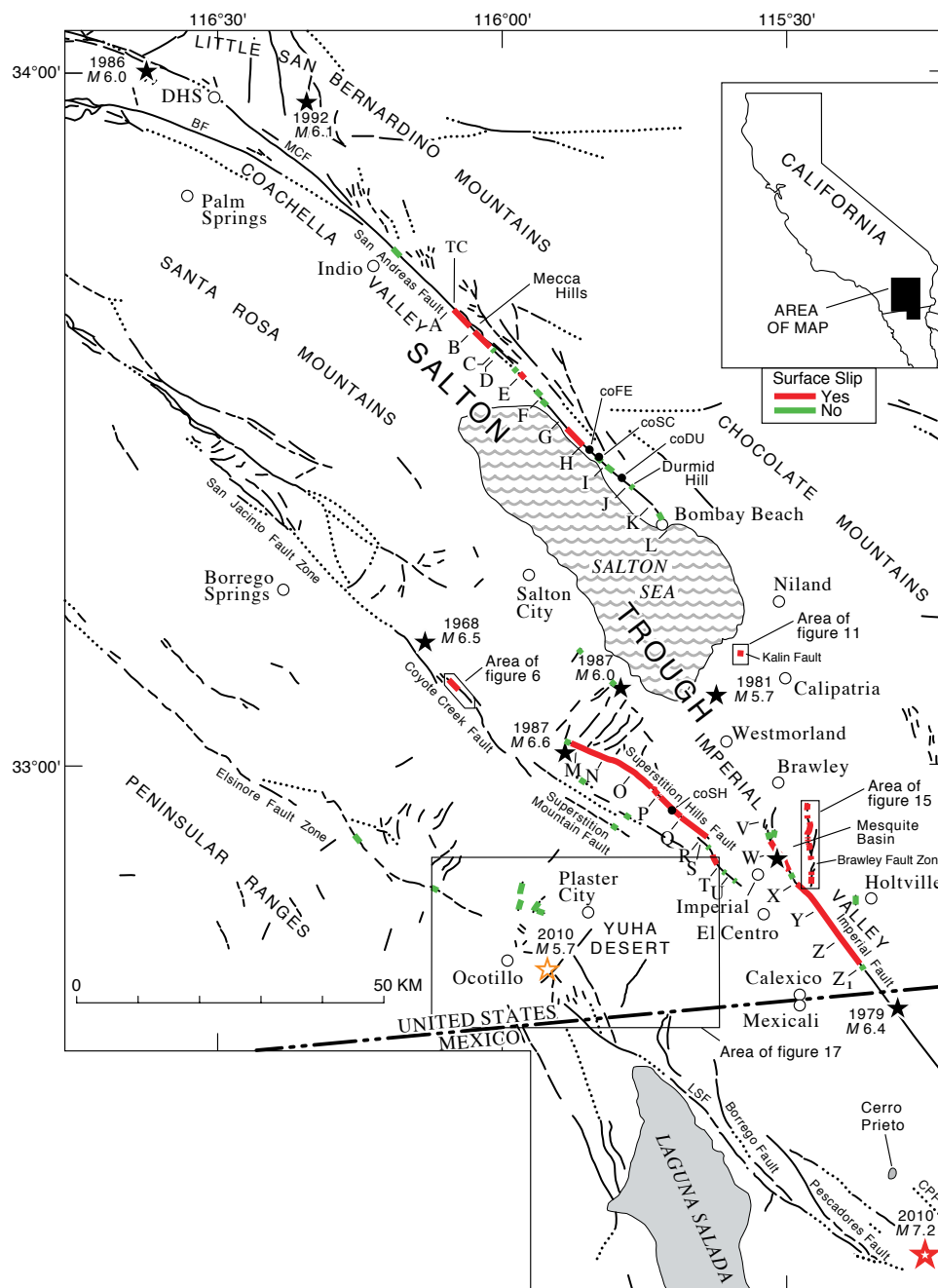
Figure 1. Index map showing Quaternary faults in the greater Salton Trough area (modified from Jennings, 1994). Red bars along faults in central Salton Trough show the generalized location of 2010 surface slip along the San Andreas, Coyote Creek, Superstition Hills, Wienert, Kalin, and Imperial Faults and along the Brawley Fault Zone triggered by the El Mayor-Cucapah earthquake—many additional faults in the Yuha Desert experienced triggered slip (see fig. 17). Green bars along faults show the location of field observations of no slip in 2010. Large red star marks location of El Mayor-Cucapah mainshock epicenter (labeled with magnitude 7.2). Large orange star marks location of June 14, 2010, aftershock (labeled with magnitude 5.7). Small black stars with date and magnitude indicate epicenters of earlier earthquakes that also triggered slip on southern San Andreas, Coyote Creek, Superstition Hills, or Imperial Fault. BF, Banning Fault; DHS, Desert Hot Springs; MCF, Mission Creek Fault; TC, mouth of Thermal Canyon. Letters A to L mark location of ends of strip maps of San Andreas Fault, shown in figure 4; letters M to R mark location of ends of strip maps of Superstition Hills Fault, shown in figure 8; letters S to U mark location of ends of strip maps of Wienert Fault, shown in figure 10; letters V to Z, mark location of ends of strip maps of Imperial Fault, shown in figure 13. Black dots show the location of creepmeter stations (coFE, Ferrum; coSC, Salt Creek; coDU, Durmid Hill; and coSH, Superstition Hills).
