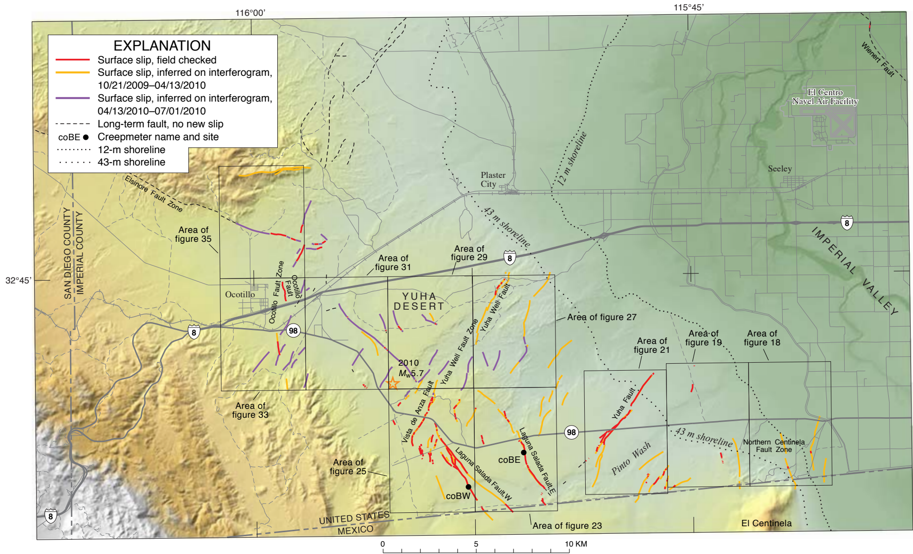
Figure 17. Shaded-relief map with background of roads, towns, and faults in the greater Yuha Desert area (see fig. 1 for location of map); also shown are areas of figs. 18, 19, 21, 23, 25, 27, 29, 31, 33, and 35. Red lines, field-verified surface fractures; orange lines, location of surface fractures inferred from dislocations in UAVSAR interferograms. Orange star, location of M_w 5.7 aftershock epicenter. Highstand of ancient Lake Cahuilla (12-m shoreline) and an earlier lake (43-m shoreline) are shown with dotted lines. Black dots show the location of creepmeter stations.
