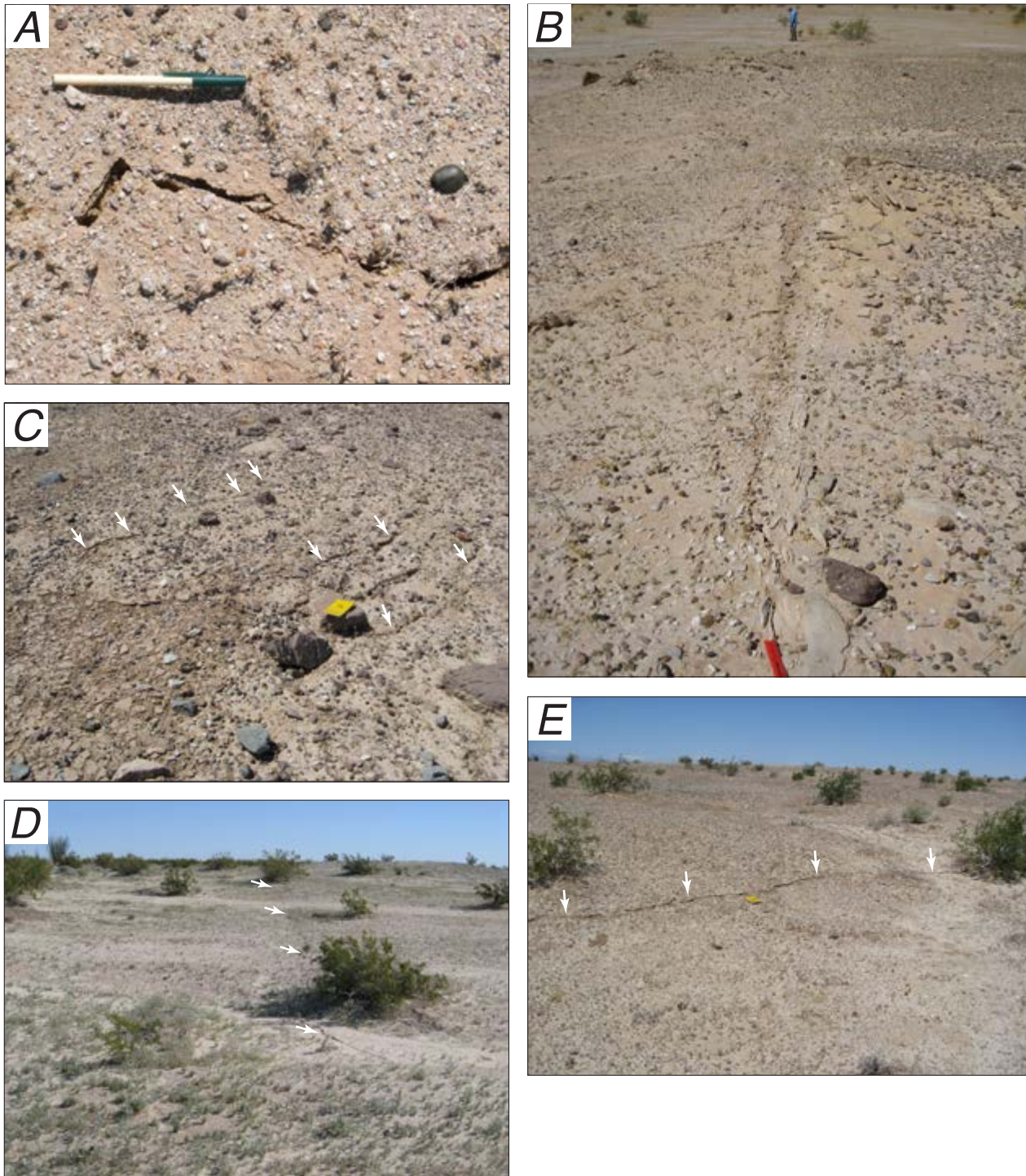
Figure 22. Photographs of fractures and Quaternary fault scarps along faults shown in figure 21. A , Left-lateral fractures along unnamed fault south of Pinto Wash, pen for scale. Photograph taken June 18, 2010. B , Continuous left-lateral fractures along unnamed fault south of Pinto Wash (surface slip extends between red scale in foreground and geologist in distance); view to the southwest. This section of fault consists of a cemented shear zone. Photograph taken June 18, 2010, by J.A. Treiman. C , Shattered and overturned surface crust. Shattered ground may be partly a topographic effect, given that the site is on a low ridge adjacent to a fault (as indicated by UAVSAR interferogram), which had no new surface fault breakage. There may also be some lateral spread of the ridge toward a wash
