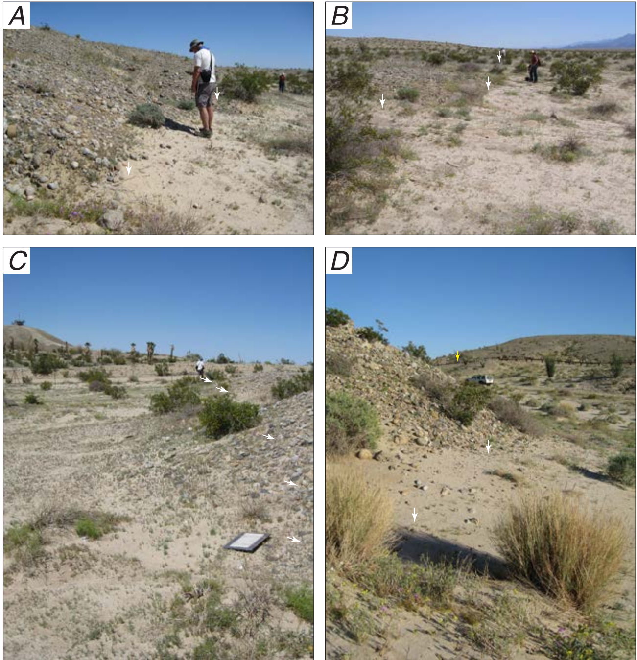
Figure 24. Photographs of fractures and fault scarps along faults shown in figure 23. A , Fault scarp (at change in slope) with fractures (white arrows) along the east branch of the Laguna Salada Fault; view to the south. Photograph taken April 6, 2010, by J.A. Treiman. B , Fault scarp (at change in slope) with fractures (white arrows) along east branch of the Laguna Salada Fault; view to the south. Photograph taken April 6, 2010, by J. A. Treiman. C , Fault scarp (at change in slope) with fractures (white arrows) along east branch of the Laguna Salada Fault; view to the north. Photograph taken April 6, 2010, by J.A. Treiman. D , Fault scarp (at change in slope) with fractures (white arrows) along east branch of the Laguna Salada Fault; view to the south. Location of U.S.-Mexico border fence marked with yellow arrow. Photograph taken April 8, 2010, by J.A. Treiman.
