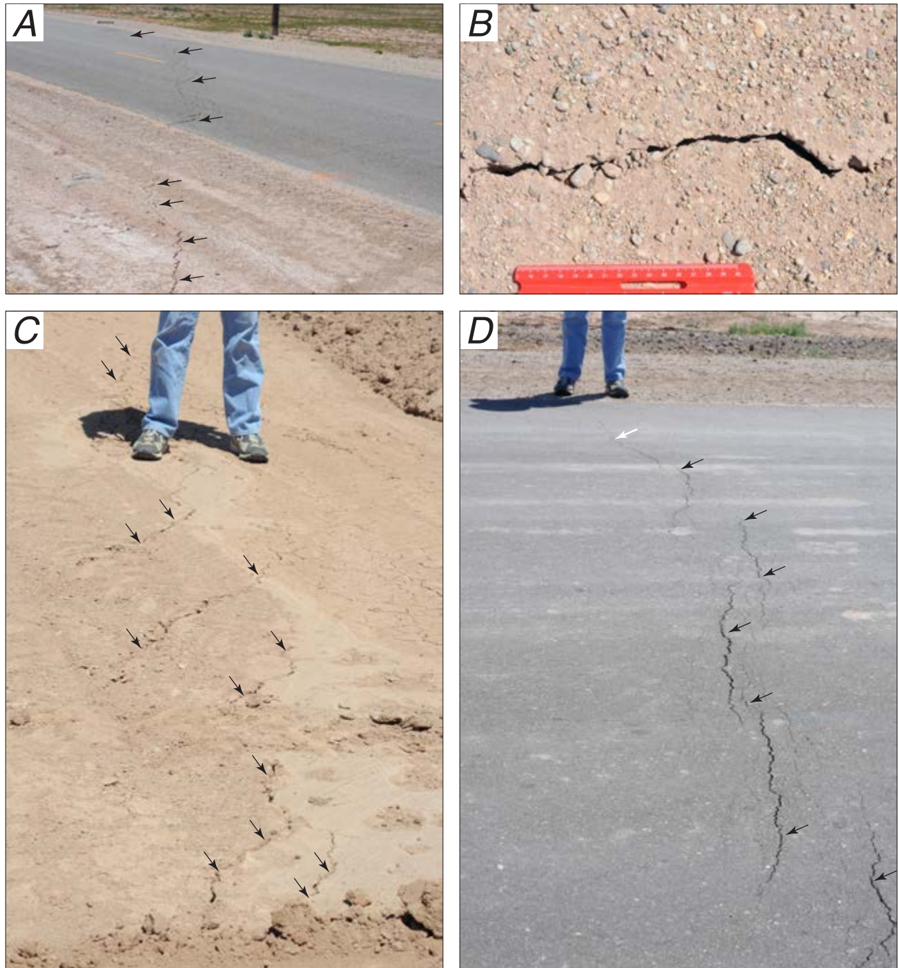
Figure 16. Photographs of surface fractures along Brawley Fault Zone in response to the 2010 El Mayor-Cucapah earthquake. A , Surface fractures (black arrows) along Brawley Fault Zone and across McConnell Road; view to the southwest. Photograph taken April 9, 2010. B , Close-up view of fresh surface fractures along Brawley Fault Zone in shoulder of Harris Road; scale in centimeters. Photograph taken April 9, 2010. C , Left-stepping, fractures (black arrows) along Brawley Fault Zone and across shoulder of Harris Road; view to the north. Photograph taken April 9, 2010. D , Fresh surface fractures (black arrows) along Brawley Fault Zone and across Ralph Road; view to the north. Slight vertical component of slip (2 mm, up on east [right] side) more noticeable at white arrow. Photograph taken April 9, 2010.
