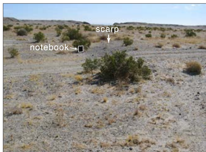
Figure 36. Photograph of fault scarp along fault farther northeast of surface slip in 2010 (see fig. 35 for location). Small white arrow points to black notebook (with white outline) for scale. Photograph taken August 3, 2010, by J.A. Treiman.
