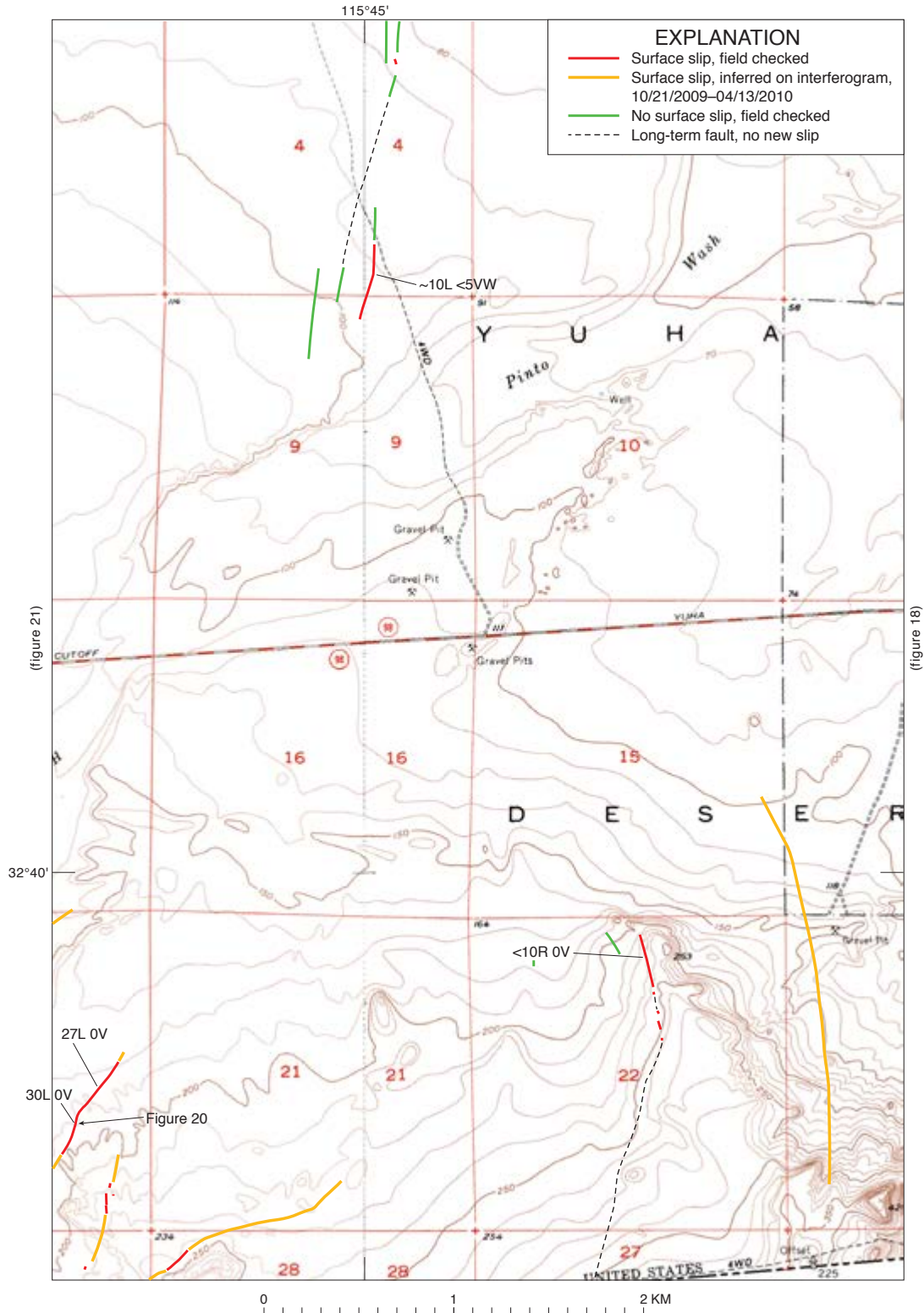
Figure 19. Map of faults and surface fractures in eastern Yuha Desert. Faults shown include elements of the Northern Centinela Fault Zone (Sections 14 and 15, 22 and 23), Yuha Fault (sections 4 and 9) and faults south of Pinto Wash (Section 20, 21, 28, and 29). Amount of slip shown in millimeters for both right-lateral (R), or left-lateral (L), and vertical (V) components. Vertical component of slip, where present, is indicated with either west (W) or east (E) side up. Map base from portions of the Mount Signal and Yuha Basin 7 1/2-minute topographic quadrangles. See figure 17 for location of map area.
