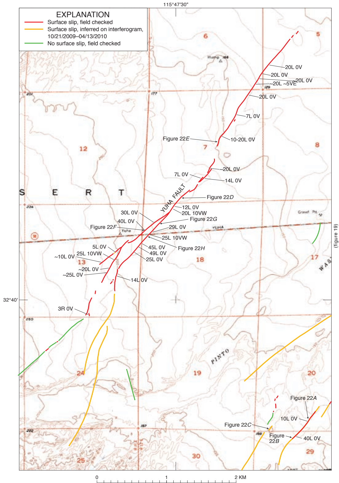
Figure 21. Map of faults and surface fractures in central Yuha Desert. Faults shown are the Yuha Fault and several faults south of Pinto Wash (Sections 20, 29–30). Amount of slip shown in millimeters for both right-lateral (R), or left-lateral (L), and vertical (V) components. Vertical component of slip, where present, is indicated with either west (W) or east (E) side up. Map base from a portion of the Yuha Basin 7 1/2-minute topographic quadrangle. See figure 17 for location of map area.
