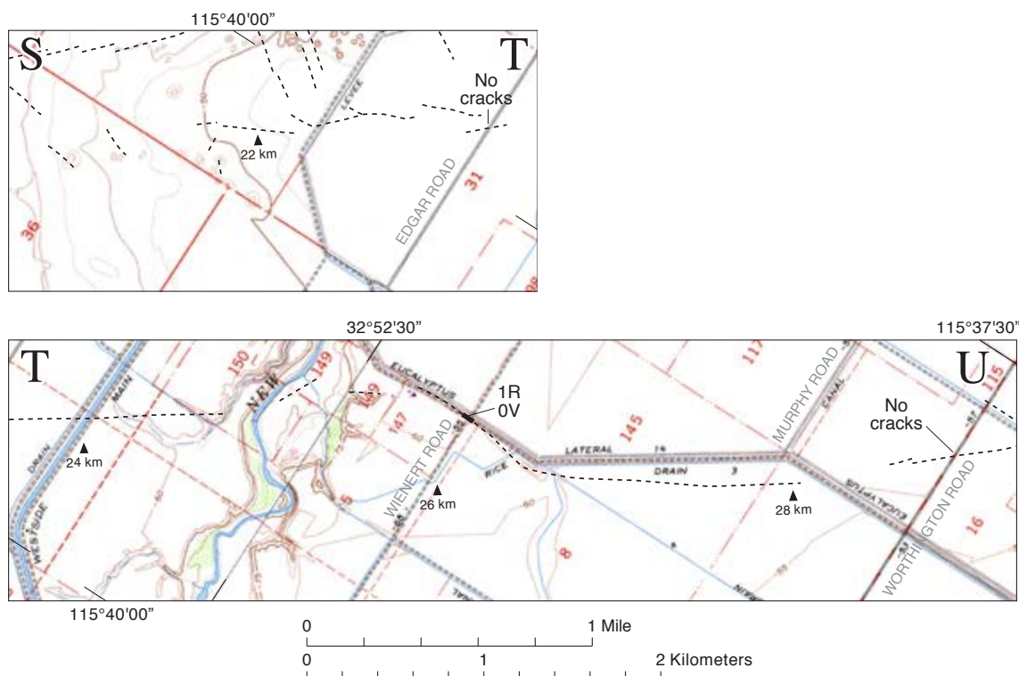
Figure 10. Strip maps of Wienert Fault (Wienert strand of the Superstition Hills Fault) with location of surface fractures formed in response to 2010 El Mayor-Cucapah earthquake (see fig. 1 for location of panels S–U). Dotted line, Wienert Fault; solid line, location of documented 2010 surface fractures. Amount of slip shown in millimeters for both right-lateral (R) and vertical (V) components. Map strips derived from topographic maps. Distance scale along fault is the same as used by Sharp and others (1989), with reference point located near western end of Superstition Hills Fault.
