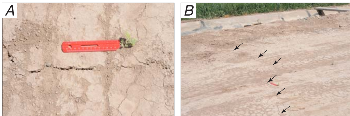
Figure 12. Photographs of Kalin Fault and surface fractures formed in response to the 2010 El Mayor-Cucapah earthquake. A , Vertical view of fractures with 14-cm-long scale. B , View of fractures across dirt roadway. Concrete canal liner (at top of photo) was not broken by new fractures. Photographs taken April 10, 2010.
