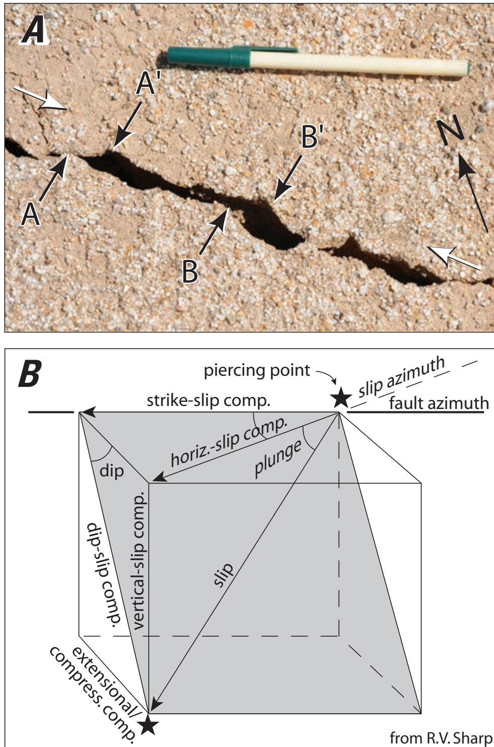
Figure 3. Photograph and diagram showing determination of components of slip. A , Photograph of fracture along Laguna Salada Fault, east branch. Corresponding piercing points A and A' and B and B' (black arrows) constrain the calculated amount of right-lateral strike-slip component of displacement (see fig. 25 for location). White arrows, orientation of local fault azimuth. Right-lateral component of displacement at time of photograph was 20 mm; photograph taken April 6, 2010. B , Schematic block diagram showing components of fault slip and how to calculate fault parallel component of displacement (see text for explanation).
