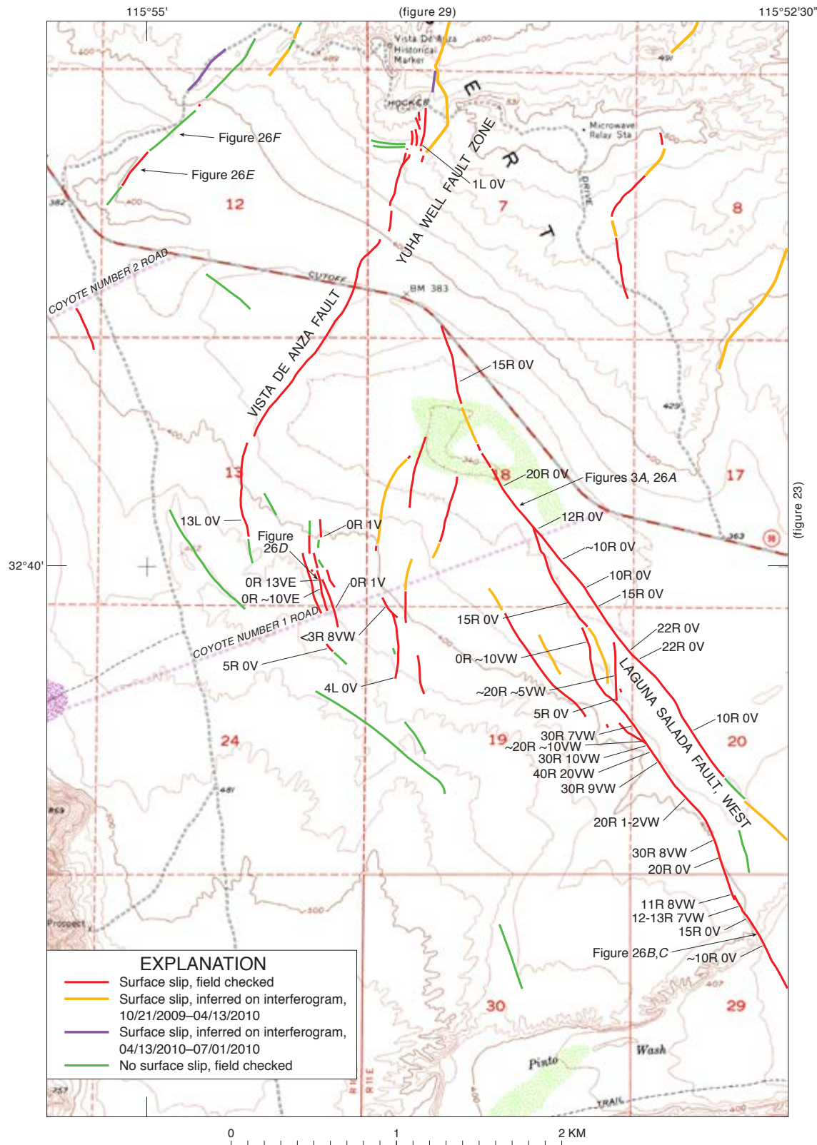
Figure 25. Map of faults and surface fractures in the central Yuha Desert. Faults include the west branch of the Laguna Salada Fault and the southwestern end of the Yuha Well Fault Zone. Amount of slip shown in millimeters for both right-lateral (R), or left-lateral (L), and vertical (V) components. Vertical component of slip, where present, is indicated with either west (W) or east (E) side up. Map base from a portion of the Coyote Wells 7 1/2-minute topographic quadrangle. See figure 17 for location of map area.
