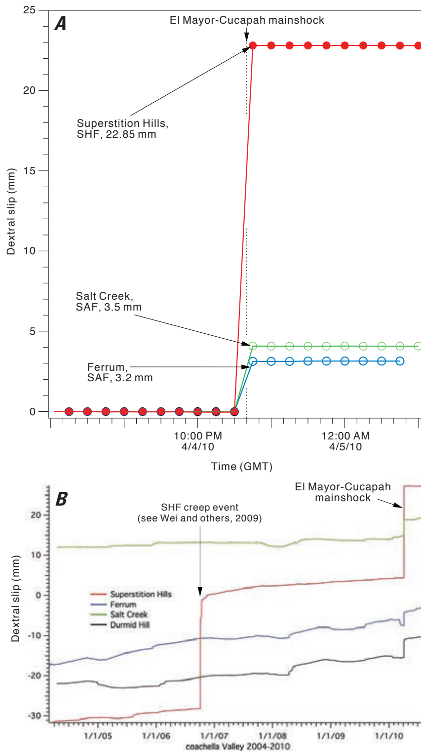
Figure 2. Creepmeter data that show timing of slip on the San Andreas and Superstition Hills Faults in association with the EI Mayor-Cucapah earthquake. A , Detailed plot of creepmeter data for three sites in a 6-hr period approximately centered on the EI Mayor-Cucapah earthquake. Data plotted with normalized zero slip before the earthquake. The circles are 10-minute samples. B , Plot of a 6-yr period (2004–2010) of creepmeter data. Included in these data is the start of a large creep event on the Superstition Hills Fault (SHF) in October 2006 (see Wei and others, 2009) compared to the abrupt triggered slip recorded on April 4, 2010. Plot shows low background creep rates on fault segments (1–3 mm/yr) interrupted by episodic creep events and triggered slip. Left-lateral excursions (negative slopes) in the data follow rainfall on Durmid Hill. Note that the creep rates on the San Andreas Fault remain high after the EI Mayor-Cucapah earthquake. Transmission problems at both Salt Creek and Ferrum resulted in data gaps following the earthquake that have been interpolated in this plot. The data from Durmid Hill are continuous and confirm the resumption of preseismic creep rates immediately after the triggered slip event. In contrast, the post-earthquake creep rate on the Superstition Hills Fault is slower than the pre-event rate.
