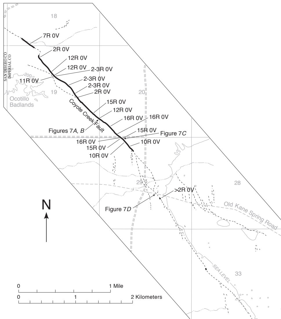
Figure 6. Strip map of central part of Coyote Creek Fault showing location of fractures formed in response to 2010 El Mayor-Cucapah earthquake (see fig. 1 for location of map area). Amount of slip shown in millimeters for right-lateral (R) and vertical (V) components. Map derived using selected contours from topographic maps; location of faults from Clark (1972). Map covers same section of Coyote Creek Fault as shown by Hudnut and Clark (1989).
