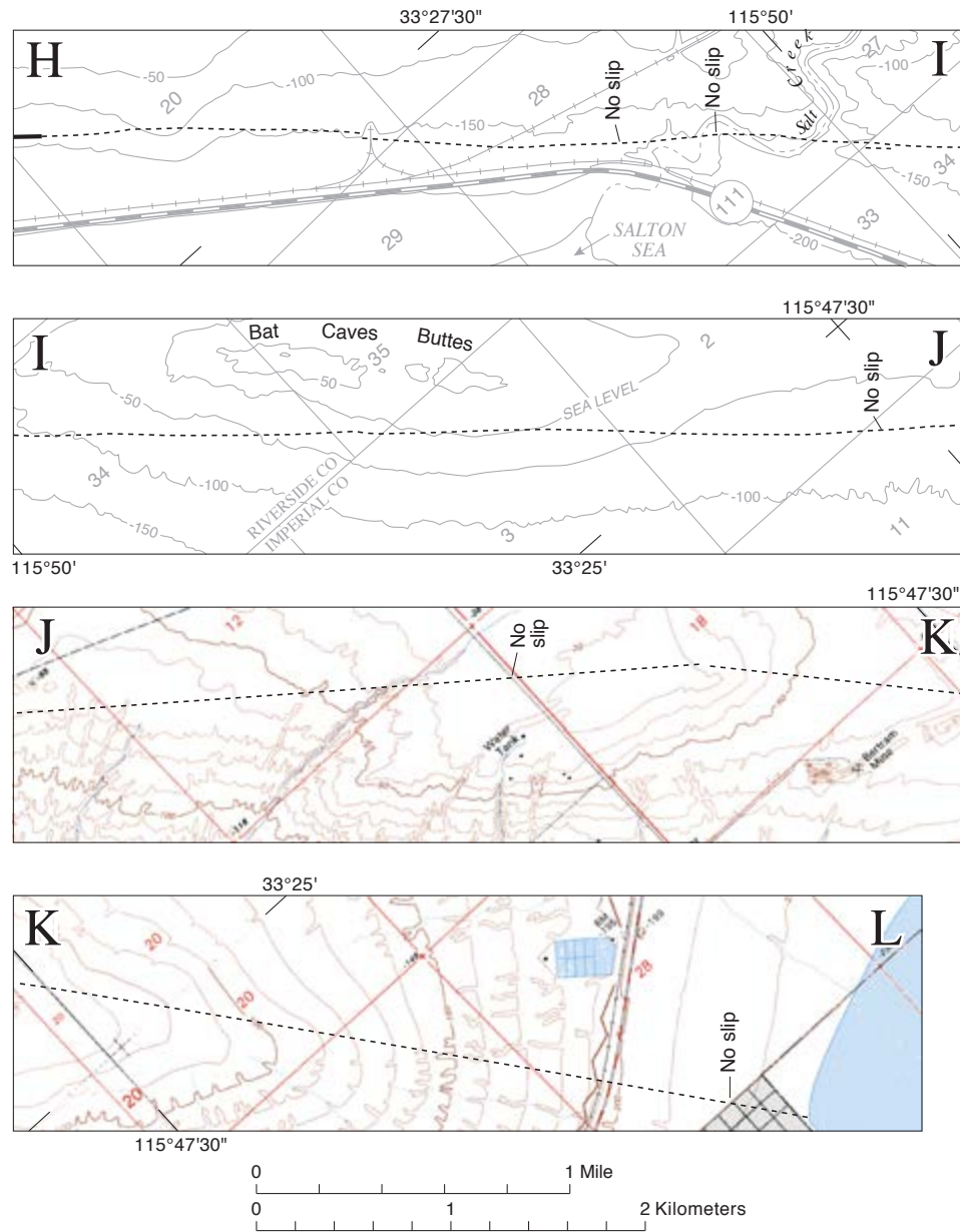
Figure 4. Strip maps from northwest to southeast (A to L) along the southern San Andreas Fault with location of surface fractures formed in response to 2010 El Mayor-Cucapah earthquake. Dashed line, San Andreas Fault; solid line, location of documented 2010 surface fractures. Amount of slip shown in millimeters for right-lateral (R) and vertical (V) components. Maps derived using selected contours from 1:24,000-scale topographic maps; location of fault from Clark (1984); location of strips shown in figure 1.
