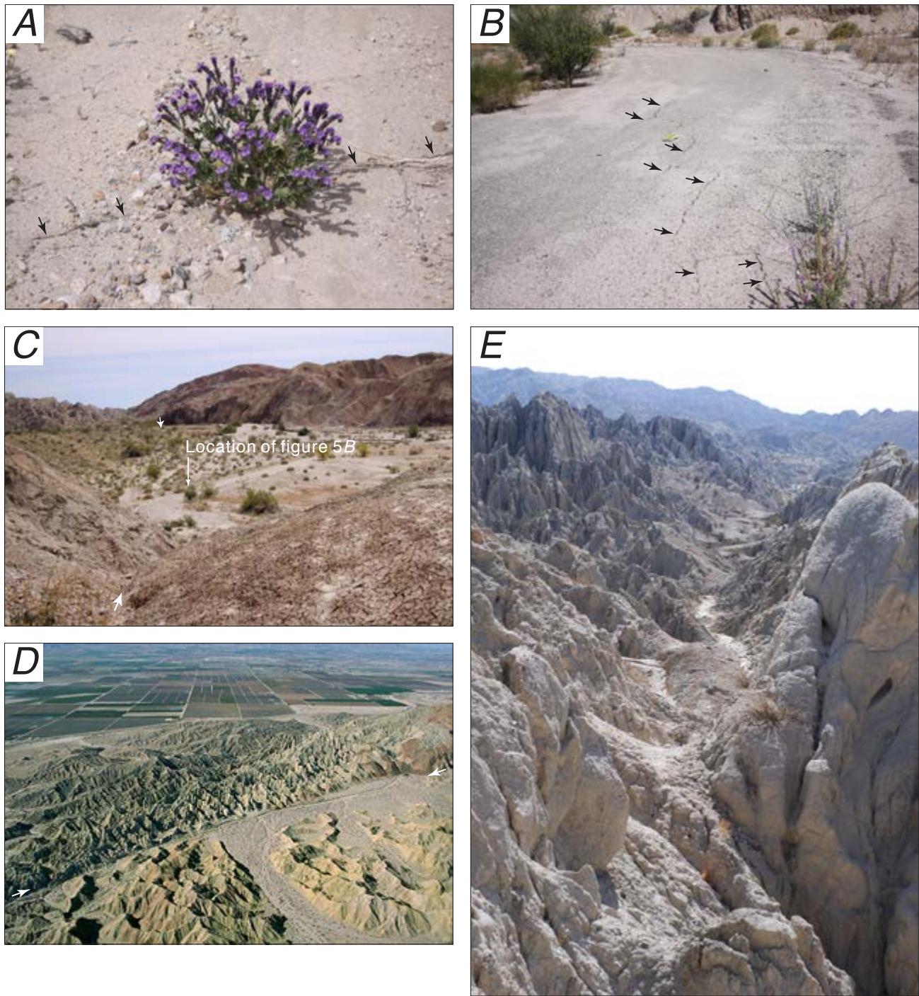
Figure 5. Photographs of fractures formed in response to the El Mayor-Cucapah earthquake and views of the San Andreas Fault in southeastern Coachella Valley. A , Fractures (black arrows) along San Andreas Fault in active wash between Thermal Canyon and Quarry Canyon; view to the northeast (see fig. 4, panel A–B for location). Photograph taken April 20, 2010, by K.J. Kendrick. B , Left-stepping fractures (black arrows) along San Andreas Fault in gravel road in Quarry Canyon. Photograph taken April 20, 2010, by K.J. Kendrick; view to the northwest. Green notebook in center of view for scale. C , View along San Andreas Fault (between white arrows) in Quarry Canyon; view to the southeast. Photograph taken April 20, 2010, by K.J. Kendrick. D , Oblique aerial view of San Andreas Fault (between white arrows) near Red Canyon; view to the west. Location of image shown in figure 4, panel B–C. Dark reddish-brown deposit beyond right white arrow is a sandy mudstone that was tectonically emplaced along this section of the San Andreas Fault. E , View along San Andreas Fault between Red Canyon and Painted Canyon; view to the southeast.
