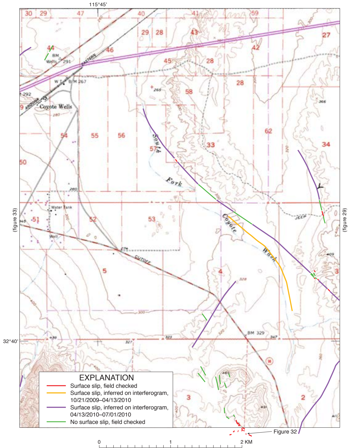
Figure 31. Map of faults and surface fractures in Yuha Desert. The principal structure is the inferred northwest extension of the Laguna Salada Fault. Map base from a portion of the Coyote Wells 7 1/2-minute topographic quadrangle. See figure 17 for location of map area.
