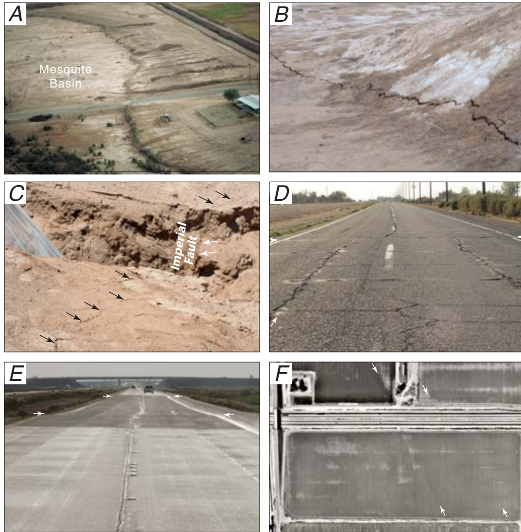
Figure 14. Photographs of surface fractures and long-term offset of features along the Imperial Fault. A , Aerial photograph of the Imperial Fault at Harris Road. Photograph taken October 1979, shortly after the 1979 Imperial Valley earthquake. View to the southwest. B , Locally continuous, right-oblique surface fractures along Imperial Fault; view to the southwest. Photograph taken about 70 m south of Harris Road; photograph shows about 4 meters of surface fractures. Photograph taken April 5, 2010. C , Right-lateral surface fractures along Imperial Fault across and through a paleoseismic trench exposure. Photograph shows surface fractures (black arrows) and fresh fractures in a vertical exposure in the trench wall (white arrows), along edge of long-term Imperial Fault; view to the south. Photograph taken April 11, 2010. D , Right-lateral fault offset at Evan Hewes Highway due to recurrent movement on the Imperial Fault. View to the west. Photograph taken March 12, 2009; roadway was resurfaced some time between June 2009 and April 2010. E , Right-lateral fault offset at I-8 due to recurrent movement on the Imperial Fault; view to the east. Photograph taken April 11, 2010. F , Vertical aerial photograph of the Imperial Fault and I-8, showing two fault traces (between white arrows) in a structural stepover (compare with fault map in fig. 13). North is at top in this view. Photograph taken October 16, 1979.
