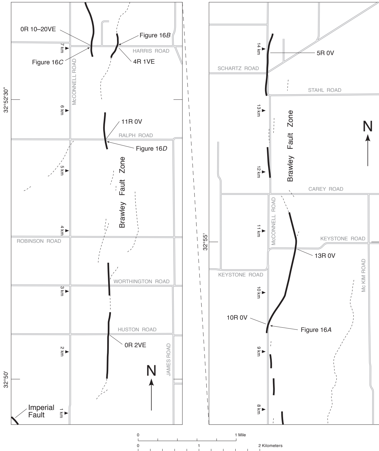
Figure 15. Strip maps of Brawley Fault Zone with location of surface fractures formed in response to 2010 El Mayor-Cucapah earthquake (see fig. 1 for location of map strips). Dotted line, Brawley Fault Zone; solid line, location of documented 2010 surface fractures. Amount of slip shown in millimeters for both right-lateral (R) and vertical (V) components. Vertical component of slip, where present, indicated with either west (W) or east (E) side up. Map strips depict local roads from Holtville West and Alamo 7 1/2-minute topographic maps. Distance scale along fault is the same as used by Sharp and others (1982), with reference point located near southern end of Imperial Fault.
