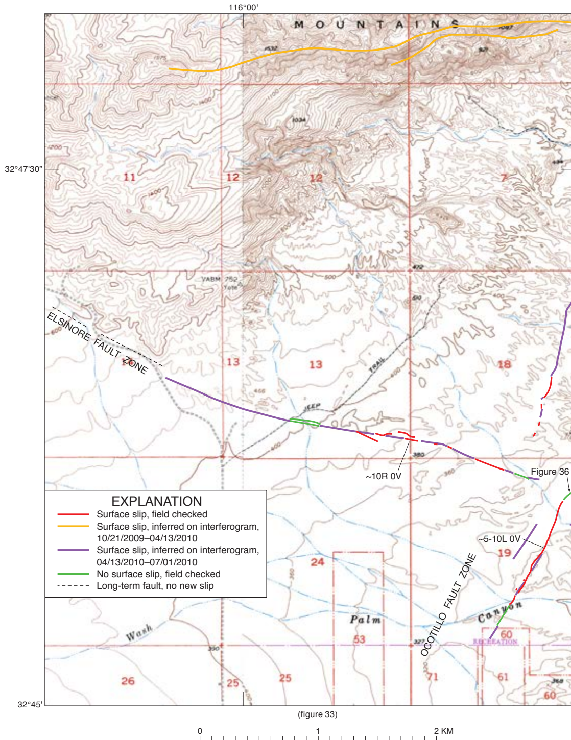
Figure 35. Map of faults and surface fractures in Yuha Desert. Amount of slip shown in millimeters for both right-lateral (R), or left-lateral (L), and vertical (V) components. Map base from portions of the Painted Gorge and Carrizo Mountain 7 1/2-minute topographic quadrangles. See figure 17 for location of map area.
