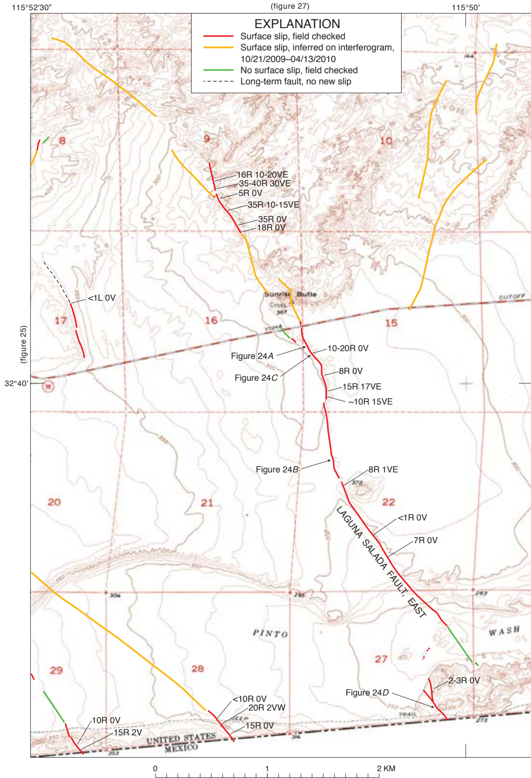
Figure 23. Map of faults and surface fractures in central Yuha Desert. Amount of slip shown in millimeters for both right-lateral (R), or left-lateral (L), and vertical (V) components. Vertical component of slip, where present, is indicated with either west (W) or east (E) side up. Map base from a portion of the Yuha Basin 7 1/2-minute topographic quadrangle. See figure 17 for location of map area.
