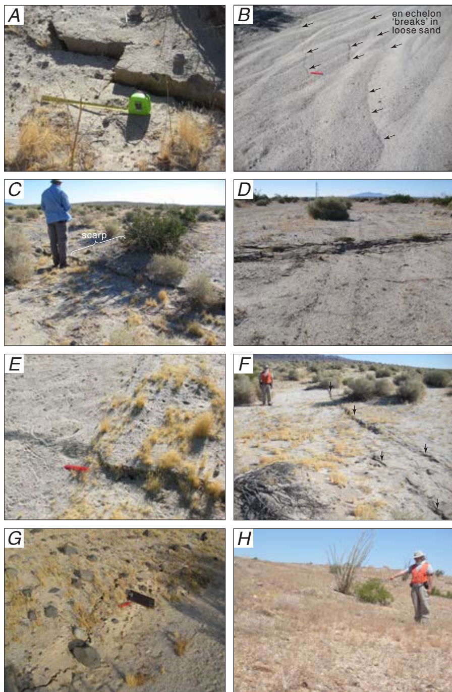
Figure 34. Photographs of fractures and fault scarps along faults shown in figure 33. A , Vertical surface fractures along Ocotillo Fault. Faulting here is associated with the nearby M_w 5.7 aftershock of June 14, 2010. Photograph taken June 16, 2010. B , Left-stepping, right-oblique surface fractures along Ocotillo Fault in loose sand. Photograph shows en echelon 'breaks' (black arrows) in loose sand, suggestive of slight right-lateral component of slip; red ruler for scale. Photograph taken June 16, 2010. C , Fractures along Ocotillo Fault at base of preexisting west-facing scarp. View to northeast. Photograph taken June 16, 2010, by J.A. Treiman. D , Fractures along Ocotillo Fault in recent wash deposits; view to the southeast. Photograph taken June 16, 2010, by J.A. Treiman. E , Right-oblique fractures along Ocotillo Fault. Photograph includes brittle fault movement (on right) and diffuse fault slip in loose sand (on left). Loose sand section in this view includes fresh track from a sidewinder rattlesnake (to the left of red scale). Photograph taken June 16, 2010. F , Fractures with vertical slip along Ocotillo Fault in sandy soil; view to the north. Subtle fault scarp on east (right) side of fault. Photograph shows local structural complexity in rupture (in foreground). Photograph taken June 16, 2010. G , Right-lateral fractures along unnamed fault south of I-8. Black notebook and red ruler for scale. Photograph taken August 2, 2010, by J.A. Treiman. H , Photograph of scarp, about 1.5–2 m high, without fresh surface fractures; view to the northwest. Photograph taken June 16, 2010.
