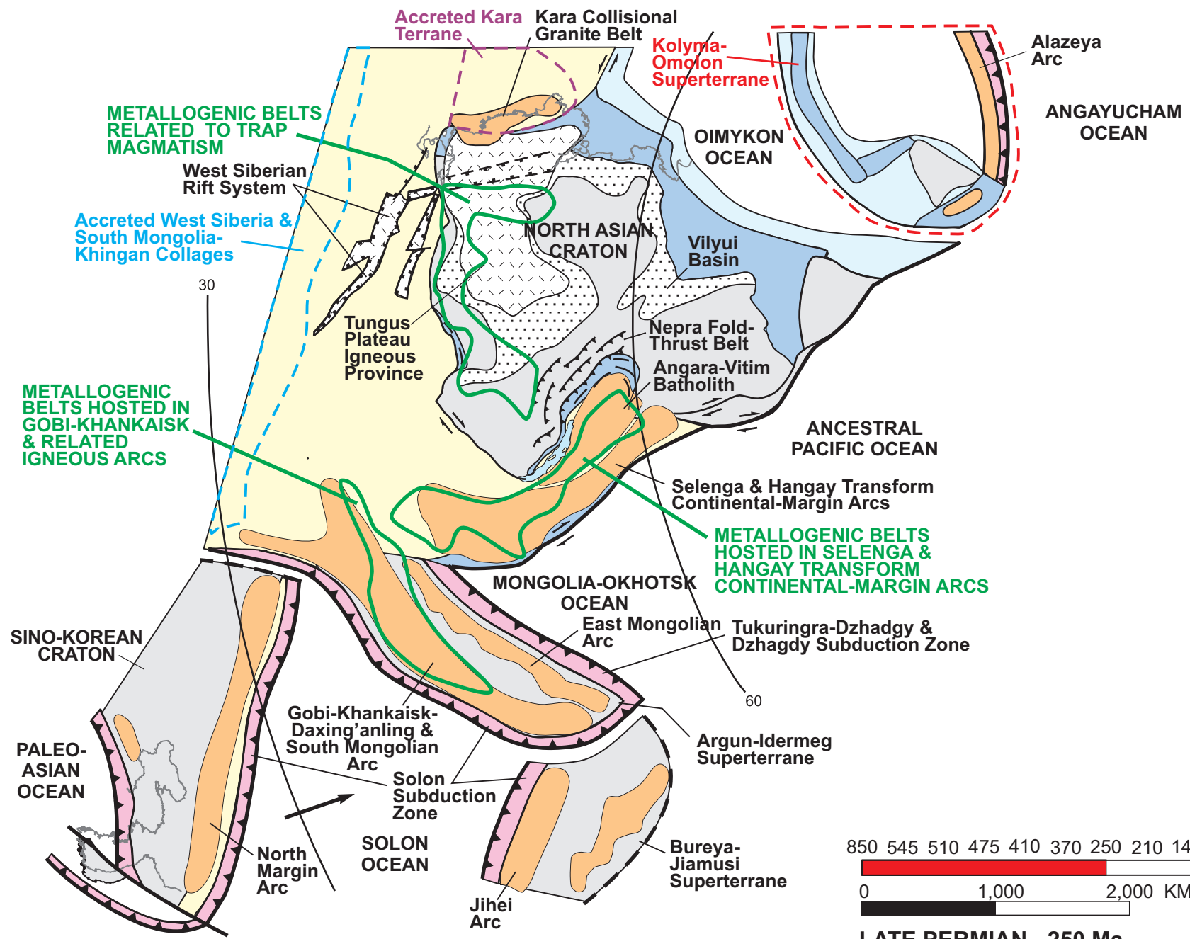
LATE PERMIAN - 250 Ma
