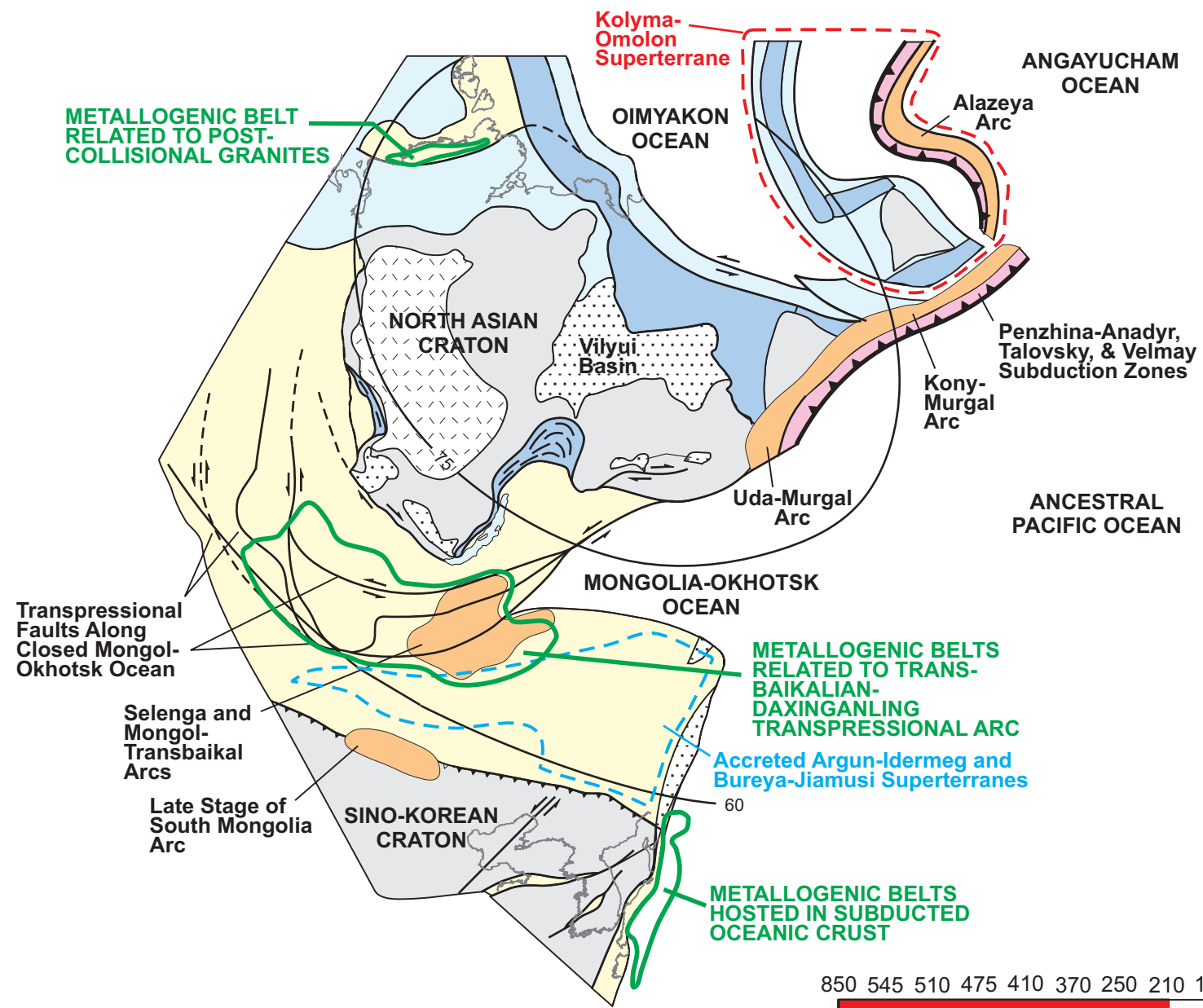
LATE TRIASSIC - 210 Ma
