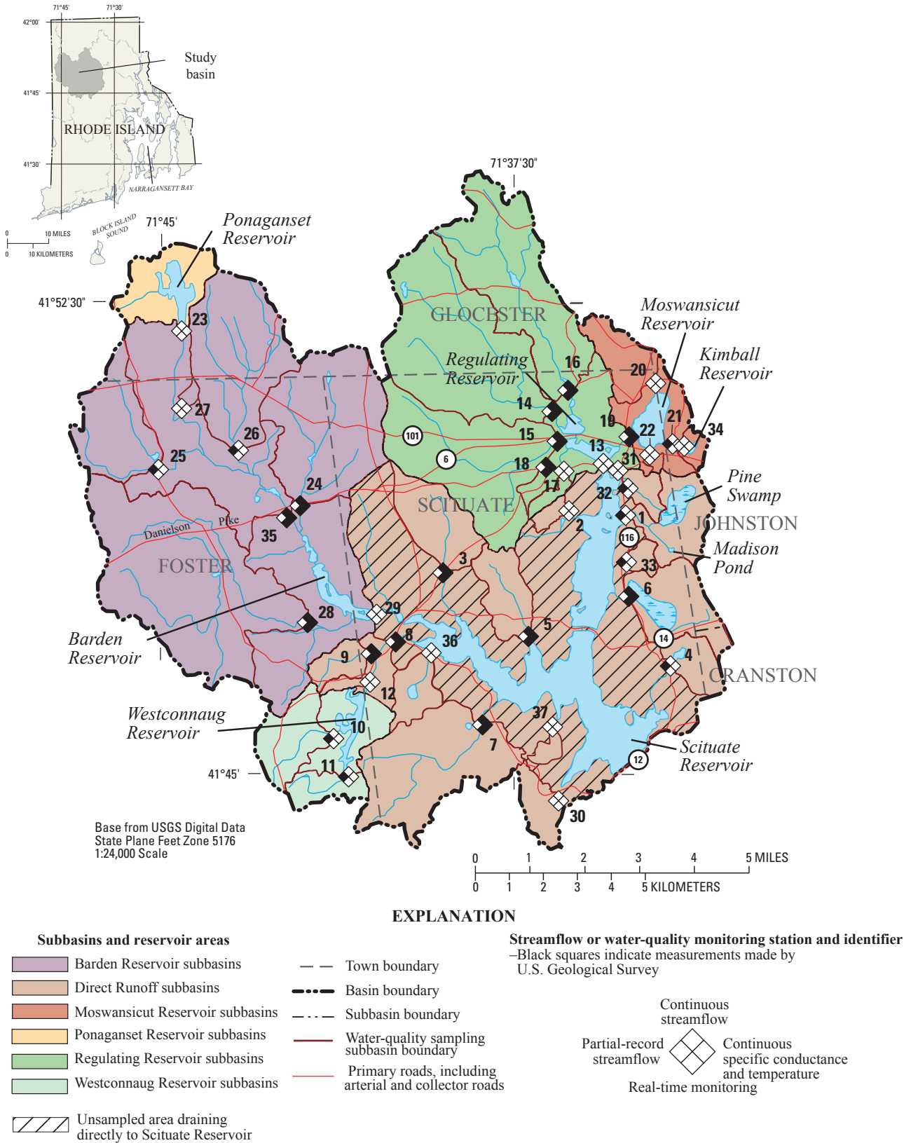
Figure 1. Locations of tributary-reservoir subbasins and streamgauge and water-quality monitoring stations in the Scituate Reservoir drainage area, Rhode Island.
