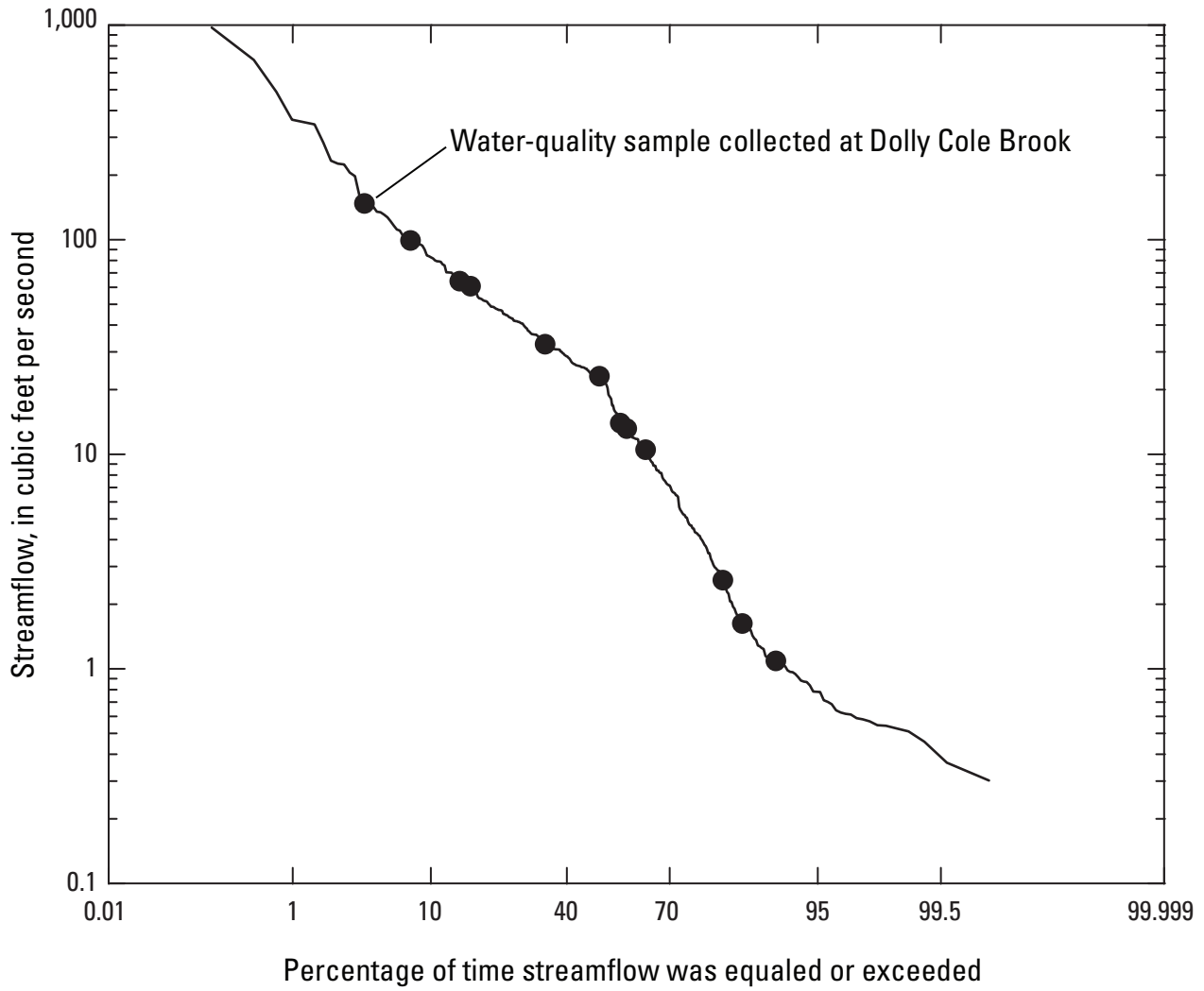
Figure 2. Flow-duration curve for the U.S. Geological Survey continuous streamgage on Ponaganset River at South Foster (streamgage 01115187) for water year 2010 and streamflow measurements at the Ponaganset River streamgage on the dates when water-quality samples were collected at Dolly Cole Brook (shown as points).
