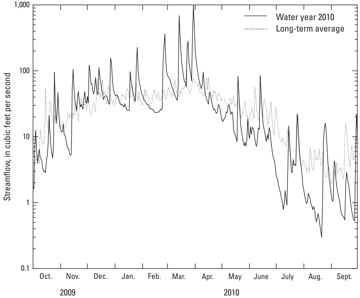
Figure 3. Measured daily mean streamflow for the U.S. Geological Survey continuous-record streamgage on the Ponaganset River at South Foster (streamgage 01115187) in the Scituate Reservoir drainage area, Rhode Island, for October 1, 2009, through September 30, 2010, and mean daily streamflow for March 22, 1994, through June 3, 2009.
