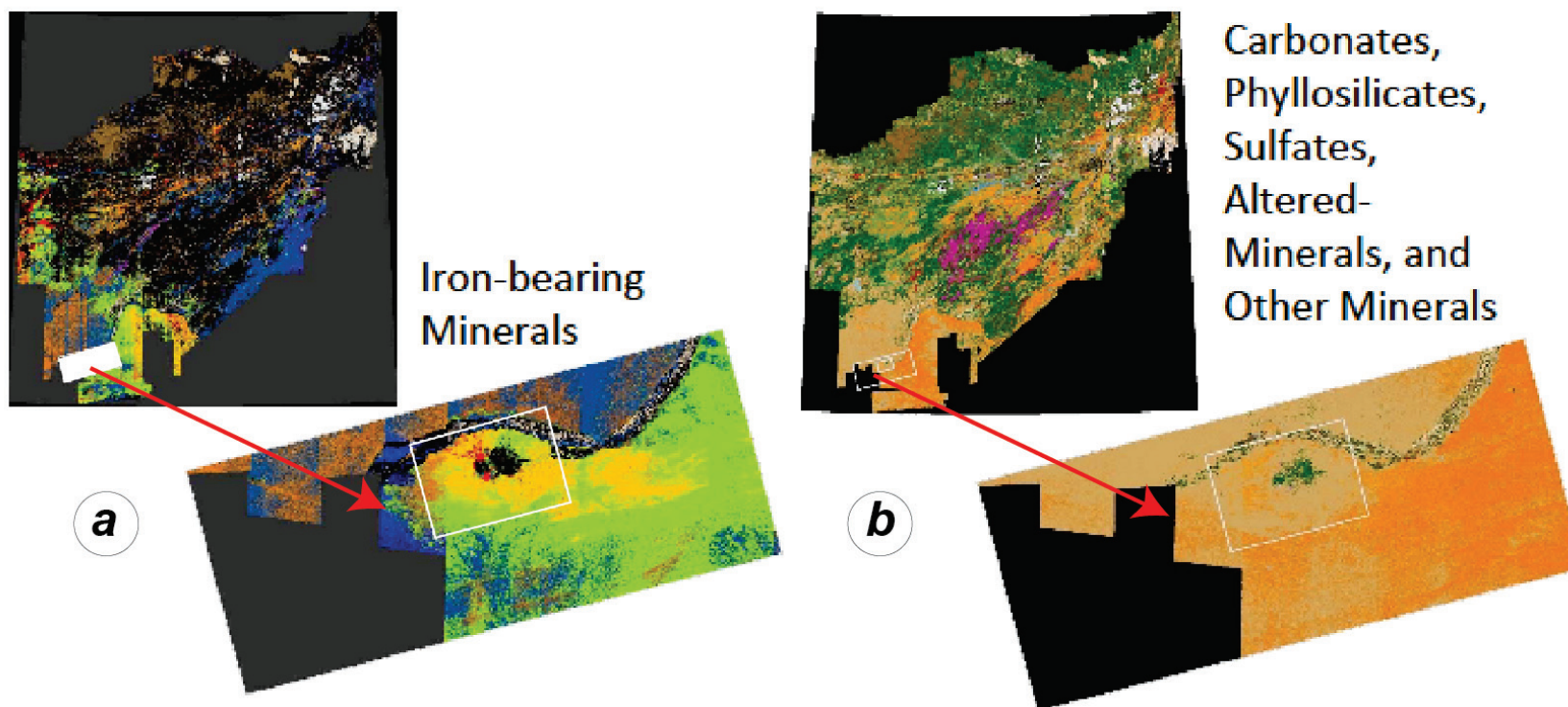
Figure 1-18. Examples of hyperspectral mapping at the Khanneshin carbonatite area of interest showing both (a) iron-bearing and (b) carbonate-phylllosilicate presentations. Images of these data are included in the data packages for each area of interest and are available for download at http://afghanistan.cr.usgs.gov/ and from the AGS Data Center in Kabul ( http://mom.gov.af/en ; http://www.bgs.ac.uk/afghanminerals/ ).
