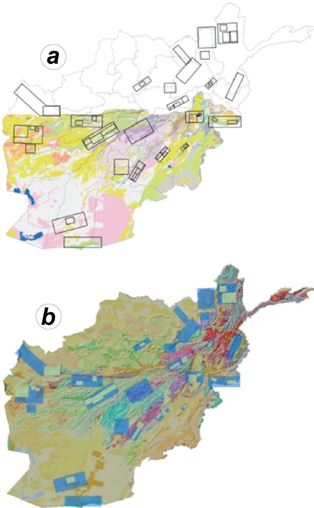
Figure1–6. Maps showing an example of different datasets overlaying different areas of interest. All areas of interest do not contain the same data. (a) German geologic data cover only the southern part of Afghanistan. (b) Russian geologic data are available for all of Afghanistan (Doebrich and others, 2006).
