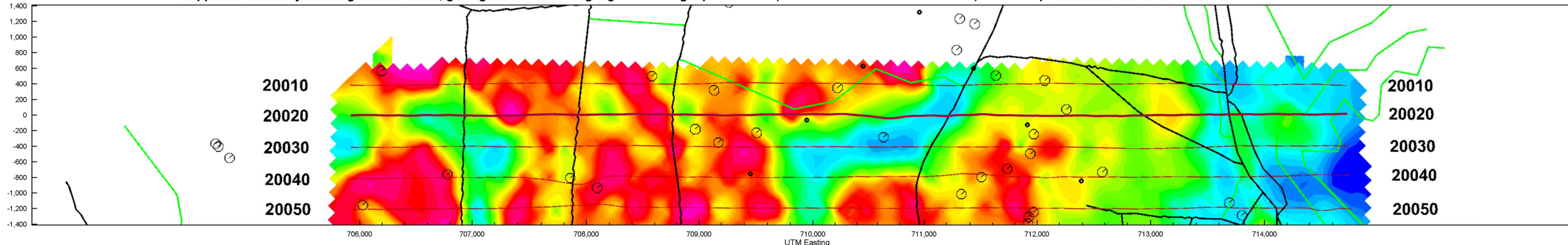
Line L20020 >>> 100 kHz apparent resistivity showing faults in black, geological contacts in light green and flight paths in red (thicker line shows middle section). Track map oriented in SW-NE direction.
