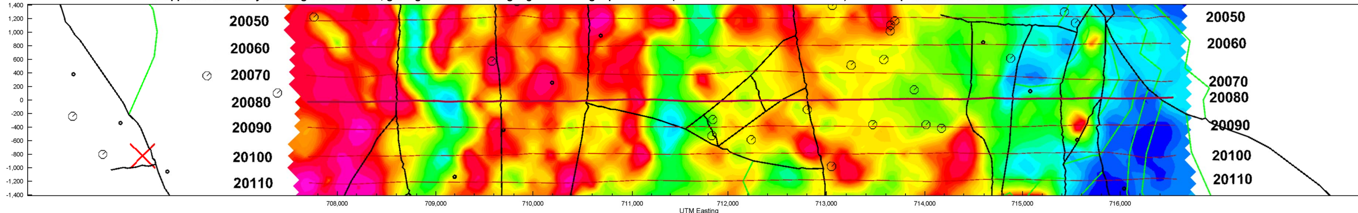
Line L20080 >>> 100 kHz apparent resistivity showing faults in black, geological contacts in light green and flight paths in red (thicker line shows middle section). Track map oriented in SW-NE direction.
