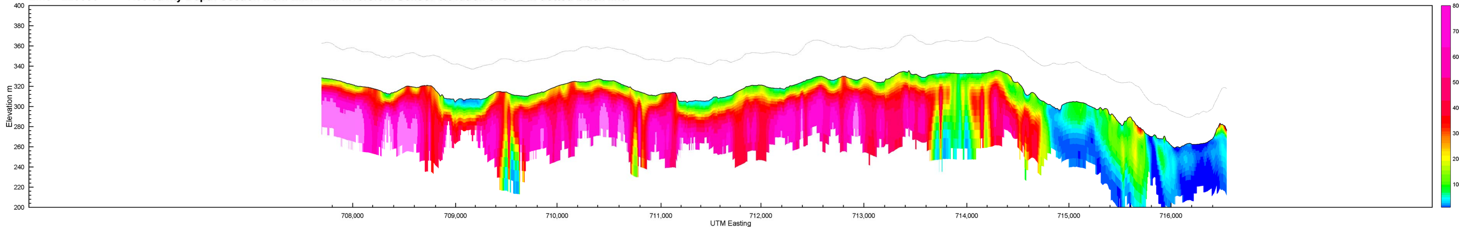
Line L20080 >>> Resistivity Depth Section from EM1DFM inversion. Sensor elevation shown in dotted black line.
