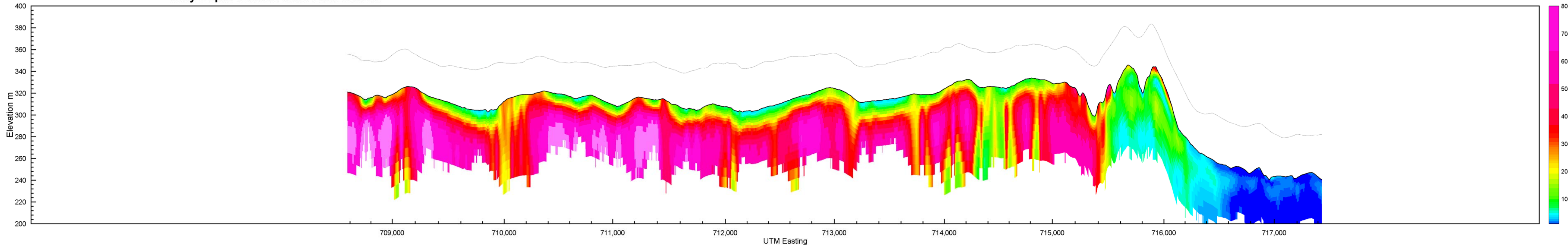
Line L20120 >>> Resistivity Depth Section from EM1DFM inversion. Sensor elevation shown in dotted black line.
