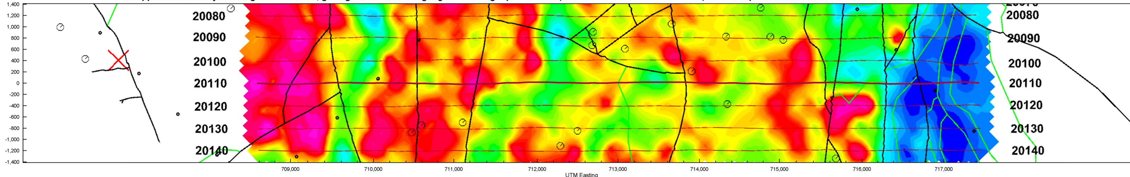
Line L20110 <<< 100 kHz apparent resistivity showing faults in black, geological contacts in light green and flight paths in red (thicker line shows middle section). Track map oriented in SW-NE direction.
