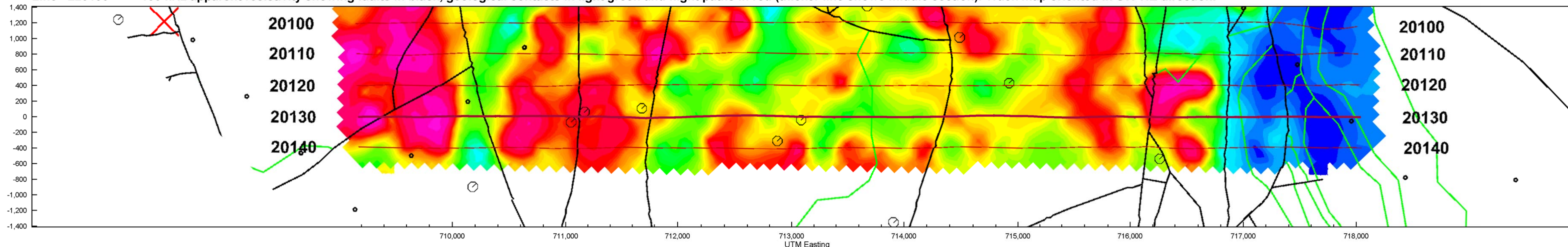
Line L20130 <<< 100 kHz apparent resistivity showing faults in black, geological contacts in light green and flight paths in red (thicker line shows middle section). Track map oriented in SW-NE direction.
