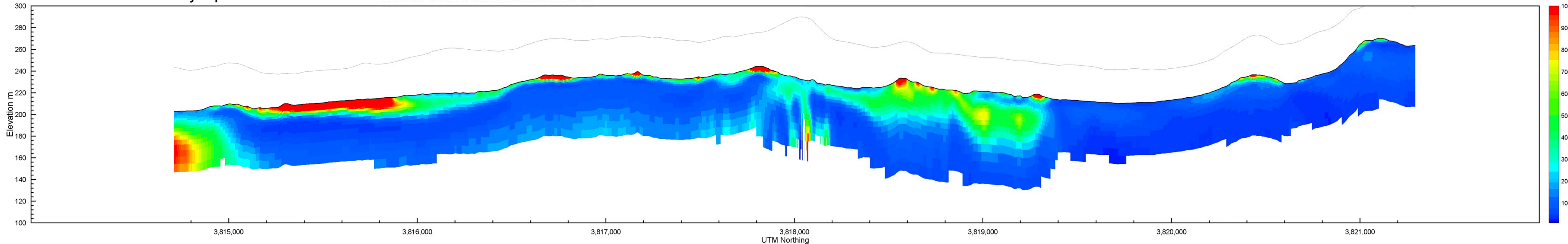
Line L30030 <<< Resistivity Depth Section from EM1DFM inversion. Sensor elevation shown in dotted black line.
