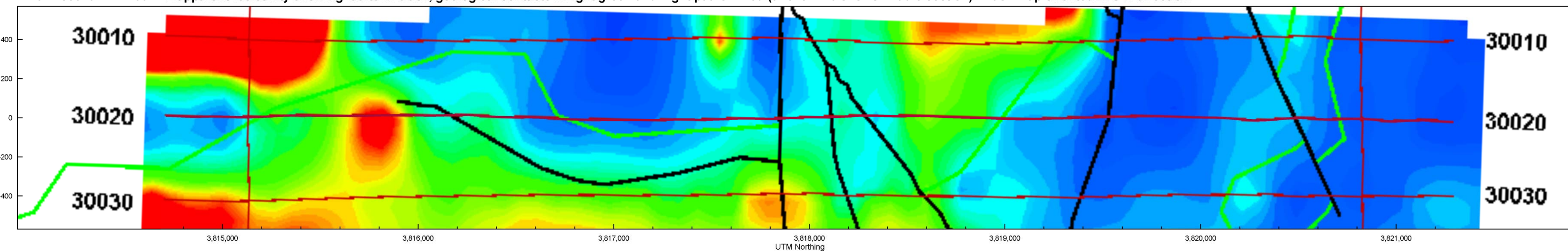
Line L30020 >>> 100 kHz apparent resistivity showing faults in black, geological contacts in light green and flight paths in red (thicker line shows middle section). Track map oriented in S-N direction.
