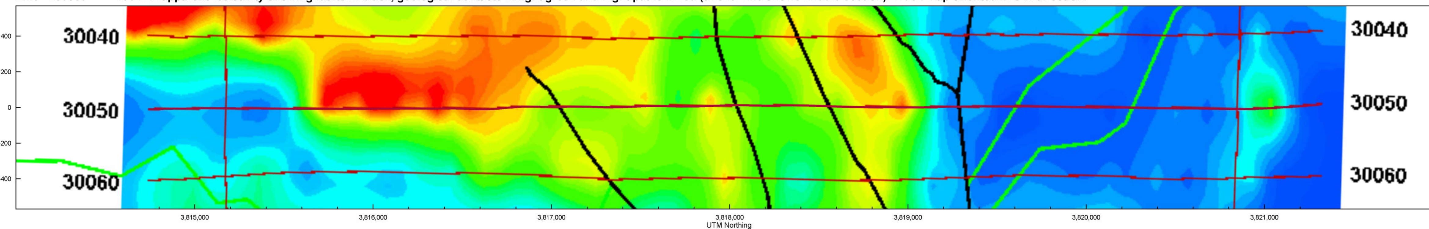
Line L30050 <<< 100 kHz apparent resistivity showing faults in black, geological contacts in light green and flight paths in red (thicker line shows middle section). Track map oriented in S-N direction.
