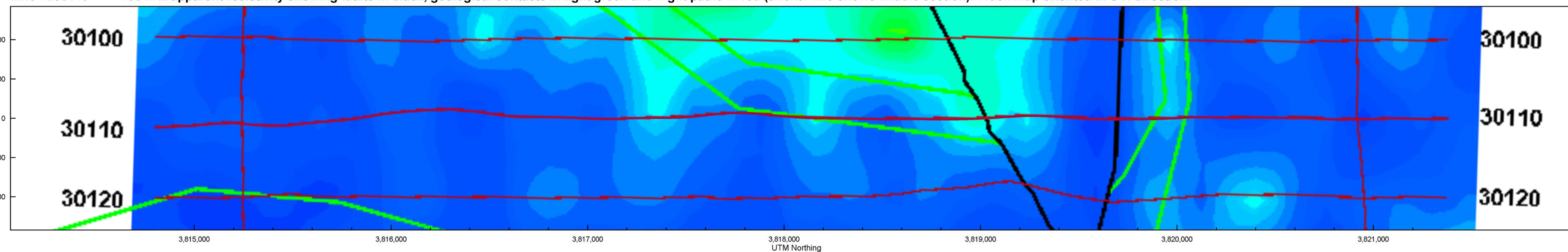
Line L30110 <<< 100 kHz apparent resistivity showing faults in black, geological contacts in light green and flight paths in red (thicker line shows middle section). Track map oriented in S-N direction.
