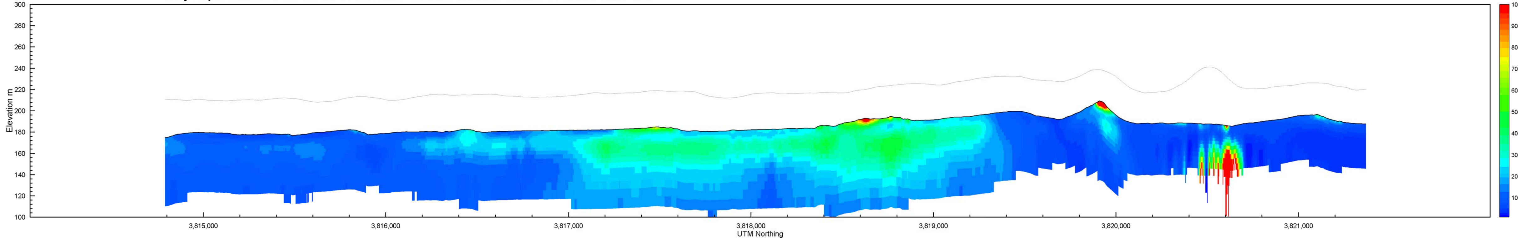
Line L30110 <<< Resistivity Depth Section from EM1DFM inversion. Sensor elevation shown in dotted black line.
