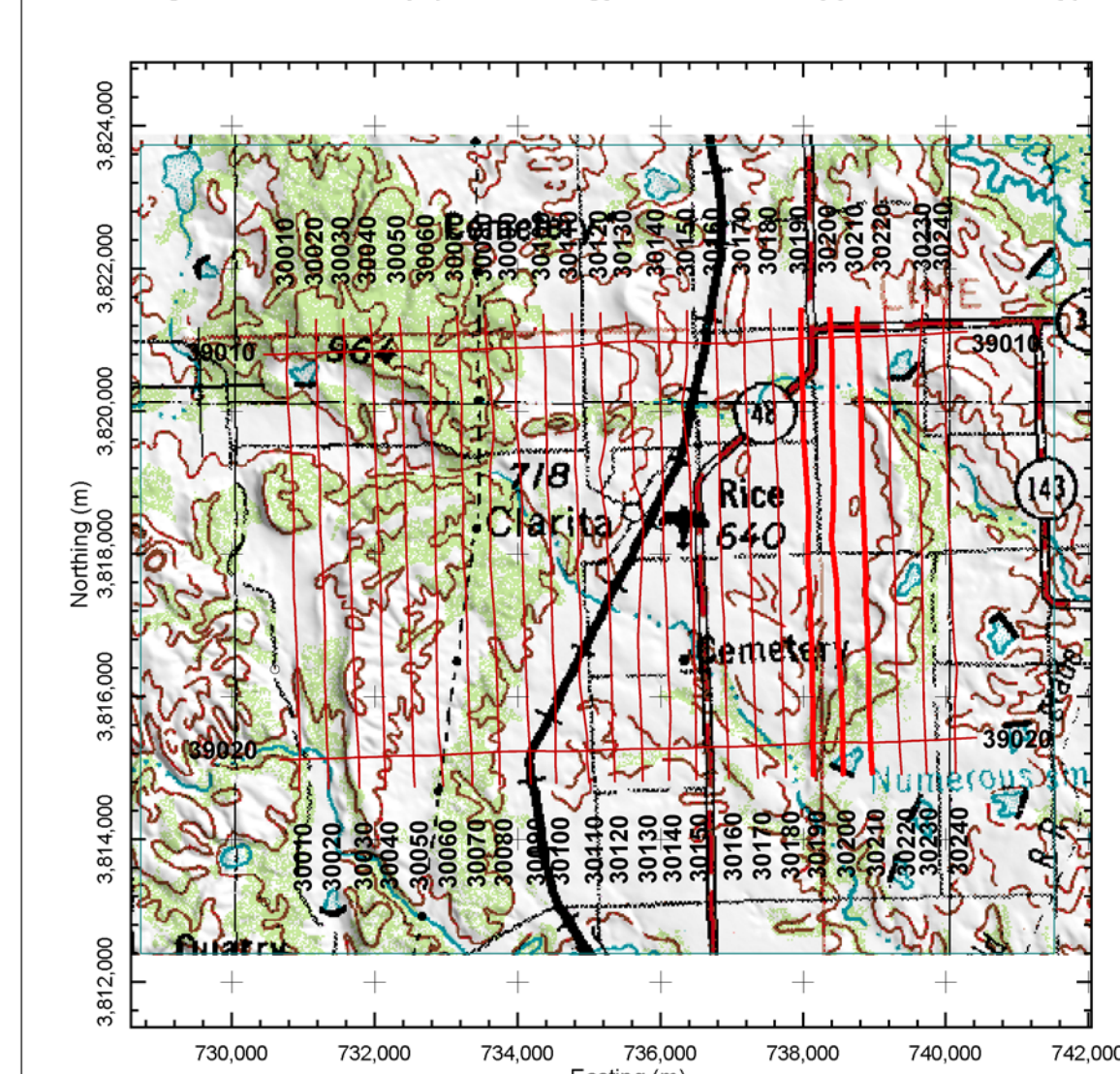
Flight Line Index Map (with Geology and 100 kHz Apparent Resistivity).
