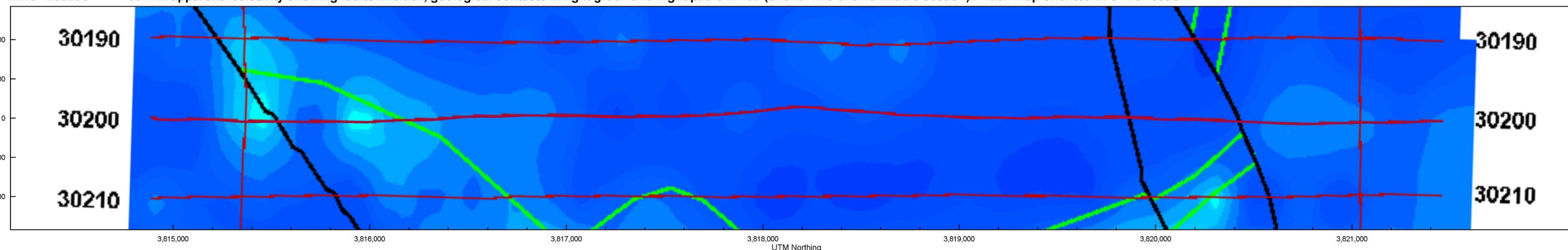
Line L30200 >>> 100 kHz apparent resistivity showing faults in black, geological contacts in light green and flight paths in red (thicker line shows middle section). Track map oriented in S-N direction.
