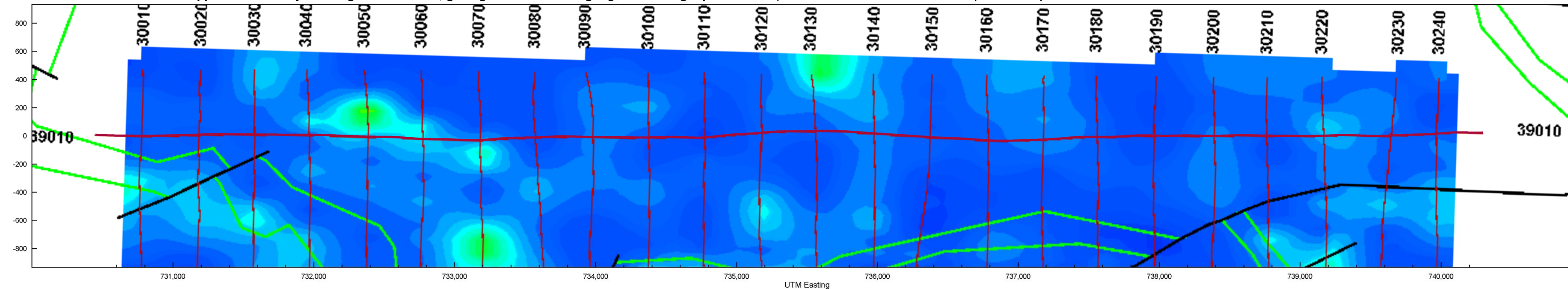
Line L39010 <<< 100 kHz apparent resistivity showing faults in black, geological contacts in light green and flight paths in red (thicker line shows middle section). Track map oriented in E-W direction.
