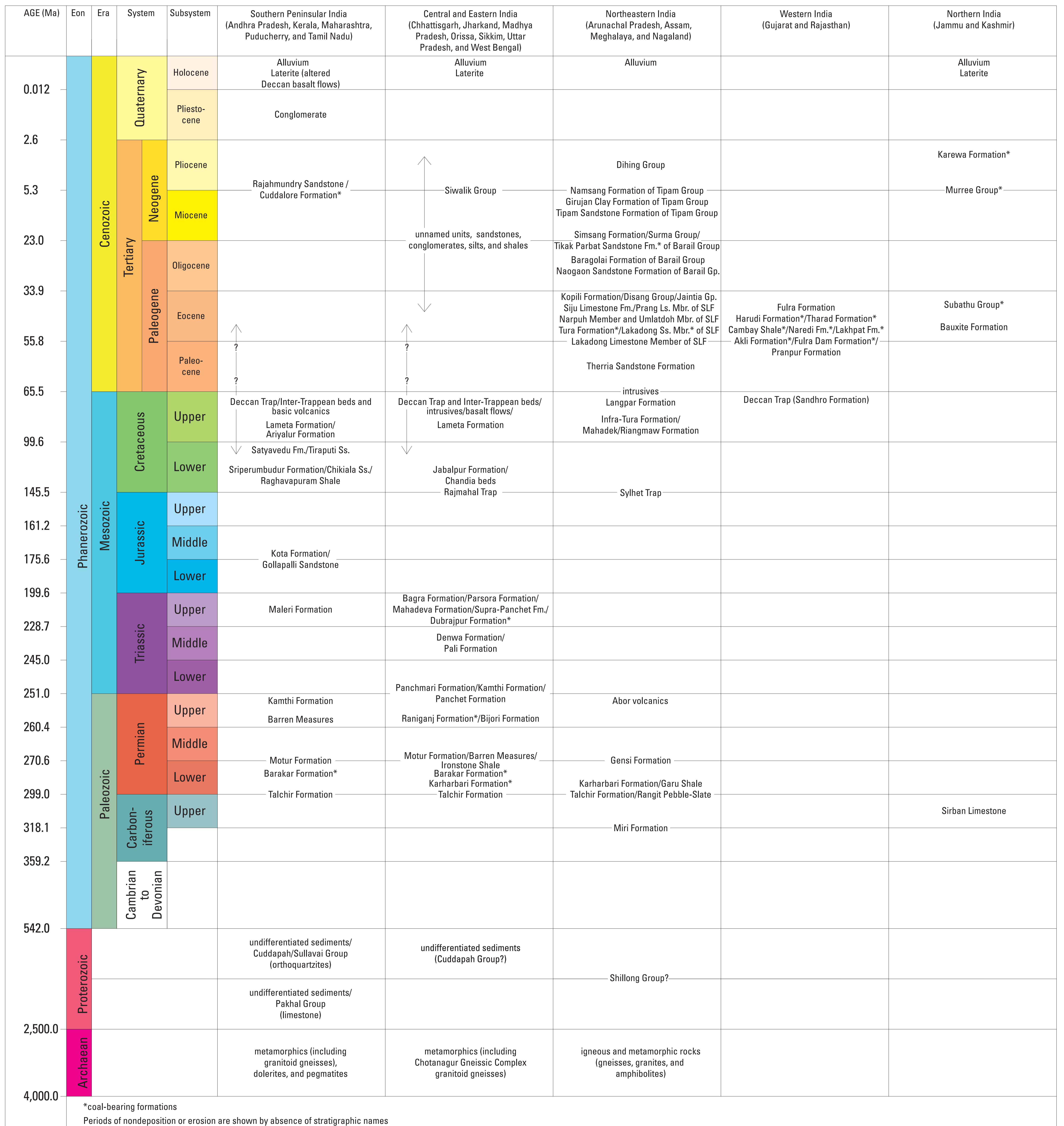
Figure 2. Correlation chart of stratigraphic units in coalfields of India
