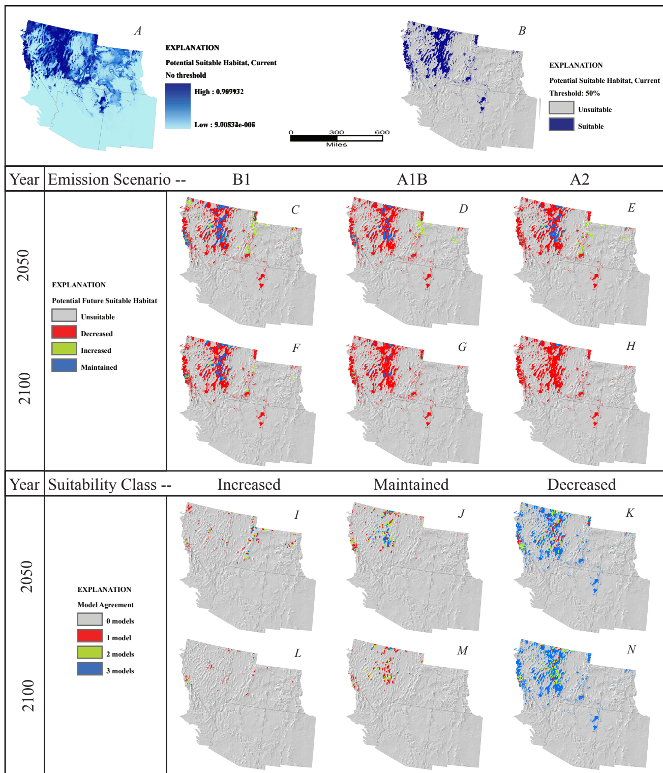
Figure 47. Artemisia arbuscula . A, Potential suitable habitat for species based on average annual and monthly precipitation and temperature from 1971 to 2000, continuous model output with no threshold. B, Potential suitable habitat, binary output using .5 threshold. C-E, Potential suitable habitat predicted by year 2050 under emission scenario (C), B1, (D), A1B, (E), A2. F-H, Potential suitable habitat predicted by year 2100 under emission scenario (F), B1, (G), A1B, (H), A2. I-K, Number of 2050 emission scenario models predicting each suitability class, (I), increased suitability, (J), maintained suitability, (K), decreased suitability. L-N, Number of 2100 emission scenario models predicting each suitability class, (L), increased suitability, (M), maintained suitability, and (N), decreased suitability.
