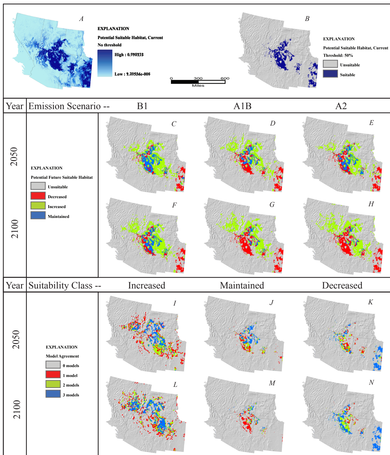
Figure 49. Artemisia filifolia . A, Potential suitable habitat for species based on average annual and monthly precipitation and temperature from 1971 to 2000, continuous model output with no threshold. B, Potential suitable habitat, binary output using .5 threshold. C-E, Potential suitable habitat predicted by year 2050 under emission scenario (C), B1, (D), A1B, (E), A2. F-H, Potential suitable habitat predicted by year 2100 under emission scenario (F), B1, (G), A1B, (H), A2. I-K, Number of 2050 emission scenario models predicting each suitability class, (I), increased suitability, (J), maintained suitability, (K), decreased suitability. L-N, Number of 2100 emission scenario models predicting each suitability class, (L), increased suitability, (M), maintained suitability, and (N), decreased suitability.
