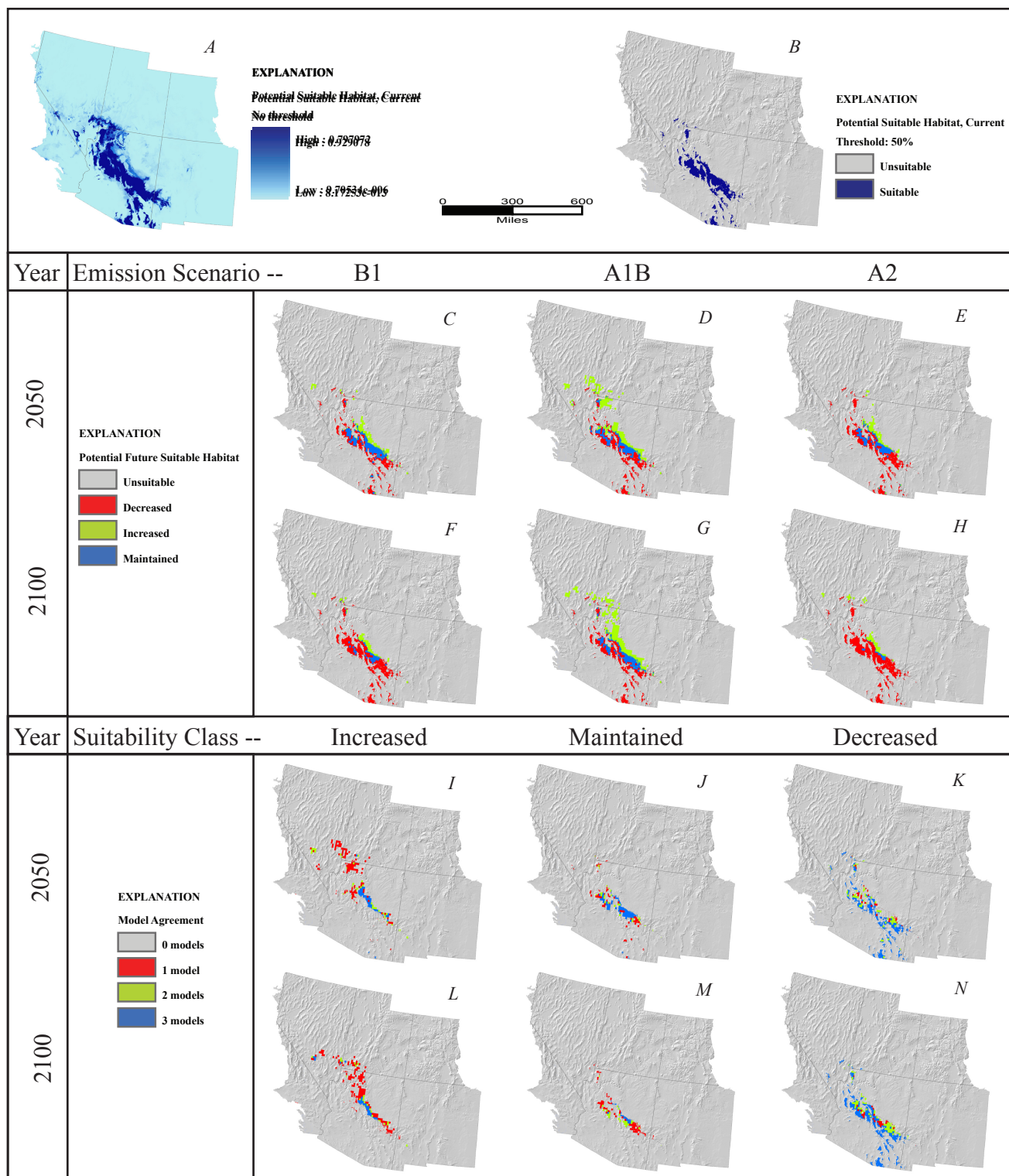
Figure 45. Arctostaphylos pungens . A, Potential suitable habitat for species based on average annual and monthly precipitation and temperature from 1971 to 2000, continuous model output with no threshold. B, Potential suitable habitat, binary output using .5 threshold. C-E, Potential suitable habitat predicted by year 2050 under emission scenario (C), B1, (D), A1B, (E), A2. F-H, Potential suitable habitat predicted by year 2100 under emission scenario (F), B1, (G), A1B, (H), A2. I-K, Number of 2050 emission scenario models predicting each suitability class, (I), increased suitability, (J), maintained suitability, (K), decreased suitability. L-N, Number of 2100 emission scenario models predicting each suitability class, (L), increased suitability, (M), maintained suitability, and (N), decreased suitability.
