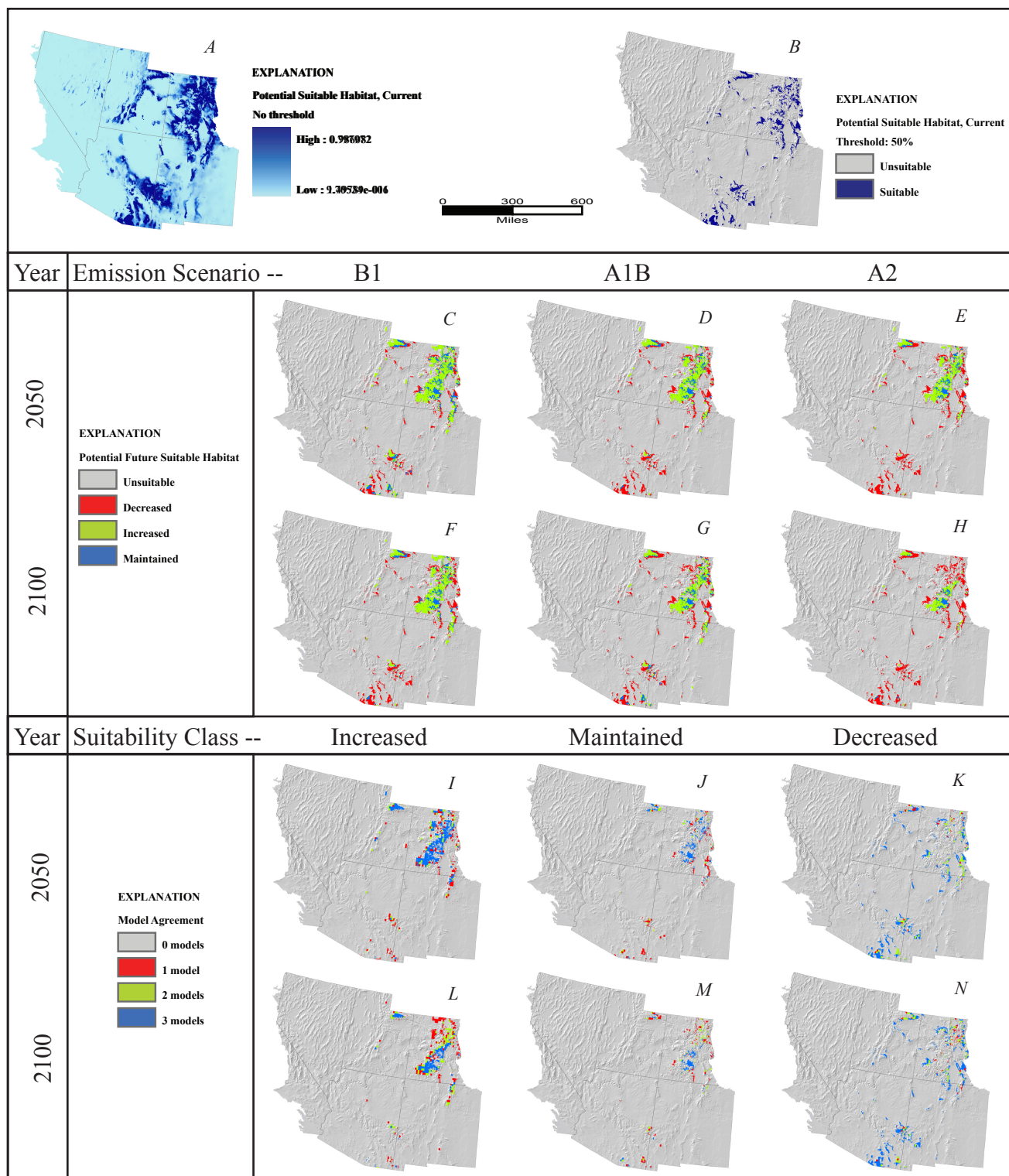
Figure 46. Arctostaphylos uva-ursi . A, Potential suitable habitat for species based on average annual and monthly precipitation and temperature from 1971 to 2000, continuous model output with no threshold. B, Potential suitable habitat, binary output using .5 threshold. C-E, Potential suitable habitat predicted by year 2050 under emission scenario (C), B1, (D), A1B, (E), A2. F-H, Potential suitable habitat predicted by year 2100 under emission scenario (F), B1, (G), A1B, (H), A2. I-K, Number of 2050 emission scenario models predicting each suitability class, (I), increased suitability, (J), maintained suitability, (K), decreased suitability. L-N, Number of 2100 emission scenario models predicting each suitability class, (L), increased suitability, (M), maintained suitability, and (N), decreased suitability.
