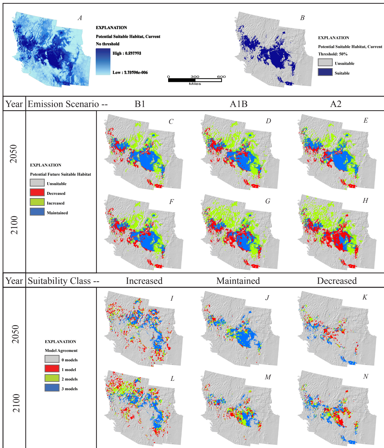
Figure 53. Atriplex canescens . A, Potential suitable habitat for species based on average annual and monthly precipitation and temperature from 1971 to 2000, continuous model output with no threshold. B, Potential suitable habitat, binary output using .5 threshold. C-E, Potential suitable habitat predicted by year 2050 under emission scenario (C), B1, (D), A1B, (E), A2. F-H, Potential suitable habitat predicted by year 2100 under emission scenario (F), B1, (G), A1B, (H), A2. I-K, Number of 2050 emission scenario models predicting each suitability class, (I), increased suitability, (J), maintained suitability, (K), decreased suitability. L-N, Number of 2100 emission scenario models predicting each suitability class, (L), increased suitability, (M), maintained suitability, and (N), decreased suitability.
