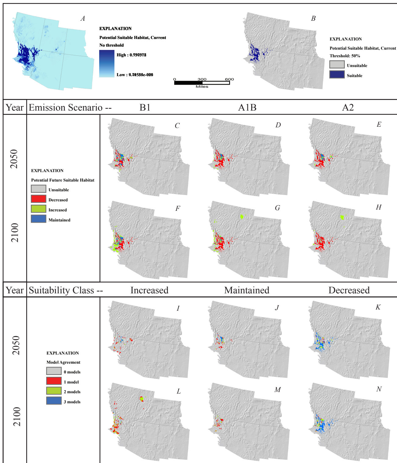
Figure 57. Atriplex hymenelytra . A, Potential suitable habitat for species based on average annual and monthly precipitation and temperature from 1971 to 2000, continuous model output with no threshold. B, Potential suitable habitat, binary output using .5 threshold. C-E, Potential suitable habitat predicted by year 2050 under emission scenario (C), B1, (D), A1B, (E), A2. F-H, Potential suitable habitat predicted by year 2100 under emission scenario (F), B1, (G), A1B, (H), A2. I-K, Number of 2050 emission scenario models predicting each suitability class, (I), increased suitability, (J), maintained suitability, (K), decreased suitability. L-N, Number of 2100 emission scenario models predicting each suitability class, (L), increased suitability, (M), maintained suitability, and (N), decreased suitability.
