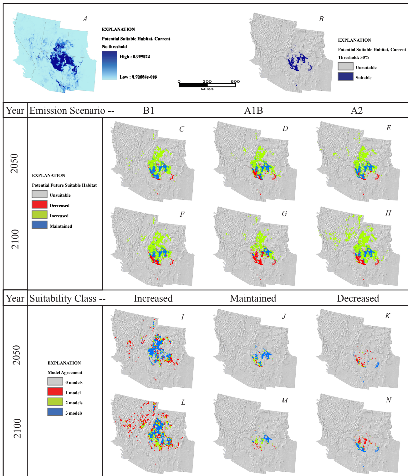
Figure 58. Atriplex obovata . A, Potential suitable habitat for species based on average annual and monthly precipitation and temperature from 1971 to 2000, continuous model output with no threshold. B, Potential suitable habitat, binary output using .5 threshold. C-E, Potential suitable habitat predicted by year 2050 under emission scenario (C), B1, (D), A1B, (E), A2. F-H, Potential suitable habitat predicted by year 2100 under emission scenario (F), B1, (G), A1B, (H), A2. I-K, Number of 2050 emission scenario models predicting each suitability class, (I), increased suitability, (J), maintained suitability, (K), decreased suitability. L-N, Number of 2100 emission scenario models predicting each suitability class, (L), increased suitability, (M), maintained suitability, and (N), decreased suitability.
