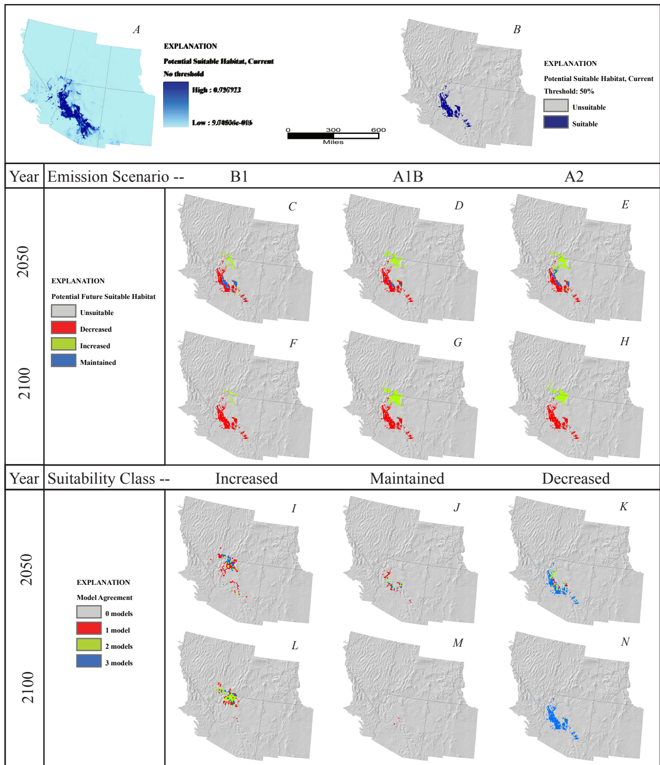
Figure 61. Canotia holacantha . A, Potential suitable habitat for species based on average annual and monthly precipitation and temperature from 1971 to 2000, continuous model output with no threshold. B, Potential suitable habitat, binary output using .5 threshold. C-E, Potential suitable habitat predicted by year 2050 under emission scenario (C), B1, (D), A1B, (E), A2. F-H, Potential suitable habitat predicted by year 2100 under emission scenario (F), B1, (G), A1B, (H), A2. I-K, Number of 2050 emission scenario models predicting each suitability class, (I), increased suitability, (J), maintained suitability, (K), decreased suitability. L-N, Number of 2100 emission scenario models predicting each suitability class, (L), increased suitability, (M), maintained suitability, and (N), decreased suitability.
