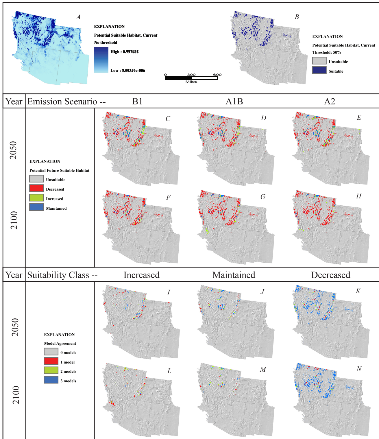
Figure 64. Cercocarpus ledifolius . A, Potential suitable habitat for species based on average annual and monthly precipitation and temperature from 1971 to 2000, continuous model output with no threshold. B, Potential suitable habitat, binary output using .5 threshold. C-E, Potential suitable habitat predicted by year 2050 under emission scenario (C), B1, (D), A1B, (E), A2. F-H, Potential suitable habitat predicted by year 2100 under emission scenario (F), B1, (G), A1B, (H), A2. I-K, Number of 2050 emission scenario models predicting each suitability class, (I), increased suitability, (J), maintained suitability, (K), decreased suitability. L-N, Number of 2100 emission scenario models predicting each suitability class, (L), increased suitability, (M), maintained suitability, and (N), decreased suitability.
