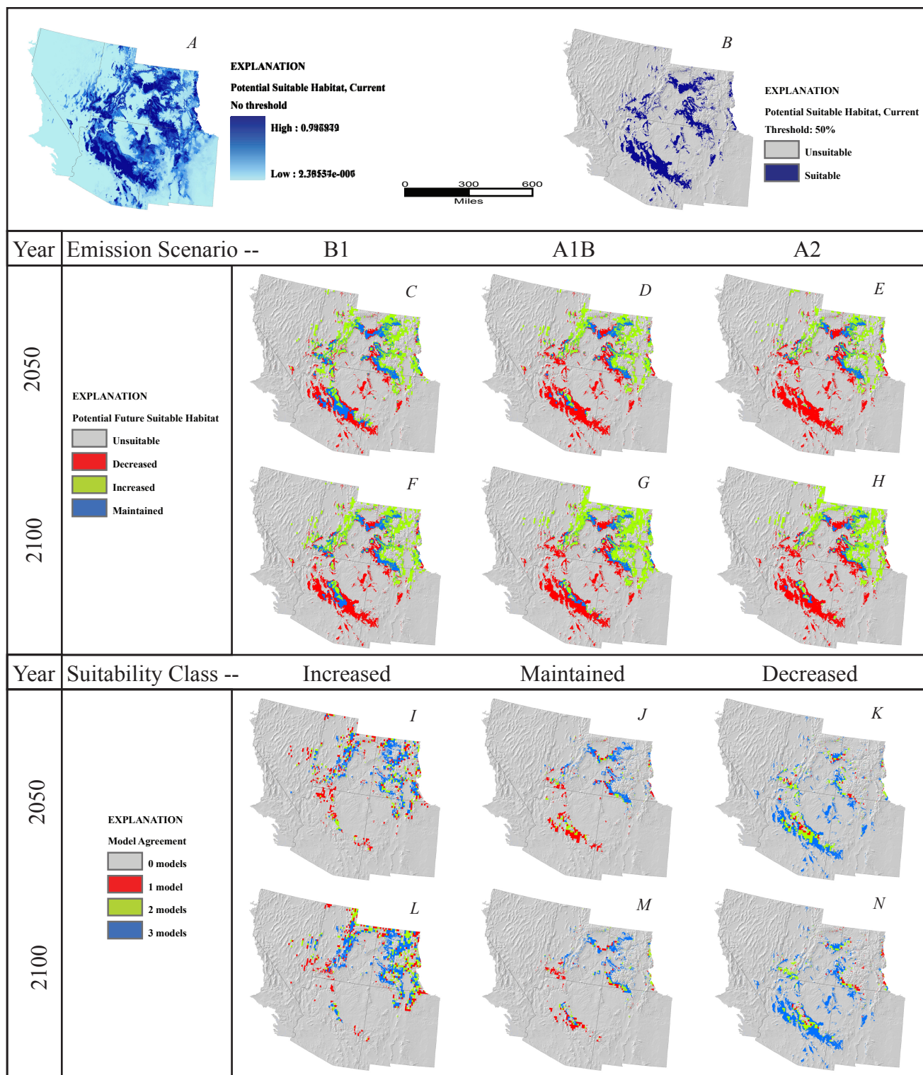
Figure 65. Cercocarpus montanus . A, Potential suitable habitat for species based on average annual and monthly precipitation and temperature from 1971 to 2000, continuous model output with no threshold. B, Potential suitable habitat, binary output using .5 threshold. C-E, Potential suitable habitat predicted by year 2050 under emission scenario (C), B1, (D), A1B, (E), A2. F-H, Potential suitable habitat predicted by year 2100 under emission scenario (F), B1, (G), A1B, (H), A2. I-K, Number of 2050 emission scenario models predicting each suitability class, (I), increased suitability, (J), maintained suitability, (K), decreased suitability. L-N, Number of 2100 emission scenario models predicting each suitability class, (L), increased suitability, (M), maintained suitability, and (N), decreased suitability.
