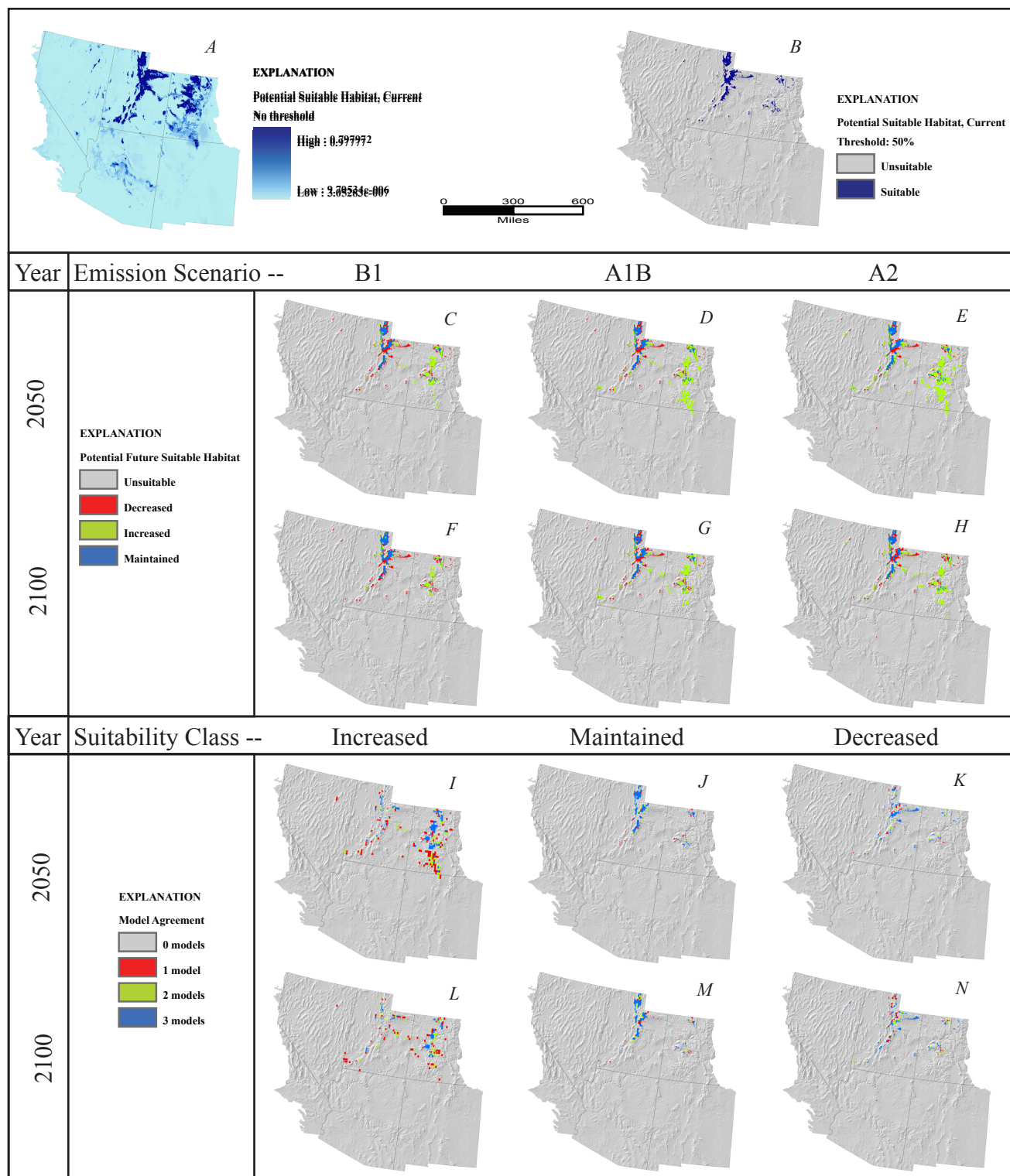
Figure 143. Elymus glaucus . A, Potential suitable habitat for species based on average annual and monthly precipitation and temperature from 1971 to 2000, continuous model output with no threshold. B, Potential suitable habitat, binary output using .5 threshold. C-E, Potential suitable habitat predicted by year 2050 under emission scenario (C), B1, (D), A1B, (E), A2. F-H, Potential suitable habitat predicted by year 2100 under emission scenario (F), B1, (G), A1B, (H), A2. I-K, Number of 2050 emission scenario models predicting each suitability class, (I), increased suitability, (J), maintained suitability, (K), decreased suitability. L-N, Number of 2100 emission scenario models predicting each suitability class, (L), increased suitability, (M), maintained suitability, and (N), decreased suitability.
