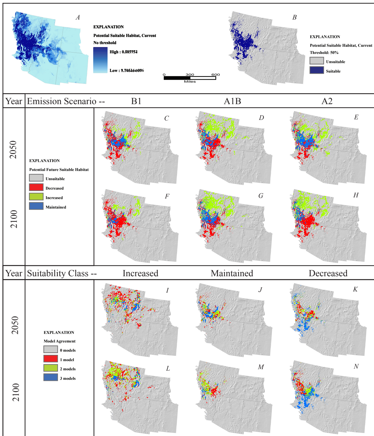
Figure 71. Ephedra nevadensis . A, Potential suitable habitat for species based on average annual and monthly precipitation and temperature from 1971 to 2000, continuous model output with no threshold. B, Potential suitable habitat, binary output using .5 threshold. C-E, Potential suitable habitat predicted by year 2050 under emission scenario (C), B1, (D), A1B, (E), A2. F-H, Potential suitable habitat predicted by year 2100 under emission scenario (F), B1, (G), A1B, (H), A2. I-K, Number of 2050 emission scenario models predicting each suitability class, (I), increased suitability, (J), maintained suitability, (K), decreased suitability. L-N, Number of 2100 emission scenario models predicting each suitability class, (L), increased suitability, (M), maintained suitability, and (N), decreased suitability.
