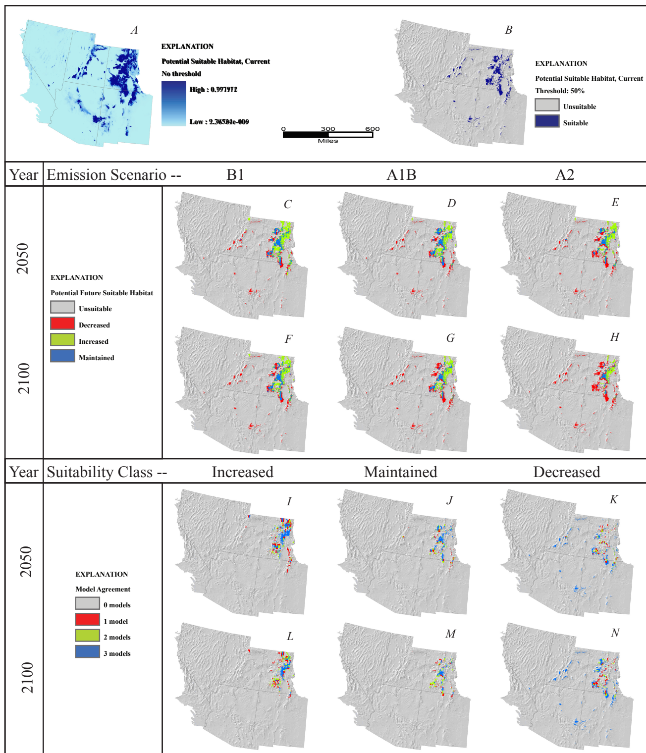
Figure 148. Festuca thurberi . A, Potential suitable habitat for species based on average annual and monthly precipitation and temperature from 1971 to 2000, continuous model output with no threshold. B, Potential suitable habitat, binary output using .5 threshold. C-E, Potential suitable habitat predicted by year 2050 under emission scenario (C), B1, (D), A1B, (E), A2. F-H, Potential suitable habitat predicted by year 2100 under emission scenario (F), B1, (G), A1B, (H), A2. I-K, Number of 2050 emission scenario models predicting each suitability class, (I), increased suitability, (J), maintained suitability, (K), decreased suitability. L-N, Number of 2100 emission scenario models predicting each suitability class, (L), increased suitability, (M), maintained suitability, and (N), decreased suitability.
