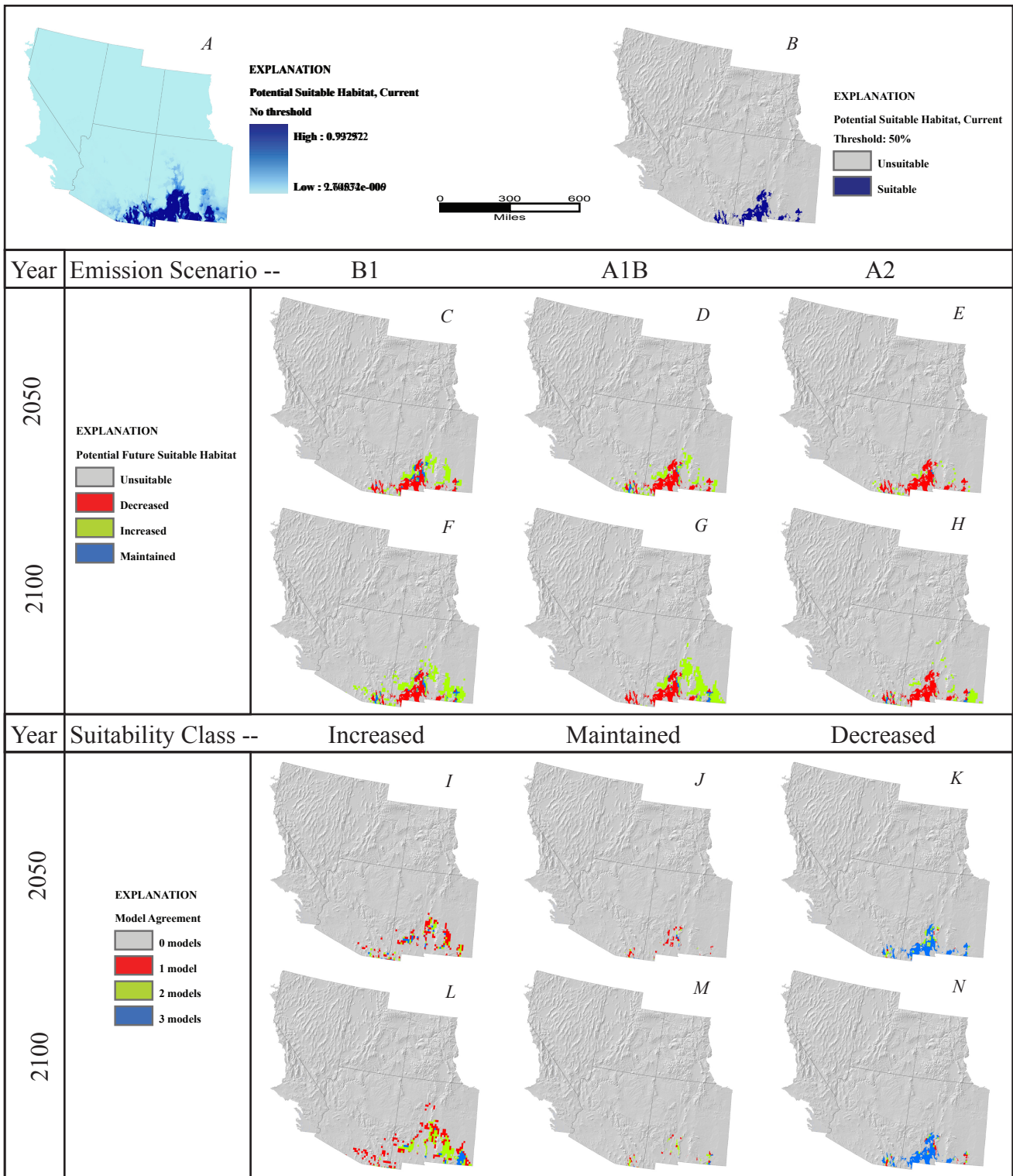
Figure 80. Flourensia cernua . A, Potential suitable habitat for species based on average annual and monthly precipitation and temperature from 1971 to 2000, continuous model output with no threshold. B, Potential suitable habitat, binary output using .5 threshold. C-E, Potential suitable habitat predicted by year 2050 under emission scenario (C), B1, (D), A1B, (E), A2. F-H, Potential suitable habitat predicted by year 2100 under emission scenario (F), B1, (G), A1B, (H), A2. I-K, Number of 2050 emission scenario models predicting each suitability class, (I), increased suitability, (J), maintained suitability, (K), decreased suitability. L-N, Number of 2100 emission scenario models predicting each suitability class, (L), increased suitability, (M), maintained suitability, and (N), decreased suitability.
