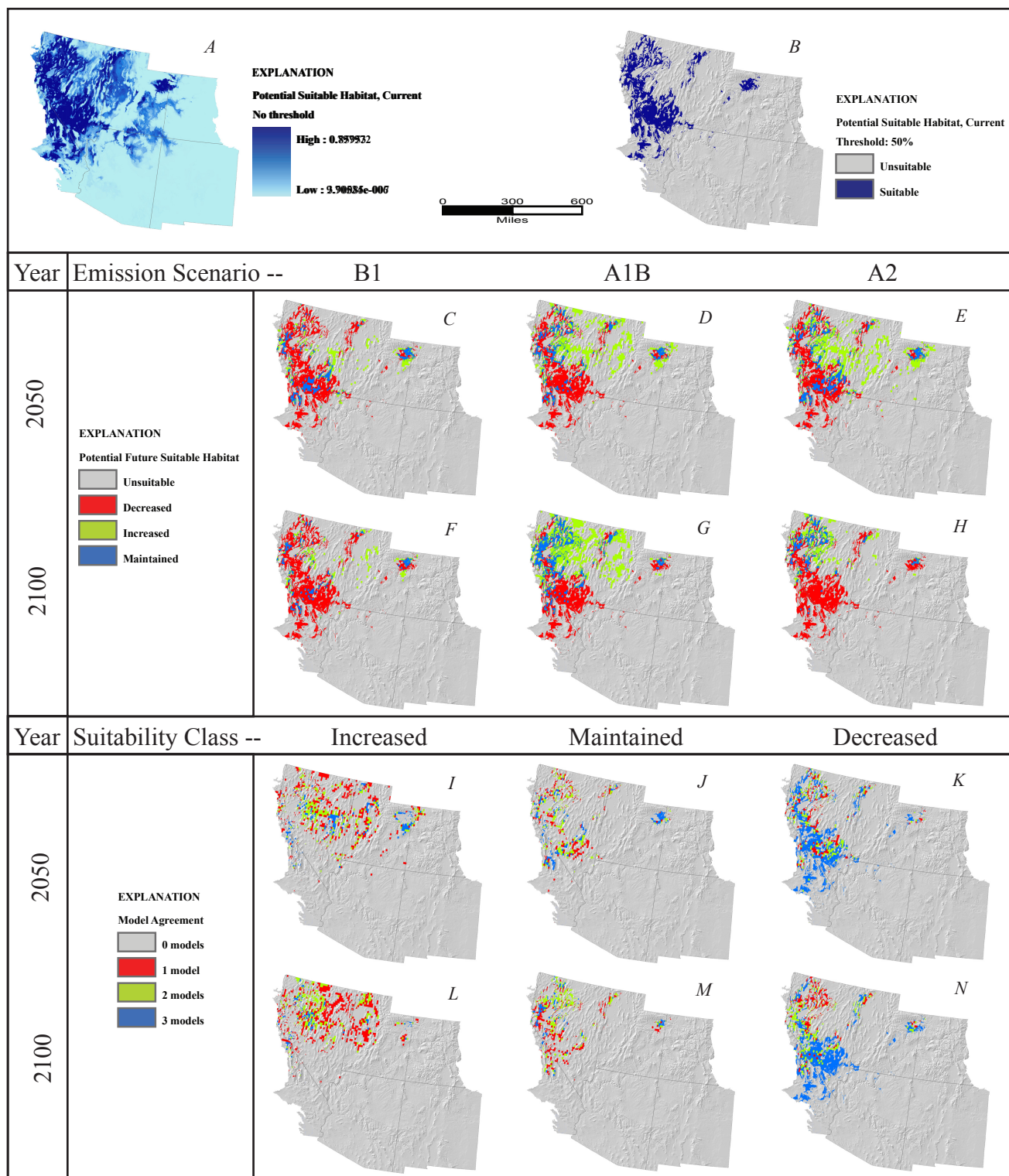
Figure 84. Grayia spinosa . A, Potential suitable habitat for species based on average annual and monthly precipitation and temperature from 1971 to 2000, continuous model output with no threshold. B, Potential suitable habitat, binary output using .5 threshold. C-E, Potential suitable habitat predicted by year 2050 under emission scenario (C), B1, (D), A1B, (E), A2. F-H, Potential suitable habitat predicted by year 2100 under emission scenario (F), B1, (G), A1B, (H), A2. I-K, Number of 2050 emission scenario models predicting each suitability class, (I), increased suitability, (J), maintained suitability, (K), decreased suitability. L-N, Number of 2100 emission scenario models predicting each suitability class, (L), increased suitability, (M), maintained suitability, and (N), decreased suitability.
