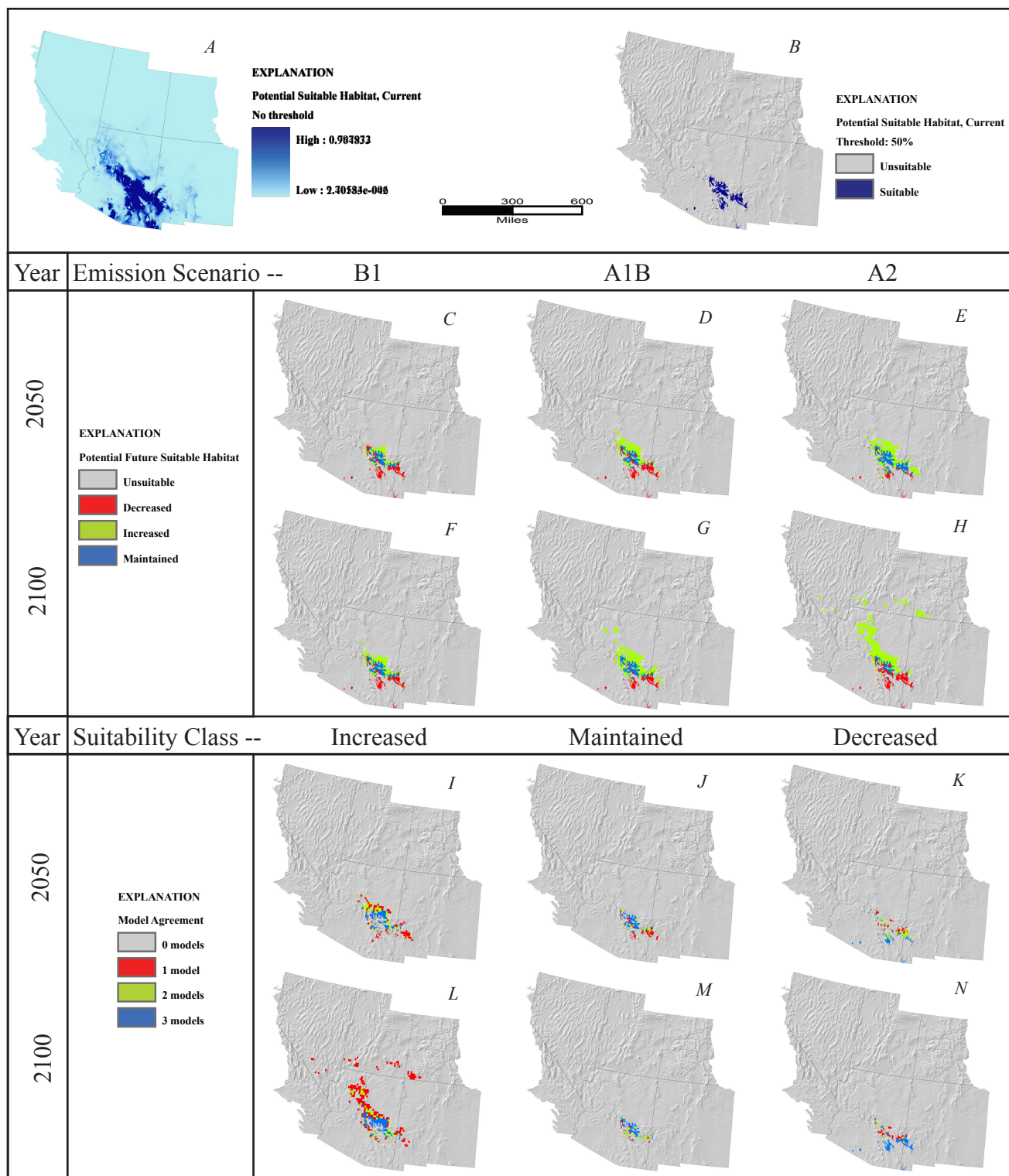
Figure 150. Hilaria belangeri . A, Potential suitable habitat for species based on average annual and monthly precipitation and temperature from 1971 to 2000, continuous model output with no threshold. B, Potential suitable habitat, binary output using .5 threshold. C-E, Potential suitable habitat predicted by year 2050 under emission scenario (C), B1, (D), A1B, (E), A2. F-H, Potential suitable habitat predicted by year 2100 under emission scenario (F), B1, (G), A1B, (H), A2. I-K, Number of 2050 emission scenario models predicting each suitability class, (I), increased suitability, (J), maintained suitability, (K), decreased suitability. L-N, Number of 2100 emission scenario models predicting each suitability class, (L), increased suitability, (M), maintained suitability, and (N), decreased suitability.
