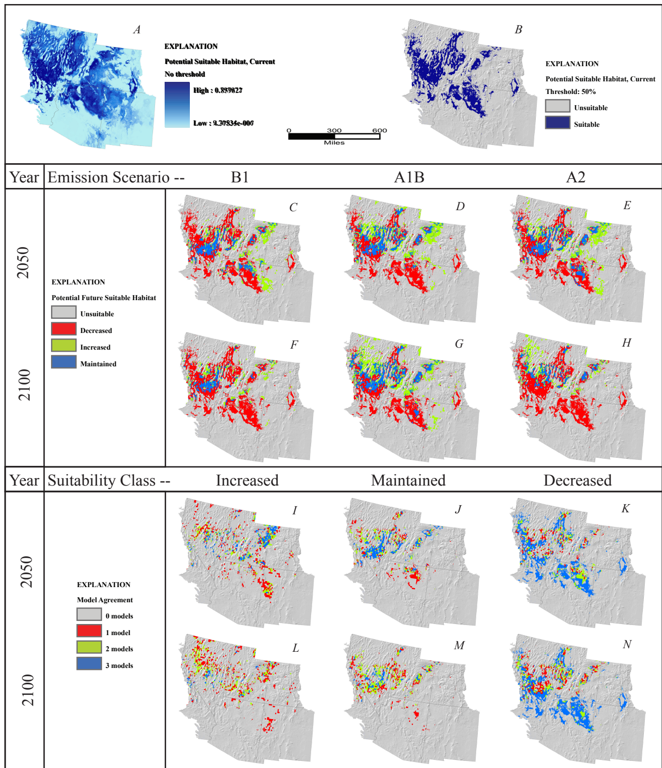
Figure 89. Krascheninnikovia lanata . A, Potential suitable habitat for species based on average annual and monthly precipitation and temperature from 1971 to 2000, continuous model output with no threshold. B, Potential suitable habitat, binary output using .5 threshold. C-E, Potential suitable habitat predicted by year 2050 under emission scenario (C), B1, (D), A1B, (E), A2. F-H, Potential suitable habitat predicted by year 2100 under emission scenario (F), B1, (G), A1B, (H), A2. I-K, Number of 2050 emission scenario models predicting each suitability class, (I), increased suitability, (J), maintained suitability, (K), decreased suitability. L-N, Number of 2100 emission scenario models predicting each suitability class, (L), increased suitability, (M), maintained suitability, and (N), decreased suitability.
