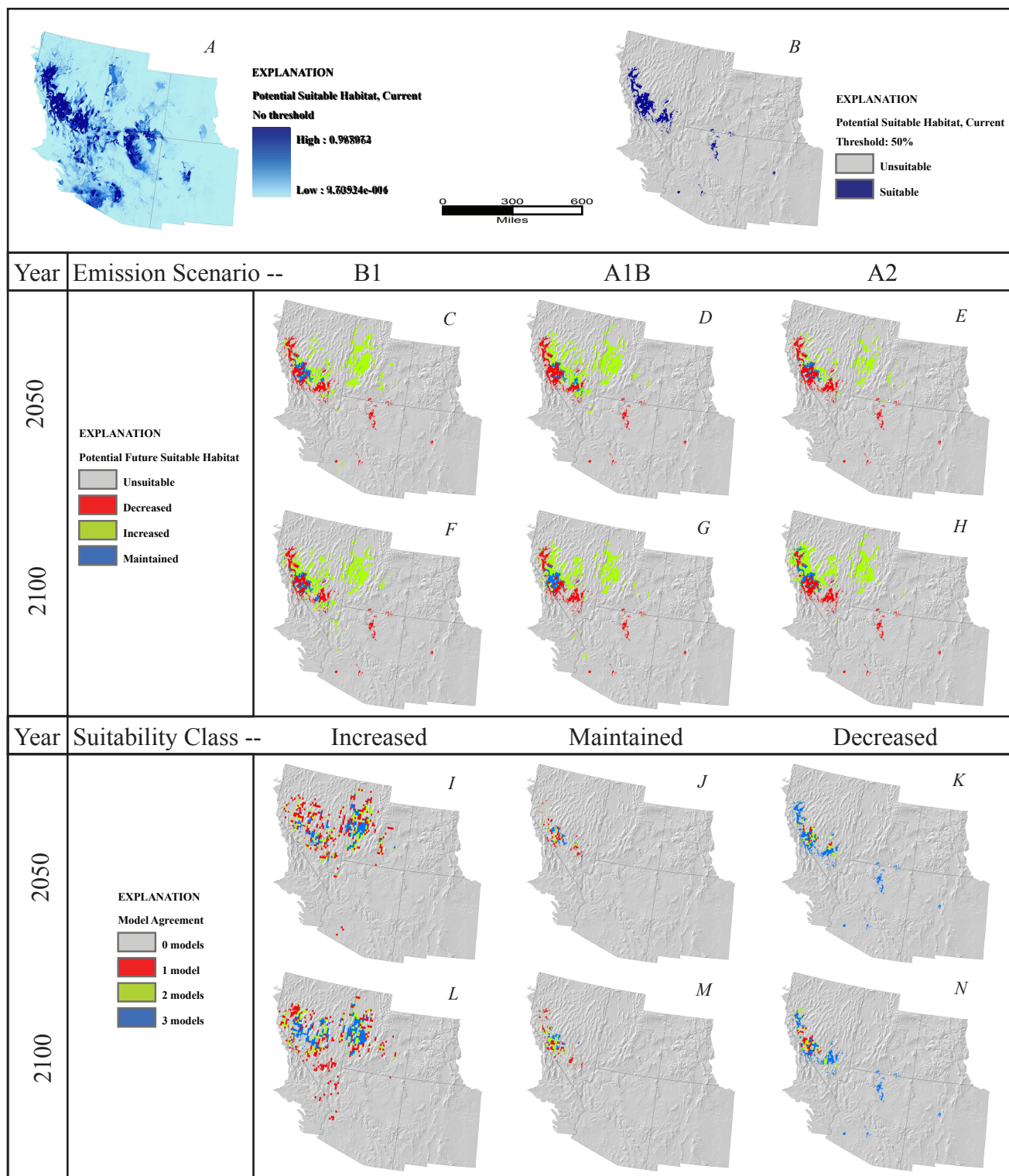
Figure 92. Lycium andersonii . A, Potential suitable habitat for species based on average annual and monthly precipitation and temperature from 1971 to 2000, continuous model output with no threshold. B, Potential suitable habitat, binary output using .5 threshold. C-E, Potential suitable habitat predicted by year 2050 under emission scenario (C), B1, (D), A1B, (E), A2. F-H, Potential suitable habitat predicted by year 2100 under emission scenario (F), B1, (G), A1B, (H), A2. I-K, Number of 2050 emission scenario models predicting each suitability class, (I), increased suitability, (J), maintained suitability, (K), decreased suitability. L-N, Number of 2100 emission scenario models predicting each suitability class, (L), increased suitability, (M), maintained suitability, and (N), decreased suitability.
