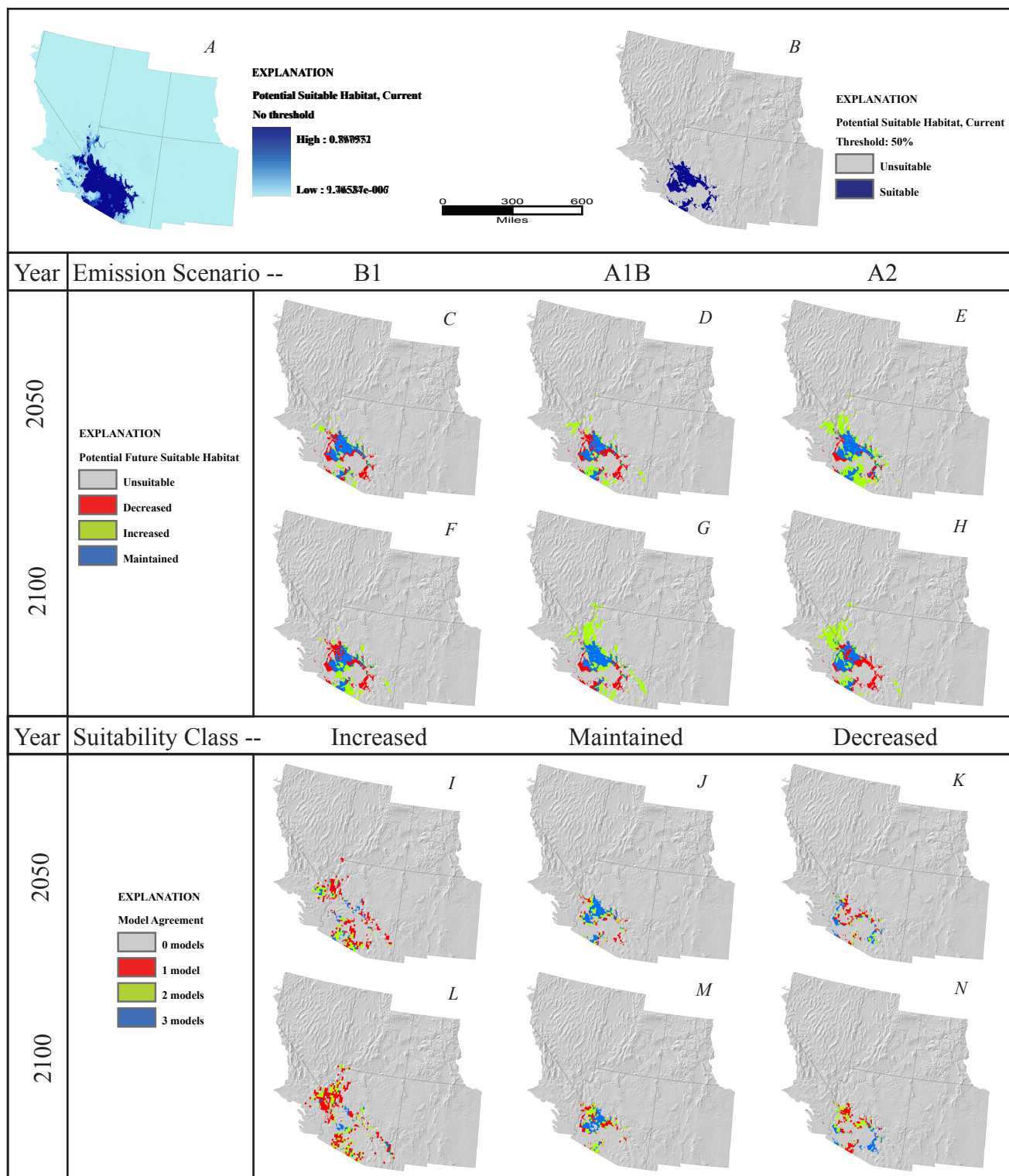
Figure 16. Parkinsonia microphylla . A, Potential suitable habitat for species based on average annual and monthly precipitation and temperature from 1971 to 2000, continuous model output with no threshold. B, Potential suitable habitat, binary output using .5 threshold. C-E, Potential suitable habitat predicted by year 2050 under emission scenario (C), B1, (D), A1B, (E), A2. F-H, Potential suitable habitat predicted by year 2100 under emission scenario (F), B1, (G), A1B, (H), A2. I-K, Number of 2050 emission scenario models predicting each suitability class, (I), increased suitability, (J), maintained suitability, (K), decreased suitability. L-N, Number of 2100 emission scenario models predicting each suitability class, (L), increased suitability, (M), maintained suitability, and (N), decreased suitability.
