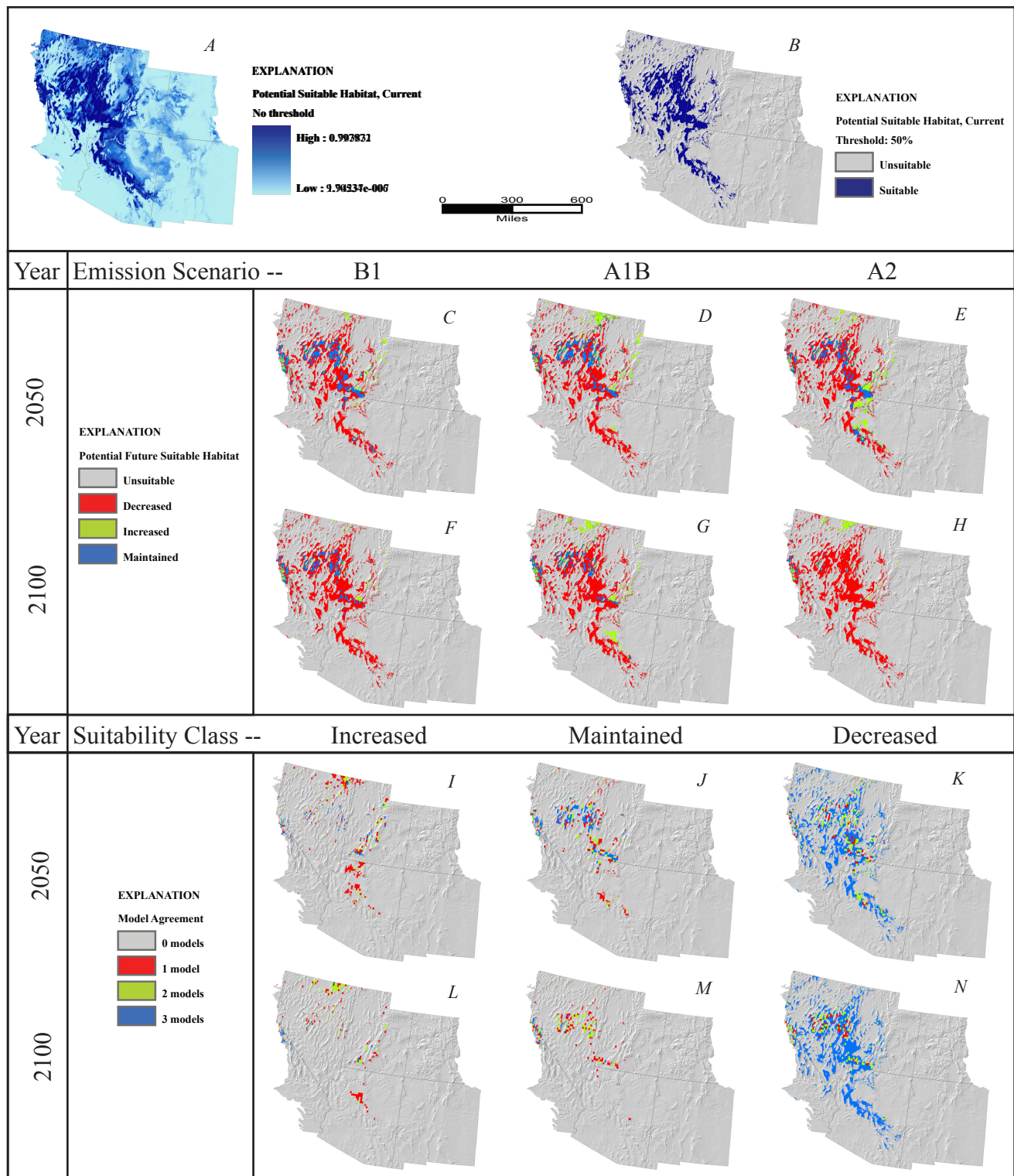
Figure 23. Pinus monophylla . A, Potential suitable habitat for species based on average annual and monthly precipitation and temperature from 1971 to 2000, continuous model output with no threshold. B, Potential suitable habitat, binary output using .5 threshold. C-E, Potential suitable habitat predicted by year 2050 under emission scenario (C), B1, (D), A1B, (E), A2. F-H, Potential suitable habitat predicted by year 2100 under emission scenario (F), B1, (G), A1B, (H), A2. I-K, Number of 2050 emission scenario models predicting each suitability class, (I), increased suitability, (J), maintained suitability, (K), decreased suitability. L-N, Number of 2100 emission scenario models predicting each suitability class, (L), increased suitability, (M), maintained suitability, and (N), decreased suitability.
